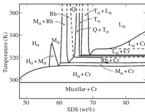
FIG. 3.9. Phase diagram of a mixture of sodium dodecylsulfate (SDS) and water [16]. Labels refer to one-dimensional lamellar ( L_\alpha ), two-dimensional hexagonal ( H_\alpha ), and monoclinic ( M_\alpha ), three-dimensional tetragonal ( T_\alpha ), cubic (Q) and rhombohedral (Rh) phases; Cr represents the SDS crystalline hydrates.
