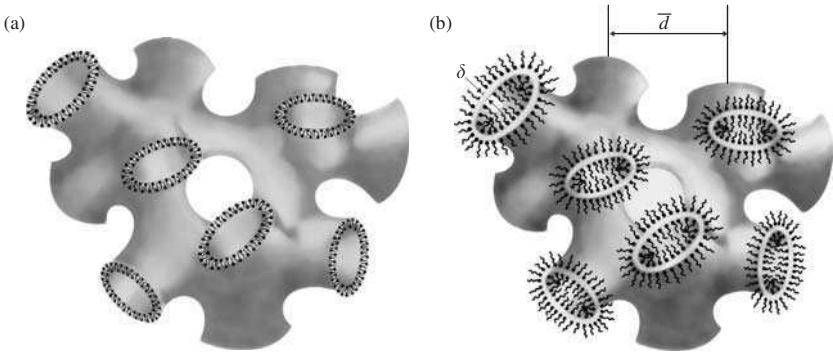
FIG. 5.4. Sketch of the sponge phase structure. Parameters \delta and \bar{d} represent the thickness of amphiphilic bilayer (water layer, for an inverted phase) and the mean distance between channels: (a) direct structure; (b) inverted structure.
