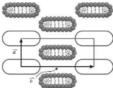
FIG. 7.13. Sketch of a cross section of the direct rectangular R_\alpha phase structure; the amphiphilic aggregates have a ribbon-type shape.
