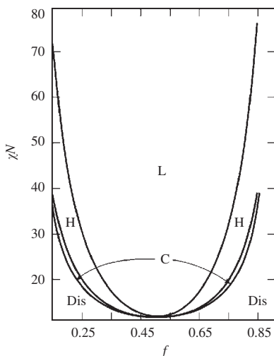
FIG. 8.10. Sketch of the phase diagram of an A–B type of DiCo in the plane \chi N versus f . Labels Dis, C, H and L refer to the disordered, cubic, hexagonal, and lamellar phases, respectively [138].
