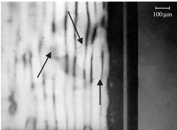
FIG. 8.5. Typical texture of an initially oriented ferrocholesteric \text{Ch}_C lyomesophase (unwinded by the magnetic field). The system has been allowed to relax after removing the magnetic field. The texture has been obtained in a polarizing light microscope, between crossed polarizers. Note the presence of large ferrofluid needles (see the indications of the arrows) decorating the hydrodynamic instabilities.
