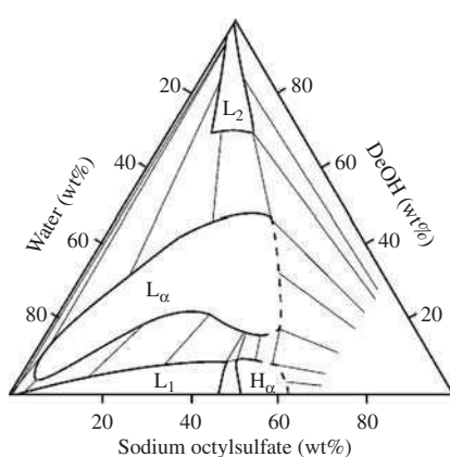
FIG. 3.10. Partial isothermal representation, at 20^\circ\text{C} , of a ternary mixture of Na octylsulfate, 1-decanol, and water [22].
