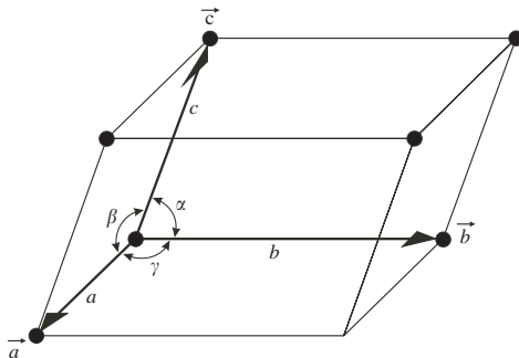
FIG. 7.11. Sketch of a unit cell.
