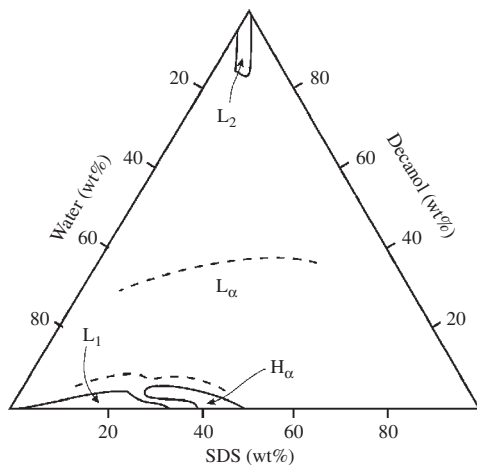
FIG. 7.1. Sketch of a partial isotherm, at 25^\circ\text{C} , for a mixture of sodium dodecylsulfate (SDS), decanol, and water [3].
