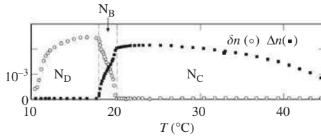
FIG. 6.1. Optical birefringences, \Delta n and \delta n , as a function of temperature, obtained from laser conoscopy measurements for a KL/DeOH/D mixture, with weight percentage composition 26/6.24/67.76 [4].
