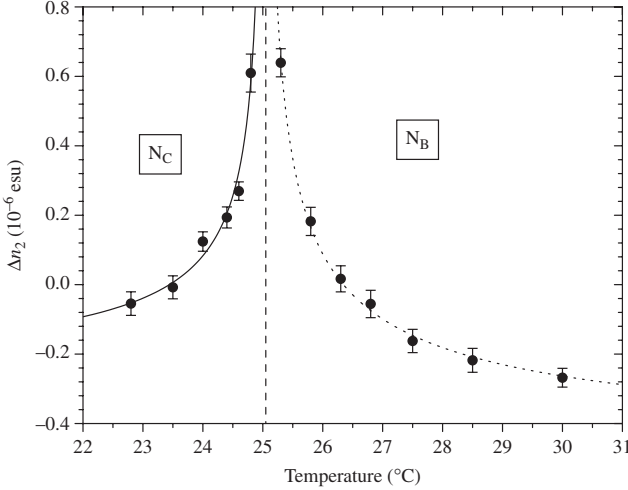
FIG. 6.4. Nonlinear birefringence, \Delta n_2 = n_{2\parallel} - n_{2\perp} , for a sample of potassium laurate, decanol, and water [21]. The subscripts \parallel and \perp refer to the configurations of the electric field \vec{E} of the probe laser beam with respect to the magnetic field \vec{B} used to orient the nematic N_C phase. The refraction index can be written as n = n_L + n_2 I_0 , where n_L is the linear index of refraction, I_0 is the intensity of the incident light, and n_2 is the nonlinear index of refraction. The dashed line corresponds to T_{c1} = 25.02^\circ\text{C} . The solid and dotted lines correspond to the fitting function \Delta n_2 \propto |T - T_{c1}|^{-\beta} , with \beta_C = 0.55(3) and \beta_B = 0.50(1) for the N_C and N_B phases, respectively.
