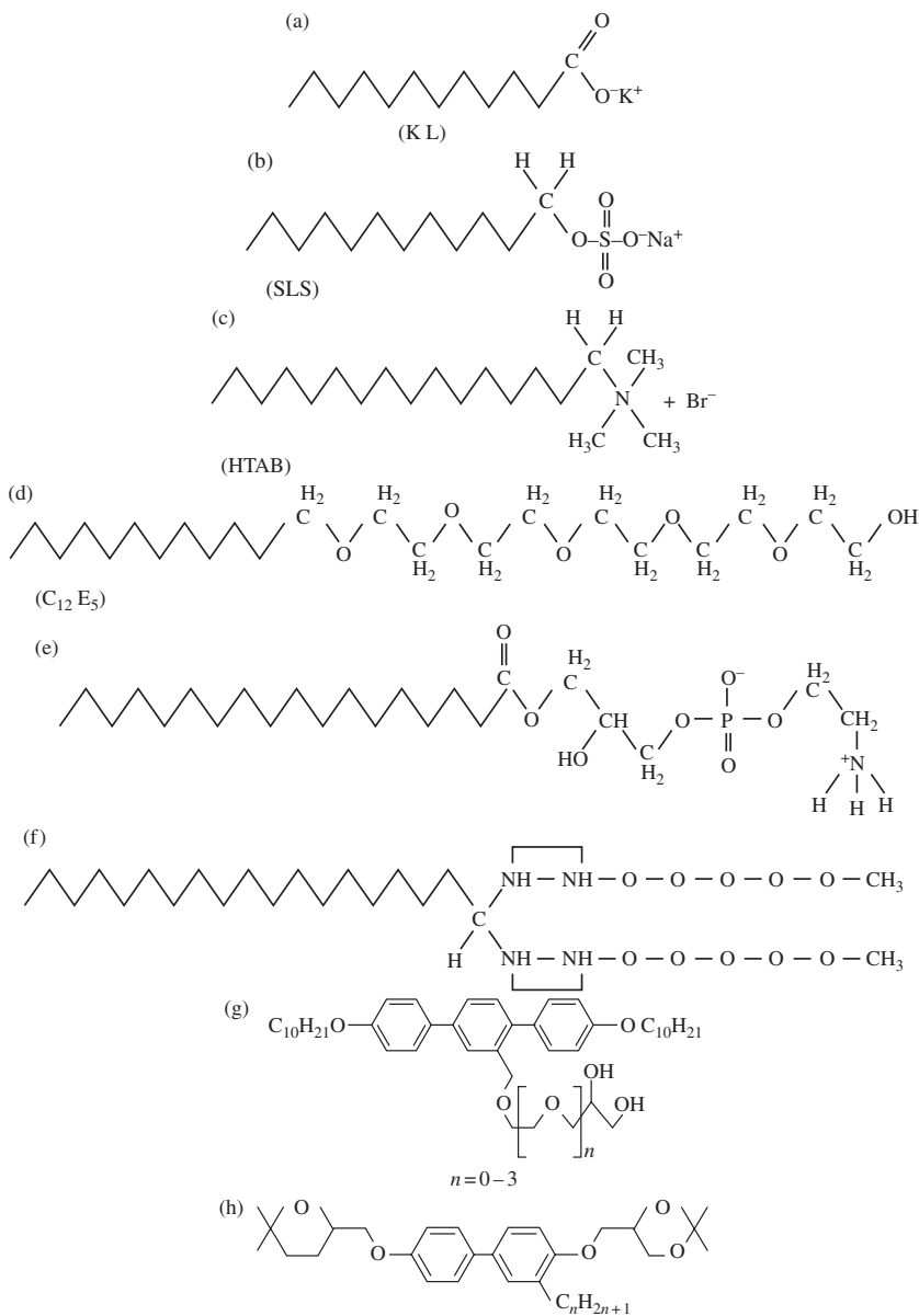
FIG. 1.2. Examples of different amphiphiles: (a) anionic, KL-potassium laurate; (b) detergent, SLS-sodium laurylsulfate; (c) cationic, HTAB or CTAB-hexadecyl trimethylammonium bromide; (d) nonionic, pentaerythylene dodecyl ether; (e) zwitterionic; (f) anelydes; (g) facial amphiphile; (h) bolaamphiphile.
