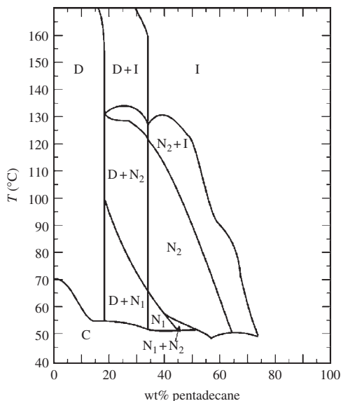
FIG. 8.13. Sketch of the phase diagram of a mixture of tetranuclear palladium organyl (see Fig. 8.12) and pentadecane [157]. We indicate the following structures: crystalline (C), nematic ( N_1 and N_2 ), discotic columnar (D), and isotropic (I).
