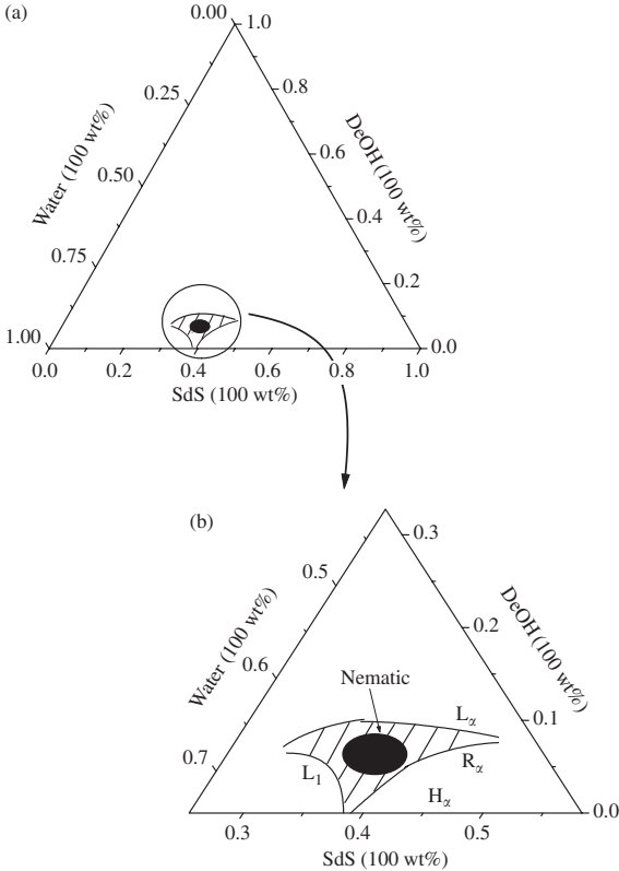
FIG. 3.11. Sketch of the partial isothermal representation, at 23°C, of the SdS/DeOH/water mixture [24]: (a) localization of the nematic domain; (b) zoom of the nematic domain and its neighboring phases (micellar isotropic, L_1 , hexagonal, H_\alpha , rectangular, R_\alpha , and lamellar, L_\alpha ).
