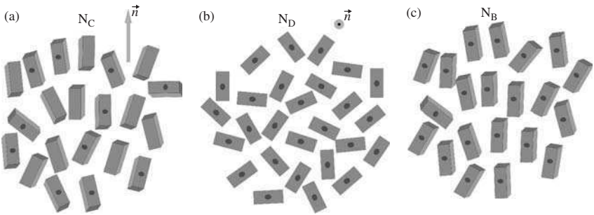
FIG. 1.11. Sketch of the micellar order in the context of the intrinsically biaxial (brick-like) micelles model. The dots represent a particular surface of the micelles and \vec{n} is the director: (a) N_C phase; (b) N_D phase; (c) N_B phase.
