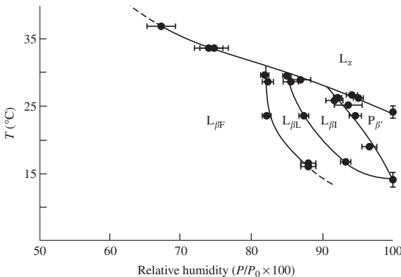
FIG. 1.34. Phase diagram of the mixture DMPC/water as a function of temperature and relative humidity (ref. [72]). P and P_0 are partial water-vapor pressure over the film, and vapor pressure of pure water over pure water, respectively.
