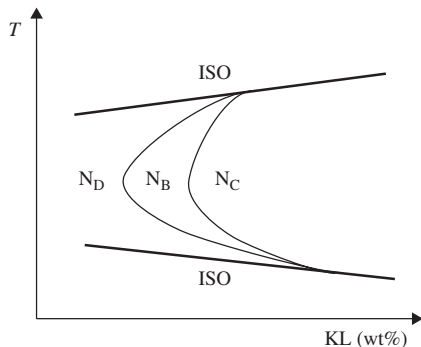
FIG. 2.13. Sketch of the typical temperature versus concentration (in this case, the potassium laurate KL amphiphile, at fixed concentration of decanol) experimental phase diagram of a ternary lyotropic mixture (KL, decanol, water). Note the reentrance of the disordered region at low temperatures.
