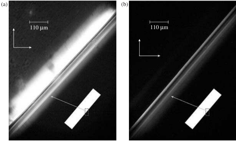
FIG. 1.24. Typical textures of N_D and L_1 phases in a polarizing light microscope, between crossed polarizers. Samples are placed in rectangular glass microslides sample-holders. The white arrows represent the directions of the polarizer and analyzer. (a) Pseudo-isotropic texture of a N_D phase in a homeotropic orientation of the director (see the bright borders of the sample holder). In the detail, in the right down corner of the figure, the microslide is sketched and the rectangle shows the corresponding region in the picture. (b) Micellar isotropic phase ( L_1 ) in the same conditions of (a).
