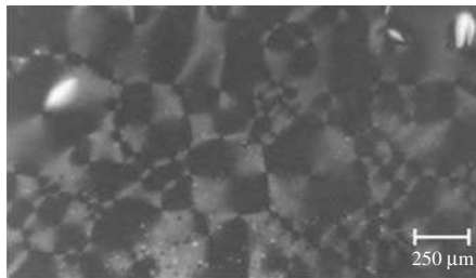
FIG. 1.33. Typical mosaic-like texture of a lamellar phase for a 100 \mu\text{m} thick sample of a potassium laurate/water mixture in a polarizing light microscope, between crossed polarizers.
