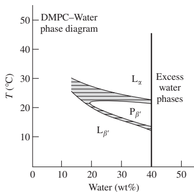
FIG. 1.32. Phase diagram of the mixture DMPC/water (ref. [133]).
