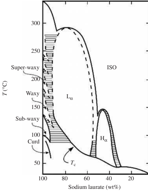
FIG. 3.18. Temperature versus concentration phase diagram of a mixture of sodium laurate and water [40].
