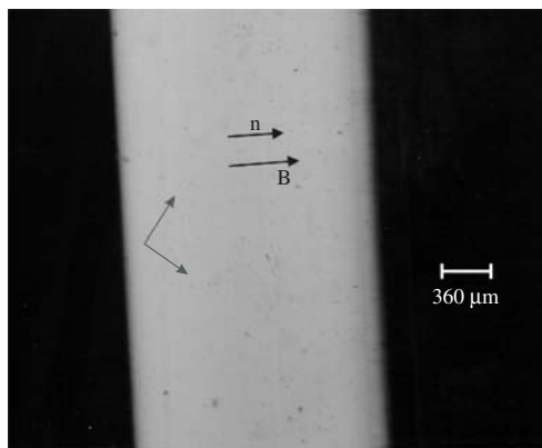
FIG. 1.21. Typical texture of a N_C phase in a polarizing light microscope, between crossed polarizer, about 1 h after the application of a magnetic field \mathbf{B} , in a sample 100 \mu\text{m} thick. The arrows represent the directions of the polarizer and analyzer.
