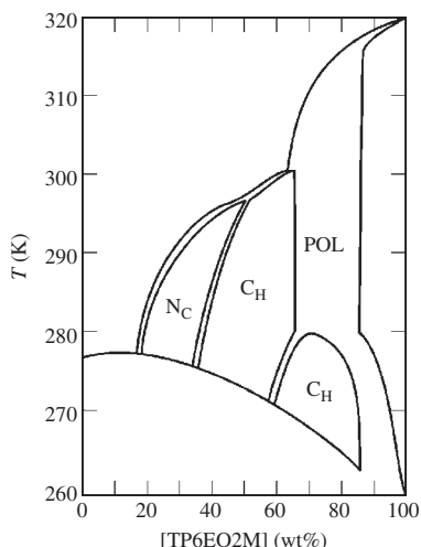
FIG. 6.6. Sketch of the phase diagram of a mixture of 2,3,6,7,10,11-hexa-(1,4,7-trioxaoctyl)-triphenylene and water [27].
