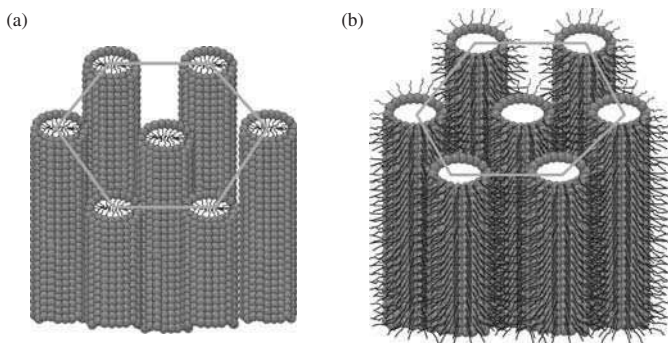
FIG. 1.15. Sketch of the hexagonal phase structure: (a) direct; (b) inverted.
