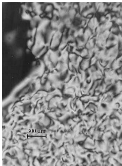
FIG. 1.25. Typical texture of coexisting nematic and micellar isotropic phases (for a 200 \mu\text{m} thick sample of a potassium laurate/1-decanol/water mixture) in a polarizing light microscope, between crossed polarizers. The isotropic phase domain is located at the upper left side of the figure.
