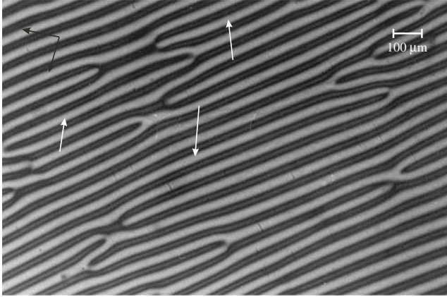
FIG. 1.29. Typical texture of an oriented cholesteric Ch_B lyomesophase (for a 200\ \mu\text{m} thick sample of sodium decylsulfate/1-decanol/water/brucine sulfate heptahydrate mixture) in a polarizing light microscope, between crossed polarizers. Black arrows represent the directions of the polarizer and analyzer. White arrows show some planar regions in the center of fingerprint stripes.
