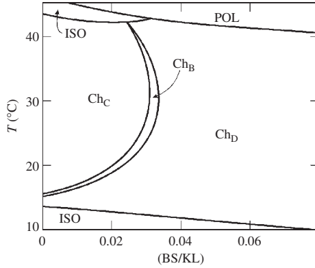
FIG. 6.13. Sketch of the surface of the phase diagram of the lyotropic cholesteric mixture KL/DeOH/D/BS [53]. Labels POL and ISO refer to polyphase and isotropic regions, respectively. The horizontal axis represents the relative weight percentage of BS with respect to KL.
