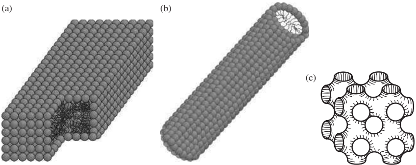
FIG. 1.3. Amphiphilic molecular aggregates. The polar head and the paraffinic chain of the molecules are represented by a sphere and a line, respectively: (a) sketch of an orthorhombic micelle. The cut in the right-down side shows the paraffinic chains in its inner part; (b) large anisotropic cylindrical aggregate; (c) sketch of a bicontinuous molecular aggregate with a cubic symmetry.
