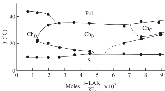
FIG. 1.27. Surface of the phase diagram of the lyotropic cholesteric mixture of potassium laurate (KL)/1-decanol/water/ l - N -lauroyl potassium alaninate ( l -LAK) [124]; POL and S refer to the polyphasic and gel regions, respectively.
