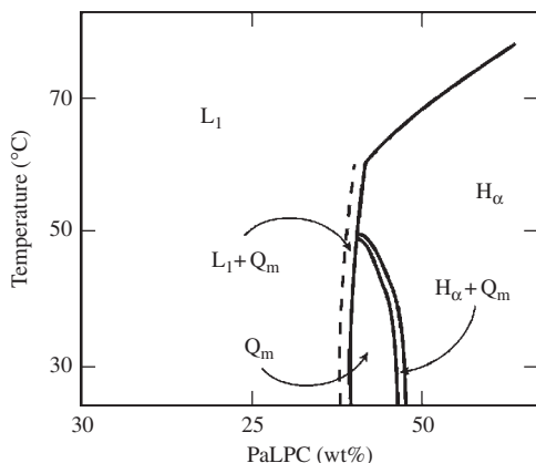
FIG. 7.19. Phase diagram of a mixture of 1-palmitoyllysophosphatidylcholine (PaLPC) and water [74]. The micellar cubic Q_m phase is located between H_\alpha and L_1 phases.
