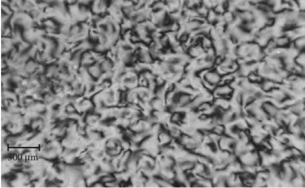
FIG. 1.20. Typical schlieren texture of a N_C phase (with a sample of thickness 200\ \mu\text{m} of a potassium laurate/1-decanol/water mixture) in a polarizing light microscope, between crossed polarizer. The line in this figure corresponds to 300\ \mu\text{m} .
