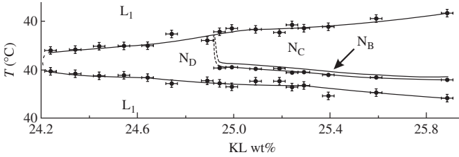
FIG. 1.9. Surface of the phase diagram of a mixture of potassium laurate, decanol (at 6.24 wt%) and water; L_1 , N_C , N_B , and N_D represent the micellar isotropic, calamitic nematic, biaxial nematic, and discotic nematic phases, respectively (from ref. [82]).
