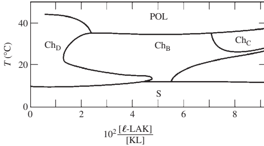
FIG. 6.14. Sketch of a surface of the phase diagram of the KL/DeOH/W/L-N-lauroyl potassium alaninate mixture [60]. The horizontal axis represents the relative molar ratio of L-N-lauroyl potassium alaninate with respect to KL.
