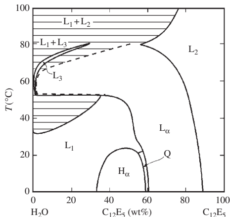
FIG. 3.8. Phase diagram of the binary C_{12}E_5 /water mixture [13]. Labels refer to lamellar ( L_{\alpha} ), direct and inverted micellar ( L_1 and L_2 ), sponge ( L_3 ), hexagonal ( H_{\alpha} ), and cubic ( Q ) phases.
