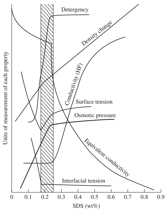
FIG. 5.2. Sketch of the behavior of some physico-chemical properties of the SDS/water mixture around CMC [3]. The hatched region corresponds to the range of CMC.
