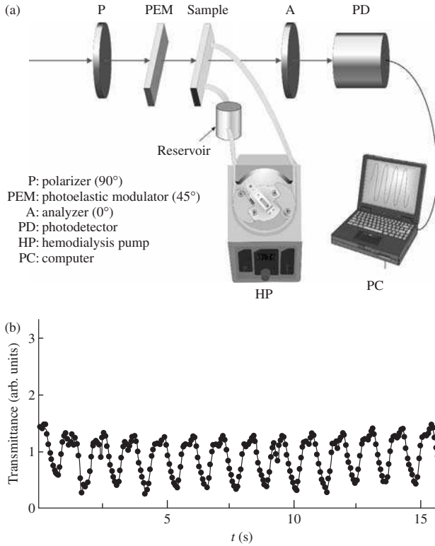
FIG. 1.37. (a) Sketch of the monitoring device for hemodialysis blood pumps using a lyotropic sponge mesophase. The angles in the figure are measured with respect to the vertical direction. (b) Optical transmittance as a function of time in the hemodialysis blood pump device.
