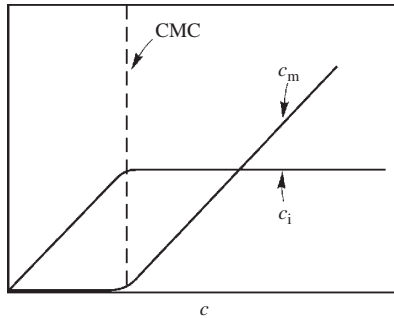
FIG. 1.4. Concentration of isolated amphiphilic molecules ( c_i ) and micelles ( c_m ) around CMC as a function of the concentration amphiphilic molecules ( c ) [14].
