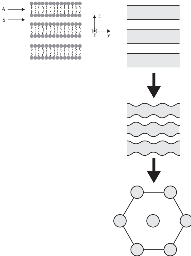
FIG. 4.6. Two dimensional sketch of the transition from the lamellar, L, to the hexagonal, H, phase, generated by undulations of the lamellae on the x - y plane.
