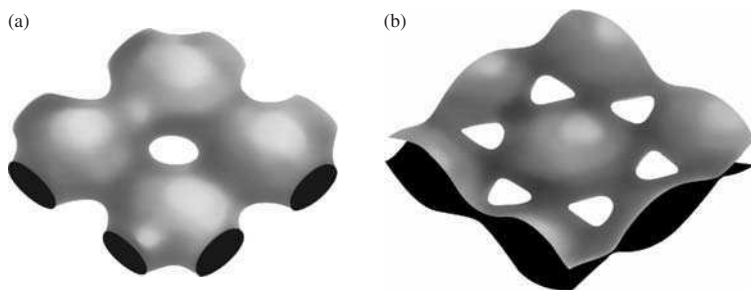
FIG. 1.36. Lower symmetry lyotropic phase structures: (a) sketch of one layer of the centered tetragonal mesh structure [190]; (b) sketch of one layer of the rhombohedral mesh structure [189].
