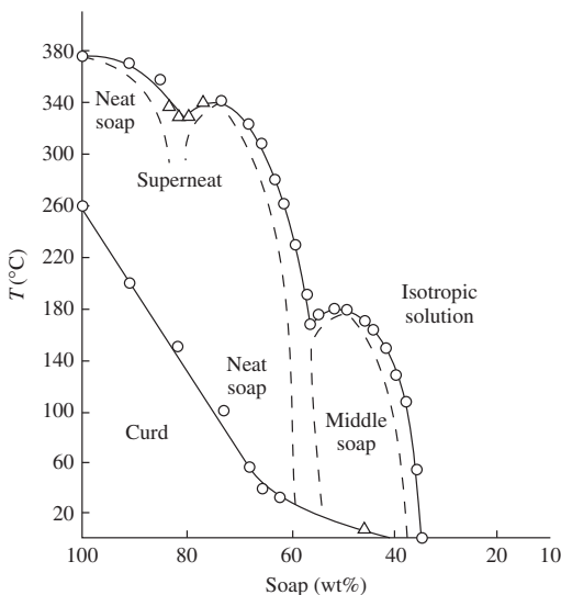
FIG. 1.6. Phase diagram of the potassium laurate/water mixture, in the temperature versus concentration plane (ref. [32]). The phases shown in the figure are discussed in the following sections.
