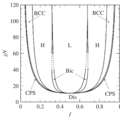
FIG. 8.11. Sketch of a mean-field calculation for the phase diagram of a DiCo in terms of \chi N and f (see Matsen and Bates [153]). We indicate the following structures: L (lamellar), H (hexagonal cylinders), Bic (bicontinuous cubic), BCC (bcc spheres), CPS (close-packed spheres), and Dis (disordered).
