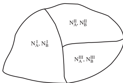
FIG. 3.1. Composite system with three subsystems (I, II, and III) of two components (A and B) each. The system is in equilibrium at fixed values of temperature and pressure. The walls between subsystems are diathermal, moveable, and permeable to all components. The outer border is impermeable.
