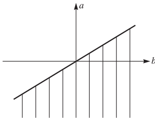
FIG. 2.14. Phase diagram, in terms of the Landau parameters a and b , of a compressible ferromagnetic model. The second-order line is given by a = b/2 (the hatched region corresponds to the ferromagnetically ordered phase).
