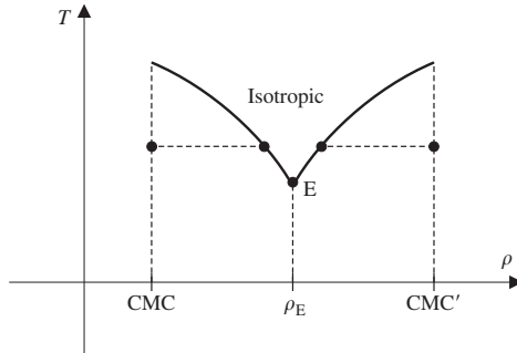
FIG. 3.17. Section of the phase diagram, in terms of temperature versus density, for a binary system with a eutectic point (E).
