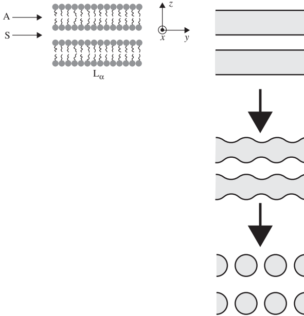
FIG. 4.1. Sketch of the lamellar-tetragonal phase transition generated by undulations of the lamellae in the x - y plane.
