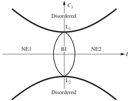
FIG. 2.15. Section of the phase diagram, in terms of the coefficients C_1 and B , with two uniaxial and a biaxial nematic phase. The heavy solid lines correspond to first-order boundaries. The biaxial–uniaxial transition remains second order. Note the re-entrance of the isotropic phase and the occurrence of two Landau points ( L_1 and L_2 ).
