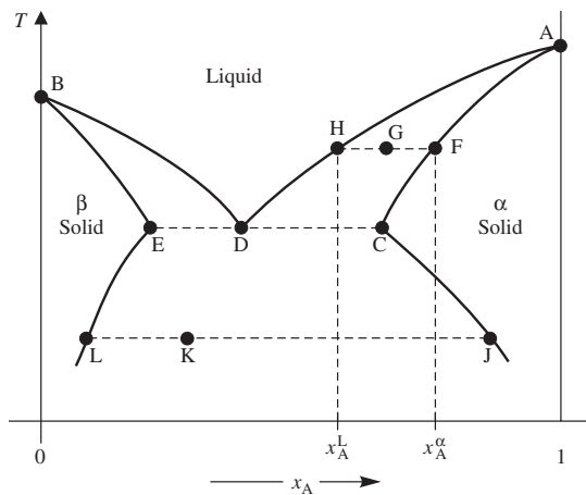
FIG. 3.4. Constant pressure section of a typical temperature versus concentration phase diagram of a binary system.
