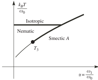
FIG. 2.12. Phase diagram of the McMillan model, with isotropic, uniaxial nematic and smectic A phases. The heavy solid lines are first-order boundaries. There is also a second-order line that ends at the tricritical point T_3 .
