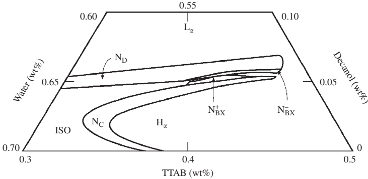
FIG. 6.11. Sketch of the surface of the phase diagram of a mixture of TTAB (tetradecyltrimethylammonium bromide), n -decanol and water (at 10 wt% of D 2 O), at room temperature (22°C) [44].
