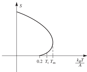
FIG. 2.8. Graph of the Maier-Saupe order parameter S versus temperature (in suitable dimensionless units). We indicate the temperature T_m = 0.22284\dots below which there is a solution S \neq 0 . From thermodynamic considerations, the first-order phase transition in this mean-field model occurs at T_t = 0.22019\dots , which is very close to T_m .
