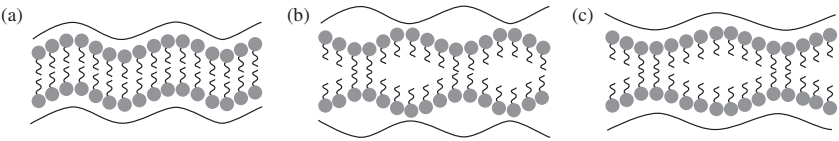
FIG. 7.8. Sketch of the low-frequency hydrodynamic modes of a lamellar structure [9,36]: (a) transverse shear mode; (b) peristaltic mode; (c) undulation–baroclinic mode.
