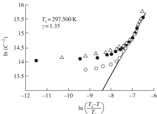
FIG. 1.31. Double logarithmic plot of the inverse of the cholesteric susceptibility, C^{-1} \propto \zeta^{-1} q^2 , versus reduced temperature, (T_c - T)/T_c [119]. The symbols \Delta , \bullet , and \circ represent different concentrations of chiral molecules, from the smallest ( \circ ) to the largest ( \Delta ). The chiral doping represents the elastic field. The line is a linear fitting.
