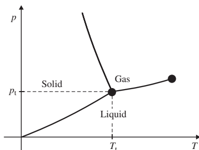
FIG. 3.2. Sketch of a T - p phase diagram of a one-component system. Solid lines indicate first-order transitions (coexistence of phases). At the triple point, T_t , p_t , there is coexistence among solid, liquid, and gas phases.
