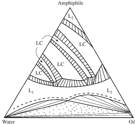
FIG. 5.1. Sketch of the partial isothermal representation of a mixture of an amphiphile, water, and oil [2]. The symbol LC represents liquid crystalline phases; the lateral sides of the triangle represent the amphiphile concentration.
