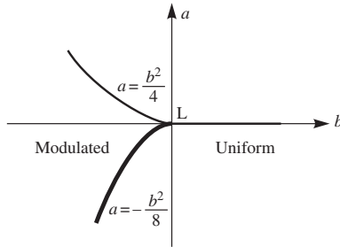
FIG. 2.7. Phase diagram with disordered, modulated, and uniform phases.
