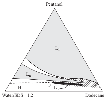
FIG. 3.13. Sketch of a particular partial isotherm, at room temperature and [\text{water wt}\%] / [\text{SDS wt}\%] = 1.2 , of a mixture of SDS, dodecane, pentanol, and water [35].
