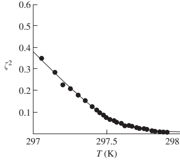
FIG. 1.30. Square of the induced biaxial order parameter ( \zeta ) as a function of temperature in the neighborhood of the \text{Ch}_D - \text{Ch}_B phase transition, for a potassium laurate/decylammonium chloride/water/brucine sulfate heptahydrated mixture [119]. The line is a fitting from the minimization of the characteristic free-energy density.
