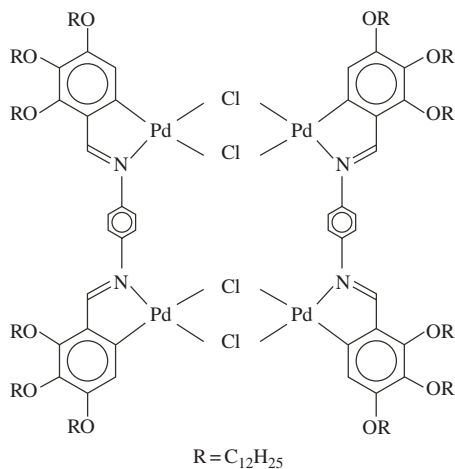
FIG. 8.12. Molecular structure of tetranuclear palladium organyl.
