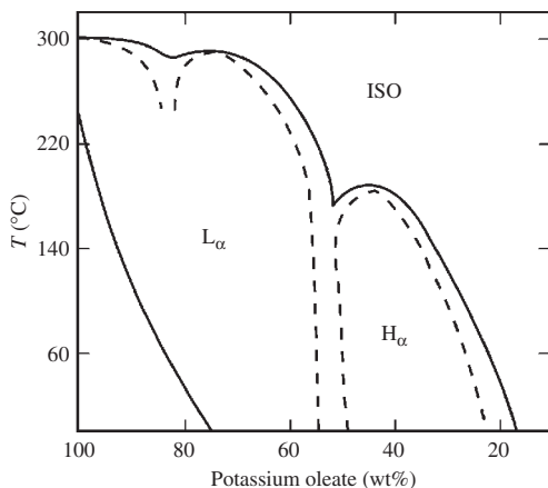
FIG. 7.2. Sketch of the temperature versus concentration phase diagram of a mixture of potassium oleate and water [14]. The label ISO refers to an isotropic phase.
