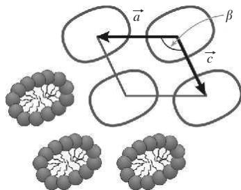
FIG. 7.12. Sketch of a cross section of the monoclinic M_\alpha phase structure; the amphiphilic aggregates have a ribbon-type shape.
