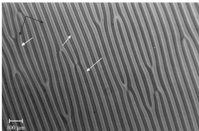
FIG. 1.28. Typical texture of an oriented cholesteric \text{Ch}_D lyomesophase (for a 200\ \mu\text{m} thick sample of a sodium decylsulfate/1-decanol/water/brucine sulfate heptahydrate mixture) in a polarizing light microscope, between crossed polarizers. Black arrows represent the directions of the polarizer and analyzer. White arrows show some homeotropic regions in the center of fingerprint stripes.
