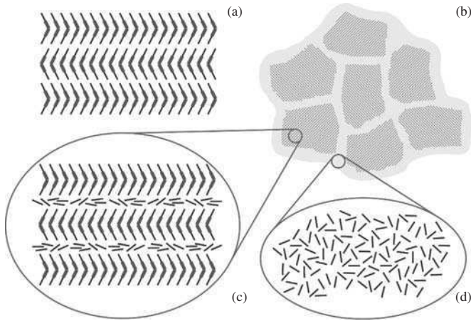
FIG. 8.15. Model for the molecular packing of the pure banana-shaped C14 liquid crystal and a mixture containing n -hexadecane [168]: (a) antiferroelectric molecular packing of pure C14 ; (b) submicrometer segregated isotropic HEX domains surrounding the smectic domains of C14 with layered nanosegregated HEX molecules; (c) magnified local structure of smectic domains with nanosegregated HEX molecules; (d) magnified local structure of submicrometer segregated HEX molecules.
