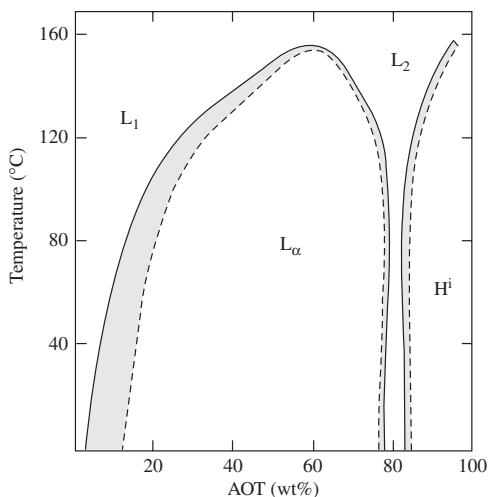
FIG. 7.3. Sketch of the phase diagram of a mixture of sodium bis-2-ethylhexyl sulfosuccinate (AOT) and water [18]. The gray regions correspond to phase coexistence.
