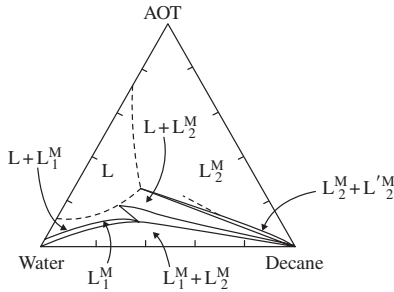
FIG. 8.6. Partial isothermal representation, at T = 25^\circ\text{C} , of the phase diagram of the mixture AOT/water/decane [92].
