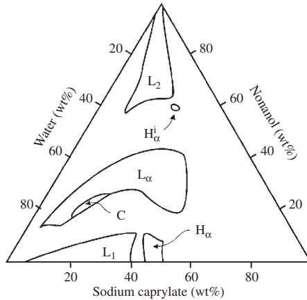
FIG. 4.4. Partial isothermal section, at 20°C, of the phase diagram of a mixture of sodium caprylate, nonanol, and water [14].
