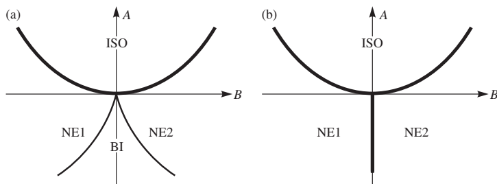
FIG. 2.11. Phase diagrams in terms of the Landau parameters A and B . The heavy solid lines are first-order boundaries. In (a), for E' > 0 , there is a biaxial (BI) and two uniaxial nematic phases (NE1 and NE2). In (b), for E' = 0 , there is no nematic biaxial phase.
