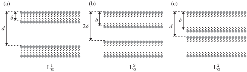
FIG. 7.6. Sketch of the lamellar structure under dilution with a non-polar solvent (polar solvent is placed between lamellae and non-polar solvent is placed inside lamellae): (a) usual lamellar structure ( L_{\alpha}^1 ); (b) symmetric case ( L_{\alpha}^S ); polar and non-polar layers have the same thickness; (c) inverted lamellar structure ( L_{\alpha}^2 ).
