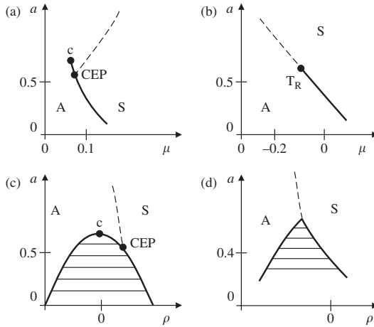
FIG. 5.5. Sketch of some phase diagrams associated with the Landau expansion for the free energy of lyotropic mixtures with a sponge phase: (a) and (c) correspond to A = -0.2 ; (b) and (d) correspond to A = 0.2 . We indicate the symmetric (S) and ordered (A) sponge phases. In (a) and (b), heavy solid lines represent first-order transitions; continuous transitions are represented by dashed lines. C, T_R , and CEP, label critical, tricritical, and critical end points, respectively. In (c) and (d), we draw the corresponding phase diagrams in terms of field and density variables, and indicate some tie lines of phase coexistence.
