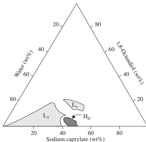
FIG. 7.5. Sketch of a partial isotherm of a mixture of sodium caprylate, 1,8-octandiol, and water, at 20°C [3].
