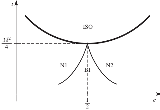
FIG. 2.10. Typical phase diagram for a mixture of prolate and oblate molecular aggregates. The heavy solid line represents a first-order transition (between an isotropic phase, ISO, and the uniaxial-nematic phases, N_1 and N_2 ). There are second-order transitions between the uniaxial nematic phases and the biaxial phase (BI).
