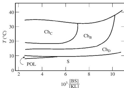
FIG. 6.12. Sketch of the surface of the phase diagram of the lyotropic cholesteric mixture of KL/DeOH/D/BS [48]. Labels POL and S refer to polyphase and gel regions, respectively. The horizontal axis represents the relative molar ratio of BS with respect to KL.
