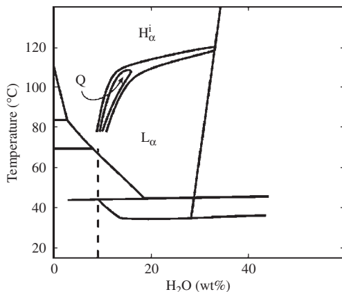
FIG. 7.20. Phase diagram of the lyotropic mixture of (di - C 12 ) dialkyl didodecylphosphatidylethanolamine (DDPE) and water [92]. The bicontinuous cubic Q phase is located between H i and L α phases.
