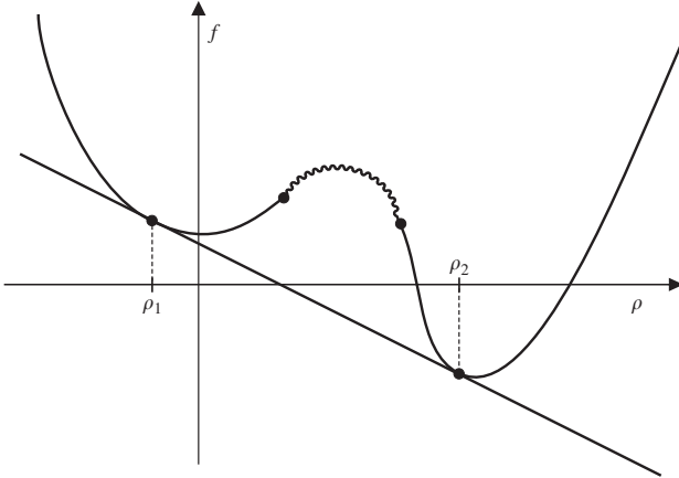
FIG. 3.15. Graph of the Helmholtz free energy per mole f versus the density \rho for sufficiently low temperatures. Note that convexity is recovered by the double-tangent construction. The curly line indicates the unstable solutions.
