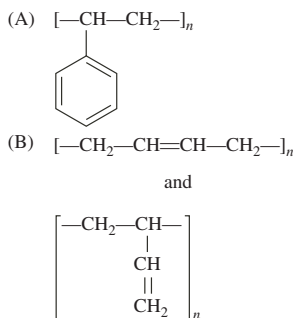
FIG. 8.9. Basic units of the diblock copolymer polystyrene (A) and polybutadiene (B).
