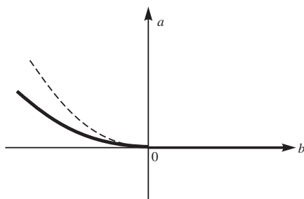
FIG. 2.3. Phase diagram in terms of the Landau coefficients a and b . The first-order boundary (heavy solid line; given by a = 3b^2/16 with b < 0 ) meets the critical line (given by a = 0 with b > 0 ), with zero slope, at a tricritical point ( a = b = 0 ). The dashed line is the stability limit of the ordered solution.
