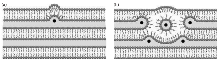
FIG. 7.9. Sketch of a possible mechanism for the lamellar–inverse hexagonal phase transition [44]. Black dots represent the water cores: (a) beginning of the process with the creation of a line defect; (b) formation of the first cylinder, with an axis perpendicular to the plane of the figure.
