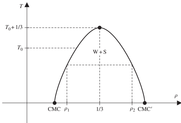
FIG. 3.16. Phase diagram, in terms of density \rho and temperature T , for the simple solvent-surfactant model; CMC and CMC' indicate critical micellar concentrations for direct and inverted micelles.
