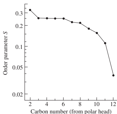
FIG. 1.7. Order parameter of the different CD (carbon-deuteron) bonds in the paraffinic chain inside a micelle (from DMR measurements of quadrupolar splittings [38]).
