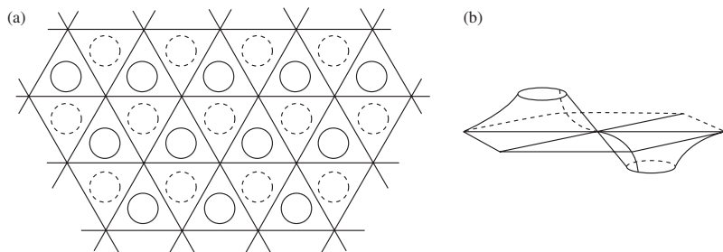
FIG. 7.16. Sketch of the diamond-type surface (D-surface) [89]: (a) lattice formed by two-fold axes; filled and open circles indicate the catenoids going upwards and downwards; (b) illustration of two of these catenoids.
