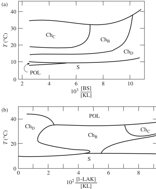
FIG. 3.14. Sketch of particular surfaces of phase diagrams of quaternary mixtures of cholesteric systems: (a) KL/DeOH/water/BS; the number of moles of KL, water and DeOH are fixed; POL is a polyphase and S is a gel region. The horizontal axis represents the relative molar ratio of BS with respect to KL [36]; (b) KL/DeOH/water/L-LAK; the number of moles of KL, water and DeOH is fixed [37]. The horizontal axis represents the relative molar ratio of L-N -lauroyl potassium alaninate with respect to KL.
