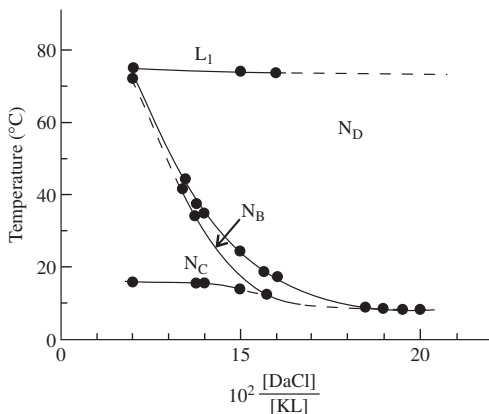
FIG. 1.19. Phase diagram of the potassium laurate/decylammonium chloride (DaCl)/water mixture (from ref. [90]).
