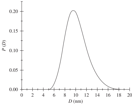
FIG. 8.3. Log-normal plot of size distribution of grains P(D) with \sigma = 0.2 and D_0 = 10 nm.
