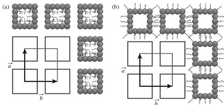
FIG. 7.14. Sketch of a cross section of the square phase structure; the amphiphilic aggregates have a square-type shape, a = b ; (a) direct, C; (b) inverted phase, K.
