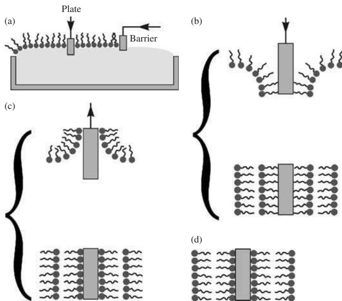
FIG. 8.8. Deposition of a Langmuir–Blodgett film: (a) deposition setup; (b) X-type deposition; (c) Z-type deposition; (d) Y-type deposition.
