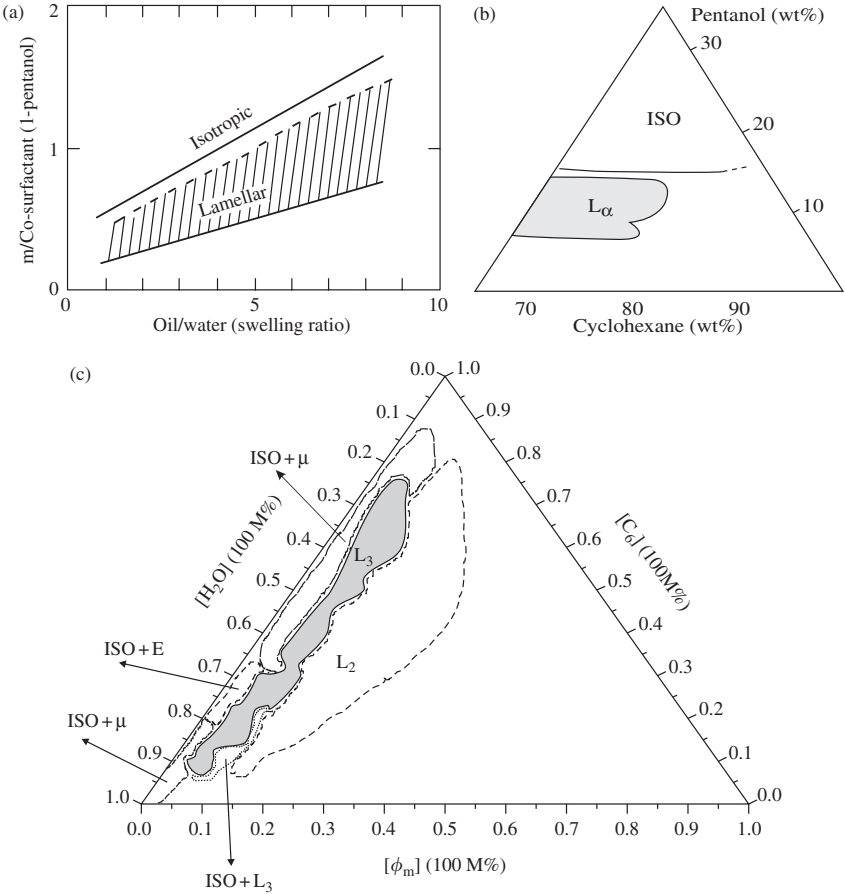
FIG. 3.12. Sketch of a particular surface of the phase diagram of a quaternary mixture of SDS, 1-pentanol (POH), cyclohexane and water: (a) at room temperature, the water volume is fixed, and the volume ratio of water/SDS is 2.5 [31]; (b) the volume ratio of water/SDS is fixed at 2.5 [32]. The sides of the triangle represent the pentanol concentration, which increases from the bottom towards the upper vertex; L_\alpha and ISO stand for the lamellar and isotropic phases, respectively; (c) representation at 21.5°C and molar ratio [\text{SDS}]/[\text{POH}] = 0.17 . The labels Iso, E, \mu , L_2 and L_3 refer to isotropic, emulsion, micro-emulsion, inverted micellar, and sponge phases, respectively; \phi_m = [\text{SDS} + \text{POH}] is the molar concentration of SDS and POH.
