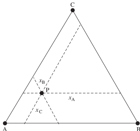
FIG. 3.5. Equilateral triangle for representing the relative molar concentrations of a ternary system (note that x_A + x_B + x_C = 1 ). The vertices correspond to pure phases.
