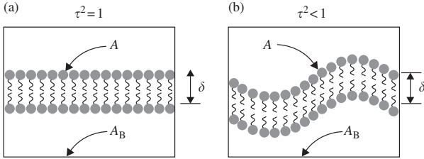
FIG. 7.7. Definition of the crumpling parameter \tau^2 = A_B/A , where A is the real area of the membrane and A_B is the projection of the area: (a) \tau^2 = 1 ; (b) \tau^2 < 1 .
