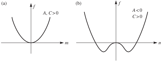
FIG. 2.1. Free-energy density f versus magnetization m for (a) A, C > 0 , and (b) A < 0 and C > 0 .
