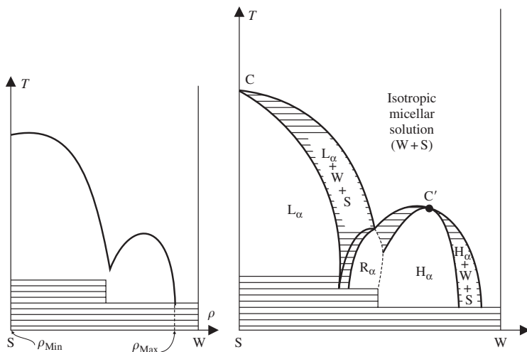
FIG. 3.19. Some theoretical predictions from a phenomenological approach to the description of the mixture of sodium laurate and water [41].
