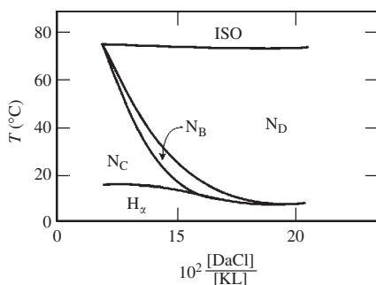
FIG. 6.10. Sketch of a surface of the phase diagram of the KL/DaCl/water mixture [32]. Labels ISO and H_\alpha refer to isotropic and hexagonal phases, respectively. The horizontal axis represents the relative molar ratio of DaCl with respect to KL. The molar ratio [\text{DaCl} + \text{KL}]/[\text{water}] = 5 \times 10^{-2} is kept fixed.
