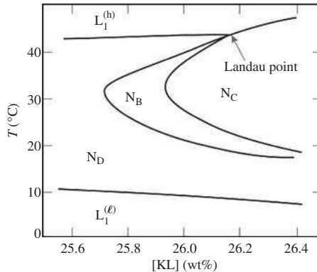
FIG. 6.2. Sketch of the surface of the phase diagram of the potassium laurate/1-decanol/D 2 O mixture [2]. Concentration of DeOH is fixed at 6.24 wt%.
