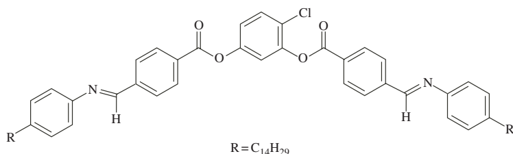
FIG. 8.14. A “banana”-shaped molecule: 4-chloro-1,3-phenylenebis [4-(4- N -tetradecyloxyphenyliminomethyl)benzoate].
