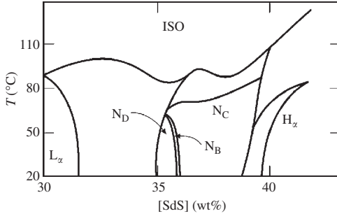
FIG. 6.9. Sketch of a surface of the phase diagram of the SdS/1-decanol/water mixture [31]. Labels ISO, L_\alpha , and H_\alpha refer to isotropic, lamellar, and hexagonal phases, respectively. The width of the N_B domain is restricted to about 0.1 wt% of the concentration of SdS. The water concentration is fixed at 57 wt%.
