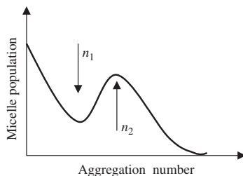
FIG. 5.3. Schematic representation of the micellar population as a function of the aggregation number, at fixed temperature and for c \gtrsim \text{CMC} .
