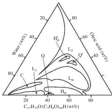
FIG. 4.3. Partial isothermal section, at 20°C, of the phase diagram of a mixture of decaoxyethylene glycol mono-lauryl ether, oleic acid, and water [14].
