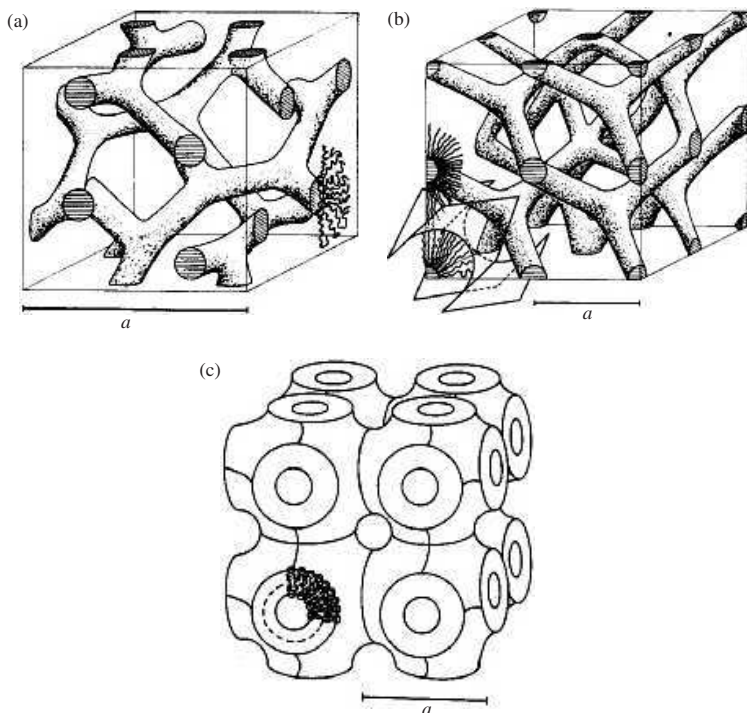
FIG. 7.18. Sketch of bicontinuous cubic structures with a lattice parameter a [91]: (a) Q^{230} , with space group Ia\bar{3}d ; (b) Q^{224} , with space group Pn\bar{3}m ; (c) Q^{229} , with space group Im\bar{3}m .
