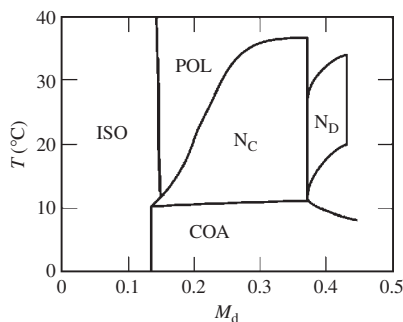
FIG. 6.7. Sketch of the phase diagram of the SLS/DeOH/W mixture [33]. Labels POL, ISO and COA refer to polyphasic, isotropic and coagel regions, respectively. In the horizontal axis, the parameter M_d represents the relative molar ratio of DeOH with respect to SLS.
