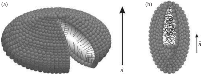
FIG. 1.10. Sketch of micelles in lyotropic mixtures with one amphiphile only; \vec{n} is the director, or axis of symmetry, of the phase. The cuts show the paraffinic chains in inner part of micelles: (a) oblate ellipsoid or disk-shaped; (b) prolate ellipsoid or cylinder-shaped.
