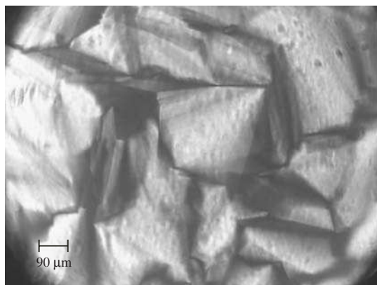
FIG. 1.39. Typical fan-like texture of a phase induced by radiation (protons of 40 Gy) in a sample of a previously nematic phase, in a polarizing light microscope, between crossed polarizers (for a 200 \mu\text{m} thick sample of a potassium laurate/decanol/water mixture).
