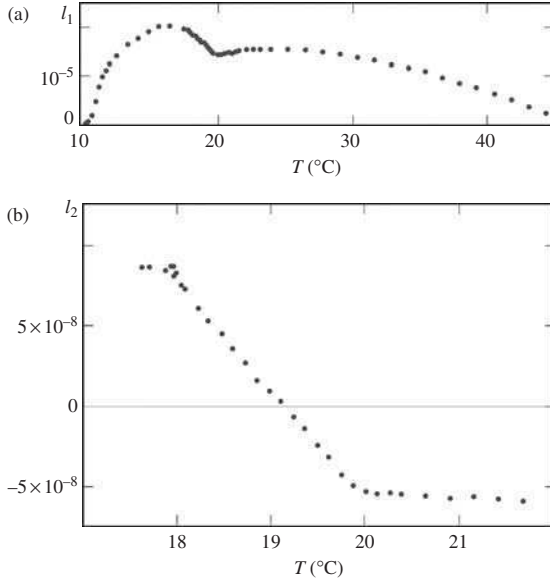
FIG. 6.3. Invariants of the symmetry-breaking order parameter (anisotropic part of the dielectric tensor) as a function of temperature, in the nematic region of the KL/DeOH/D mixture [4]: (a) I_1 invariant; (b) I_2 invariant.
