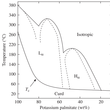
FIG. 3.7. Phase diagram of the potassium palmitate/water mixture, in terms of temperature versus concentration [3].
