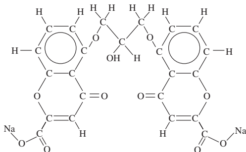
FIG. 1.8. Disodium chromoglycate (DSCG) molecule, which leads to a chromonic mixture.
