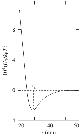
FIG. 8.4. Sketch of the total interaction potential U_T between magnetic grains in a ferrofluid as a function of the intergrain distance r , for \psi_0 = 15 mV, \text{pH}=2.5 , and D = 8.2 nm [13].
