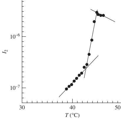
FIG. 1.26. Invariant I_2 of the dielectric tensor as a function of temperature, at the uniaxial–biaxial phase transition in a potassium laurate/decylammonium chloride (DaCl)/water mixture (from ref. [90]).
