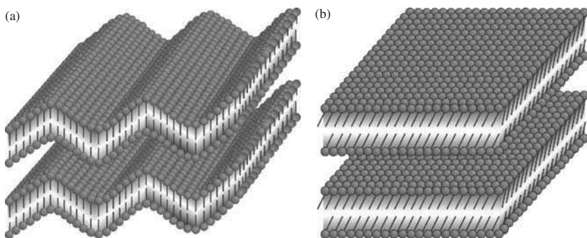
FIG. 1.14. Sketch of lamellar phase structures: (a) ripple phase P_{\beta'} ; (b) L_{\beta'} phase.
