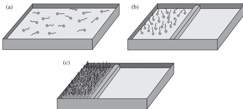
FIG. 8.7. Monolayer of surfactant molecules in a liquid–gas interface: (a) small concentration of surfactant molecules; (b) large concentration of non-compressed surfactant molecules; (c) large concentration of compressed surfactant molecules.
