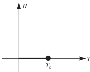
FIG. 2.2. Phase diagram, in terms of external field H and temperature T , of a simple uniaxial ferromagnet. The first-order boundary (solid line) ends at the critical temperature T_c .
