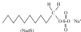
FIG. 1.1. Amphiphilic molecule of sodium decylsulfate.
