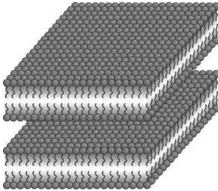
FIG. 1.13. Sketch of the lamellar L_\alpha structure.
