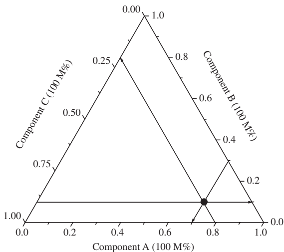
FIG. 3.6. Sketch of a triangular phase diagram (also known as partial isotherm) of a hypothetical mixture with three components. The axes are represented in molar percentages, M%.
