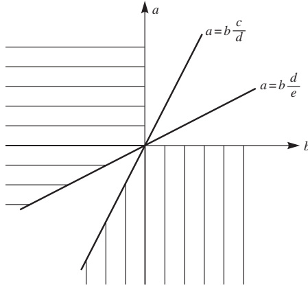
FIG. 2.5. Regions of stability of the Néel ordered phase [ a < 0 , and a < b(c/d) ; vertical hatches] and of the spin-flop phase [ b < 0 , and a > b(d/e) ; horizontal hatches].
