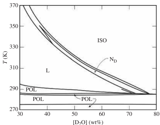
FIG. 6.5. Sketch of the phase diagram of a mixture of cesium perfluoro-octanoate and water [26].
