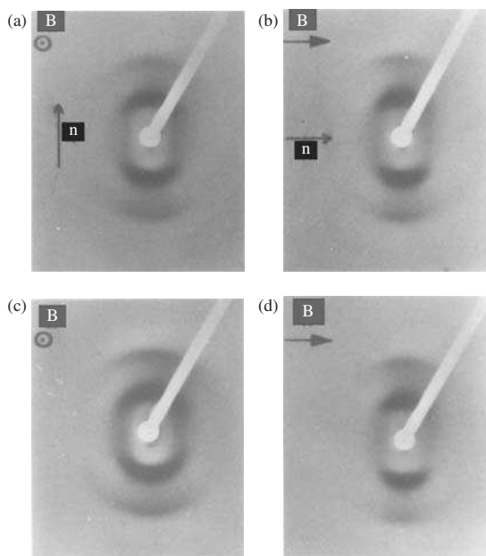
FIG. 1.22. Typical X-ray diffraction pattern of oriented sample (from ref. [61]): (a) N_D phase; (b) N_C phase; (c); and (d) N_B phase.
