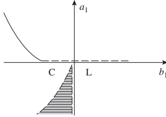
FIG. 4.2. Typical phase diagram [12] obtained from the minimization of Eq. (4.3) with respect to \rho_1 and \rho_2 ; L and C are lamellar and tetragonal phases. The locus of the intermediate phases corresponds to the region between dashed lines. Dashed and full lines represent second- and first-order transitions, respectively.
