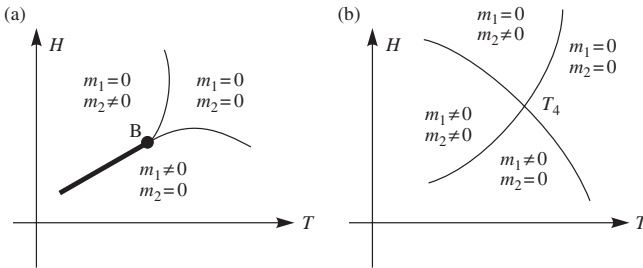
FIG. 2.4. Phase diagram of a two-sublattice anisotropic antiferromagnet in terms of the external field along the easy direction, H , and the temperature T : (a) the heavy solid line indicates a first-order boundary that ends at a bicritical point B ; the light solid lines represent second-order transitions; (b) there are four lines of second-order transitions meeting at the tetracritical point T_4 .
