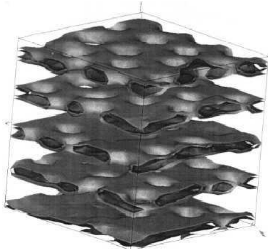
FIG. 7.21. Sketch of a typical perforating lamellar structure of a mesh phase. There are holes filled with the solvent in the original lamellar structure [42].
