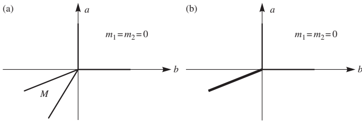
FIG. 2.6. (a) Phase diagram for ce - d^2 > 0 . There is a mixed phase ( M ) and four lines of second-order transitions meeting at the origin (tetracritical point); (b) Phase diagram for ce - d^2 < 0 . There is no mixed phase. The first-order line, drawn as a heavy solid line, given by a = b(c/e)^{1/2} , meets the second-order lines ( a = 0 and b = 0 ) at the origin (which is now a bicritical point).
