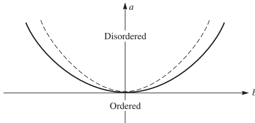
FIG. 2.9. The heavy solid line ( a = b^2/4 ) is the first-order boundary between the nematic and the disordered phase. The dashed line ( a = 2b^2/9 ) is the limit of stability of the ordered solution.
