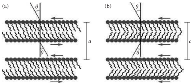
FIG. 4.5. Sketch of two tilted lamellar phases, with oriented interfaces: (a) anti-parallel surfaces in a lamellae; (b) parallel surfaces or chevron-type.
