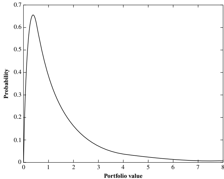
Figure 5.5 A lognormally distributed portfolio.
