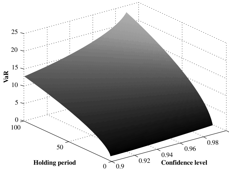
Figure 2.9 A VaR surface.
