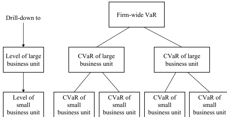
Figure 7.4 Multiple-level risk decomposition and drill-down capability.
