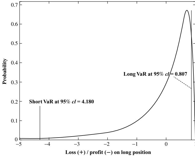
Figure 5.8 Lognormal VaRs for long and short positions. Note: Estimated with the ‘lognormalvarfigure’ function, assuming the mean and standard deviation of geometric returns are 0 and 1, and with initial positions worth plus or minus $1.
