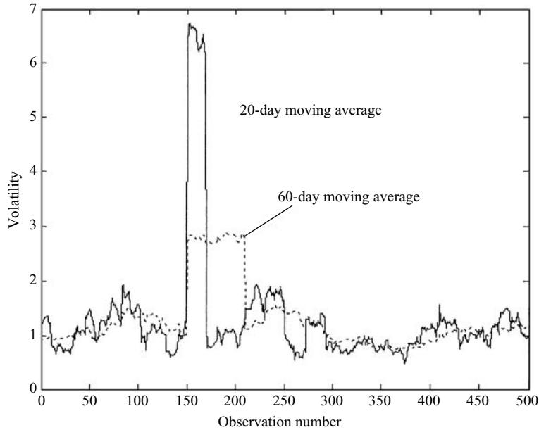
Figure T7.1 Historical volatilities.
