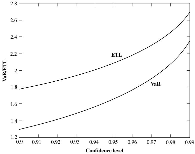
Figure 2.11 ETL and the confidence level. Note: Produced using the 'normalvaretplot2D_cl' function.
