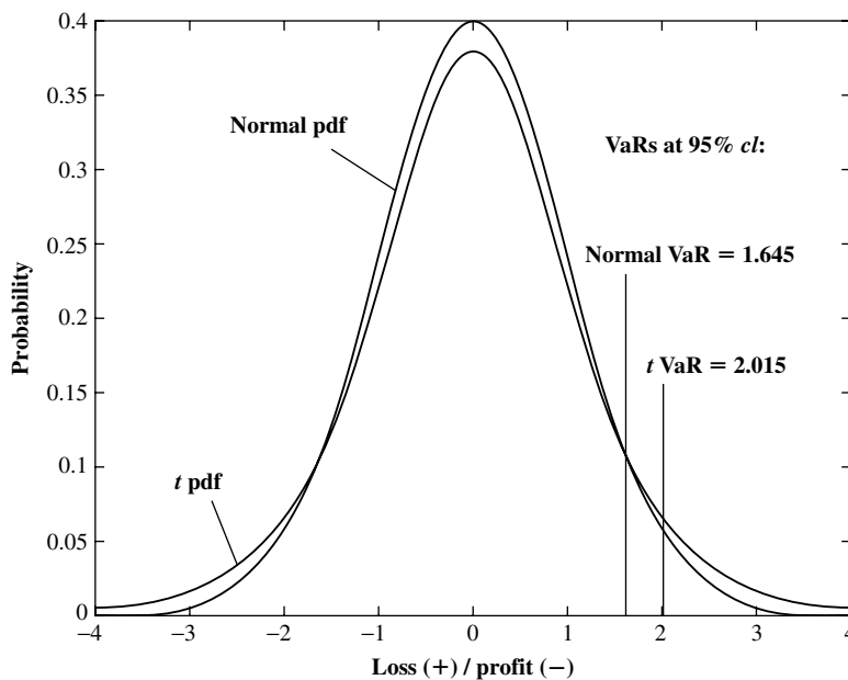
Figure 5.4 Normal VaR vs. fat-tailed VaR.
