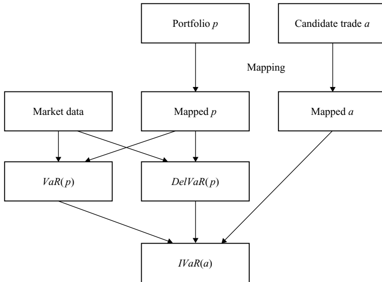
Figure 7.3 The delVaR approach to IVaR estimation. Note: Adapted with permission from Garman (1996c, figure 3).
