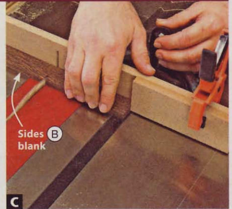
C Without changing the setup used to cut the body (A) to finished size, cut two sides (B) to length from the blank.
