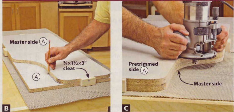
B To easily draw a line about \frac{1}{8} " from the large curved area of the master side onto a side (A), use a \frac{1}{4} " flat washer as a guide for a pencil.
