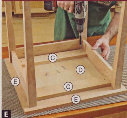
E Drill pilot holes into the tall-table top (D/E) using the shank holes in the cross-rails (C) of the base as guides. Drive the screws.
