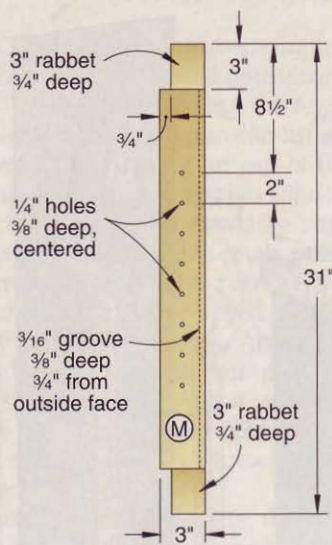
TOOL BASE STILE (Left front inside face shown)
