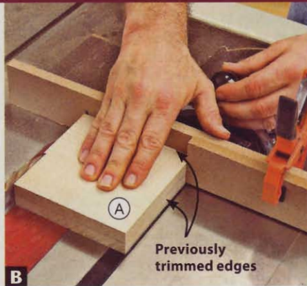
B With one previously trimmed edge against the extension, cut the body (A) to width, and then rotate and cut again.
