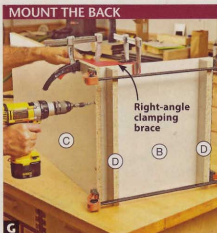
G Clamp a back (C) to a bottom large shelf/base trim assembly (B/D), flush with the shelf bottom. Drill the holes, and drive the screws.
