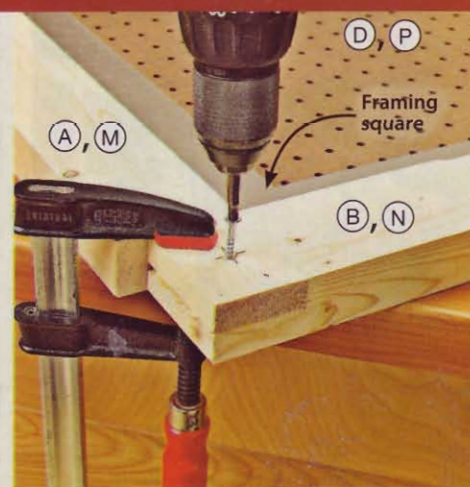
TOOL CABINET STILE (Left front inside face shown)
