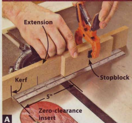
A Clamp a stopblock to the miter-gauge extension 5" from the saw kerf. The ruler raises the stopblock for sawdust relief.
