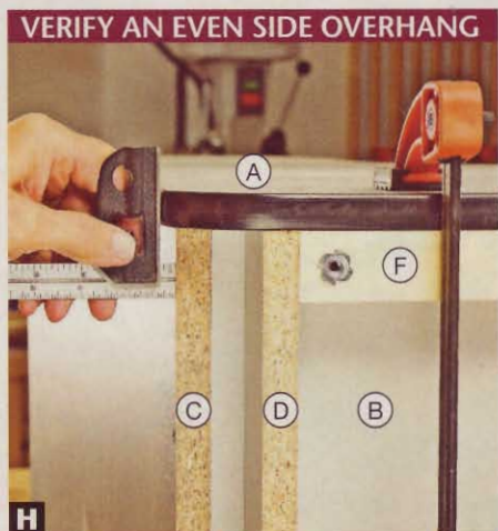
H Using a combination square, check that the side (A) overhangs the back (C) evenly along the length to ensure a square assembly.
