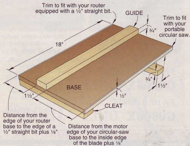
To clean out the rabbets, start with the router edge of the jig \frac{3}{8} " from the stile ends, and make repeat router cuts to the saw kerf.
