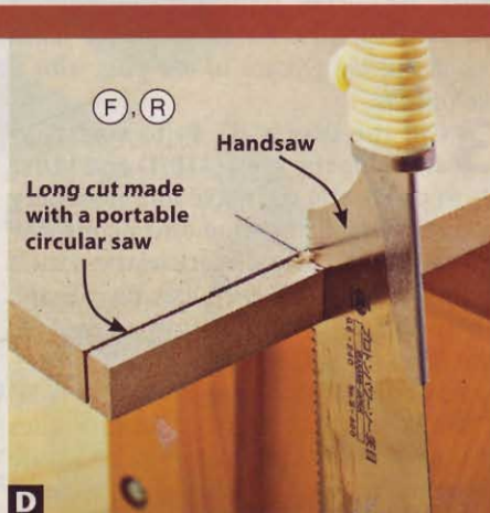
D After making the long cuts with a portable circular saw, finish cutting the notches with a handsaw.
