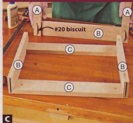
C Glue, biscuit, and clamp the tall-table back leg/rail assembly (A/B) to the side rail/cross-rail assembly (B/C), ensuring tight joints.
