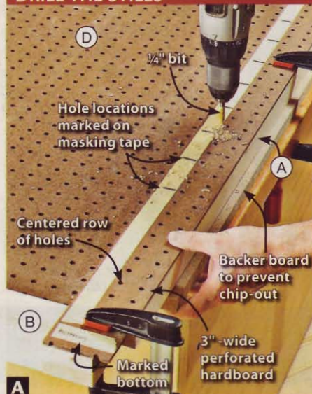
Mark hole locations on masking tape applied to a perforated hardboard strip. Using the strip as a guide, drill the holes in the stile (A).
