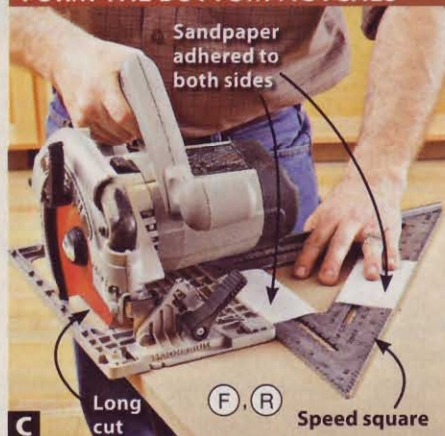
C To make the long cuts, adhere sandpaper to a speed square to keep it from slipping. Then use it to guide your portable circular saw.
