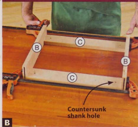
B With the parts upside down for easy alignment, glue, biscuit, and clamp together the tall-table side rails (B) and cross-rails (C).
