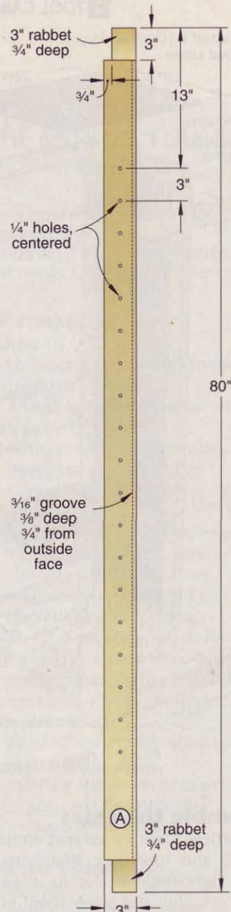
TOOL CABINET STILE (Left front inside face shown)
