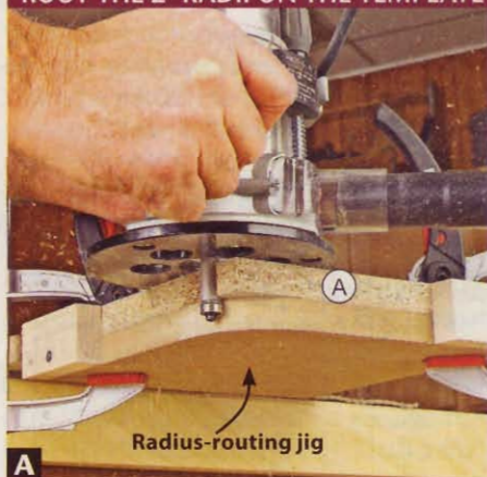
A Using a flush-trim bit and the radius-routing jig as a guide, rout the four 2" radii at the corners of the "master" side (A).
