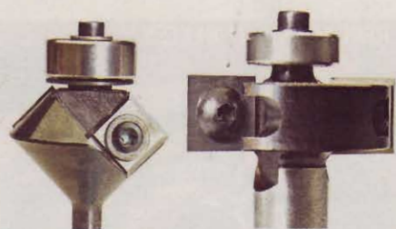
Both the Freud 45° chamfer bit and CMT rabbeting bit use four-edged replaceable cutters to extend bit life.
