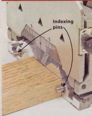
Using the Domino's retractable indexing pins to reference from workpiece edges or ends ensures perfect alignment of the mortises.
