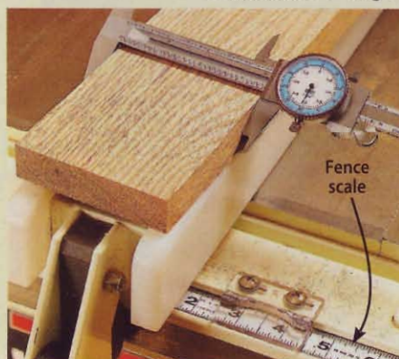
Installing a different blade or adjusting the fence parallel to the blade can throw off your tablesaw fence scale's accuracy.
