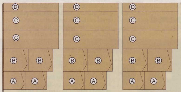
3/4 x 48 x 96" Medium-density fiberboard
