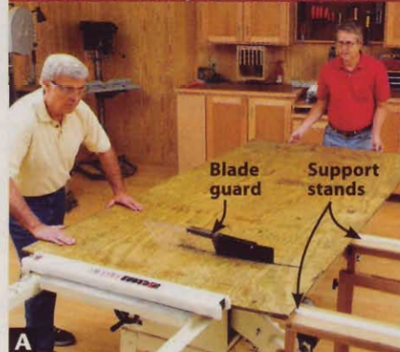
A Position at least two support stands behind the saw and a helper at the side.
