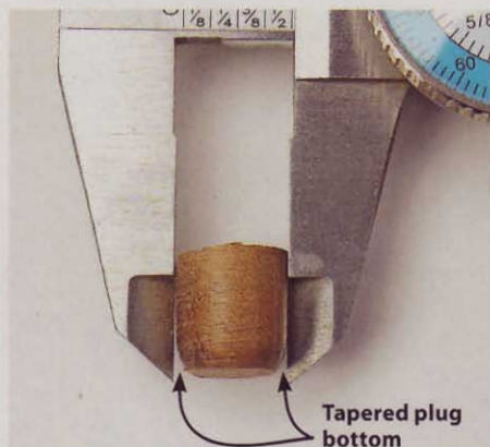
A tapered plug has two major benefits over non-tapered plugs: It's easier to start and produces a snug fit at the top of the hole, where it matters most.
