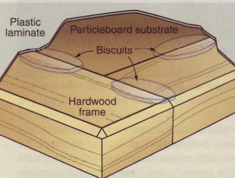
The hardwood frame provides a more rigid, durable surface than the particleboard for clamping workpieces to the table.
