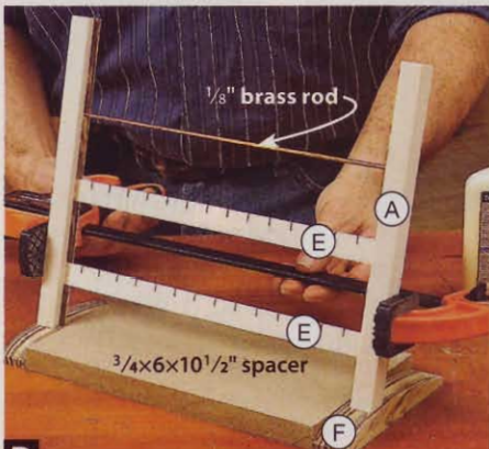
D ASSEMBLE THE STAND
