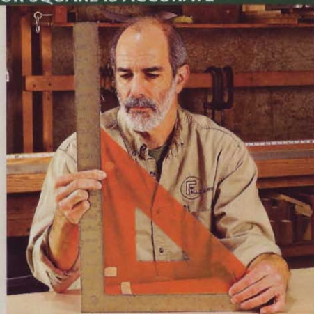
A Keep several plastic drafting squares, including a 12" model for maximum surface contact, in your shop to check tools.
