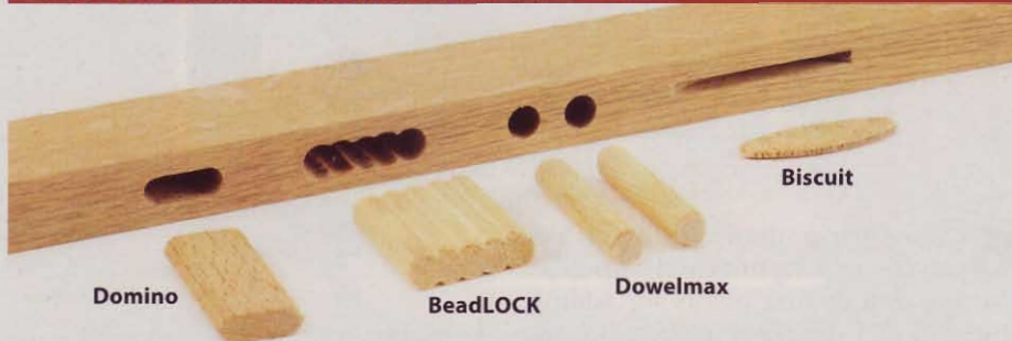
Shown are four types of loose tenons with their mortises, as machined by the tools in our test.
