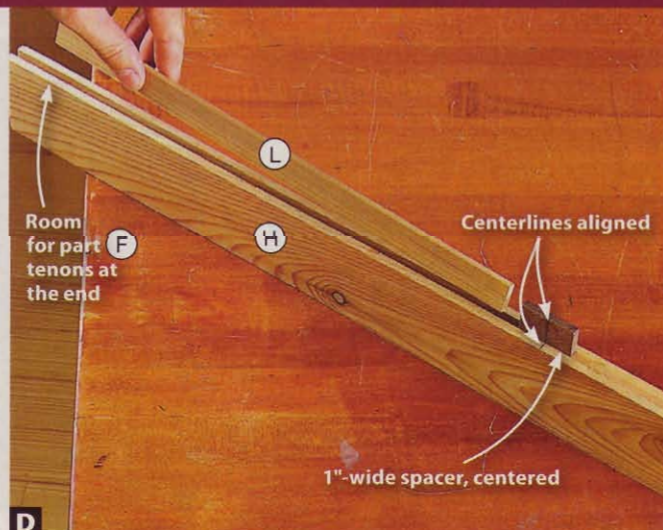
D With the 1"-wide spacer centered in the top end rail (H) groove, insert the long fillers (L), leaving room for the top side rail (F) tenons.
