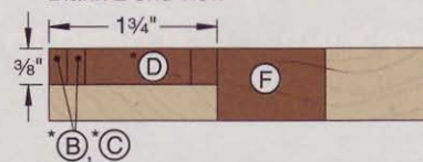
Blank 2 end view
