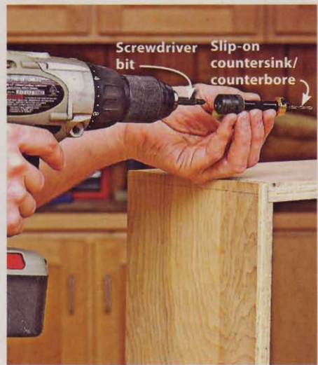
The Jack Rabbit set saves time by letting you mount the countersink/counterbore bit over a screwdriver bit chucked in your drill.
