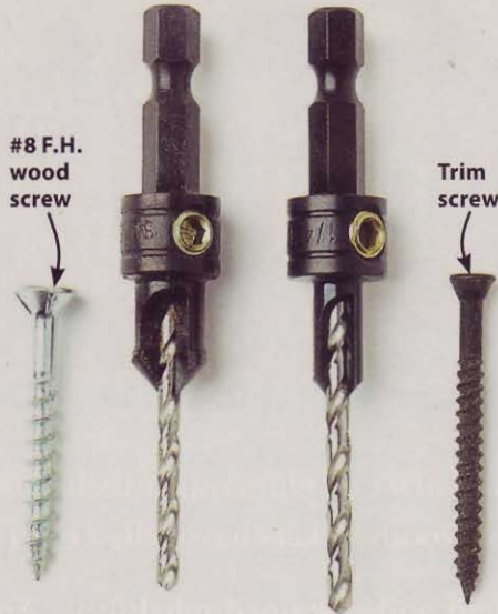
Match the countersink/counterbore to your screw head's diameter. The bit on the right has a 1/4" counterbore for trim screws.
