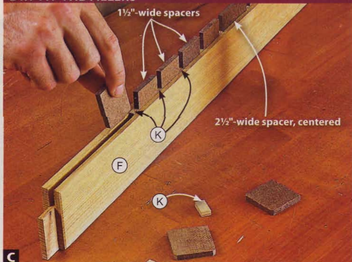
C With the 2 1/2"-wide spacer centered in the top side rail (F) groove, alternately insert short fillers (K) and 1 1/2"-wide spacers.
