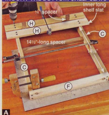
A With the inner long shelf slat (H) in place, mount another long shelf slat at the front with ¼" spacers inserted between the slats.
