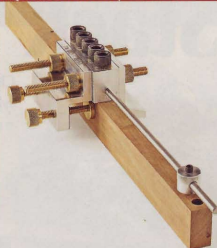
Dowelmax's extension indexing rod allows you to accurately reference the jig from previously drilled holes, as shown, or the end or edge of a board.
