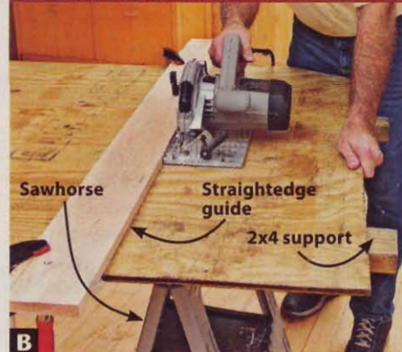
B Clamp a straightedge guide to the panel. Keep the saw tight against the guide.
