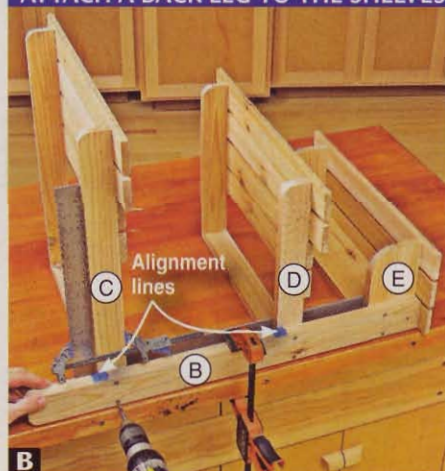
B Using a framing square to position each shelf at 90°, drill the holes and screw-mount the back leg (B) to the shelves.
