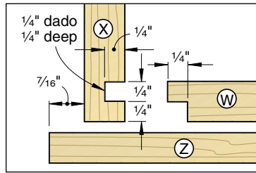
7a DRAWER JOINT DETAIL
