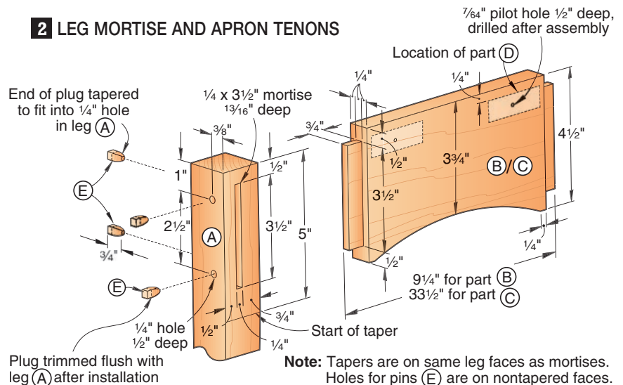
To avoid splitting, clean up the ends of the leg (A) mortises using a ¼" chisel. Then pare the sides using a chisel at least ¾" wide.
