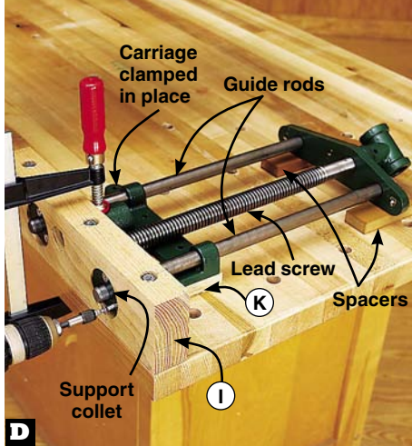
D Using the holes in the support collets as guides, drill \frac{5}{32} " pilot holes into the jaws and drive the supplied #14 \times 1 \frac{1}{2} " flathead screws.
