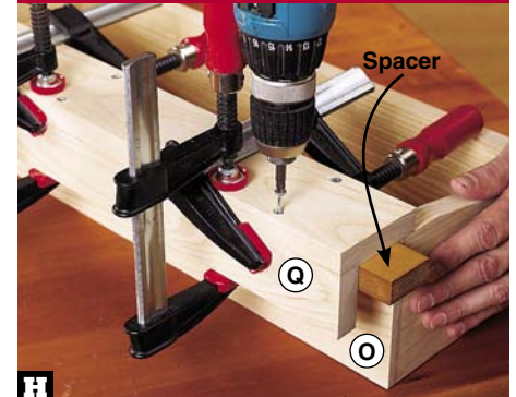
Clamp a 1⅙"-wide spacer between the cleat (Q) and back (O). Then drill countersunk screw holes, and drive the screws.
