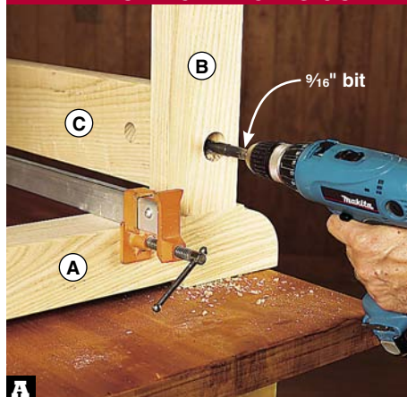
A Clamp the stretchers (C) between the end assemblies. Using the holes in the uprights (B) as guides, drill into the stretcher ends.
