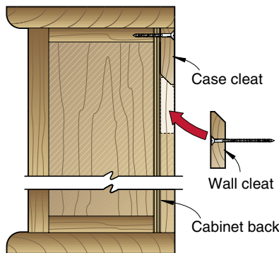
Hidden cleats allow the cabinet back to hang flat against the wall. We used this method to hang the display shelf.
