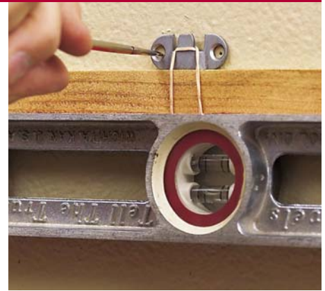
An awl marks mounting screw locations for the two clips used here. This method works just as well for spacing three or more clips.
