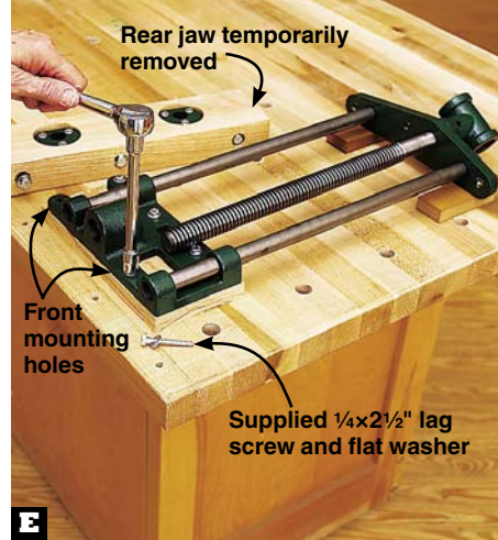
E Using the two front holes as guides, drill shank and pilot holes and finish fastening the carriage with lag screws and washers.
