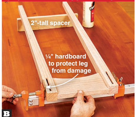
Glue and clamp together a pair of legs (A) and a side apron (B). Position a 2"-tall spacer under the legs to keep them aligned.
