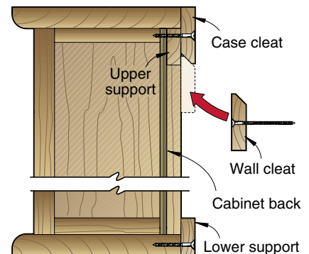
Exposed-cleat cabinets stand out from the wall, but are easily moved along a continuous cleat rail. This works great for shop cabinets.
