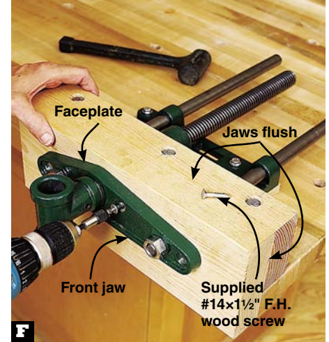
F Using the three holes in the faceplate as guides, drill \frac{5}{32} " pilot holes into the front jaw. Screw the jaw to the faceplate.
