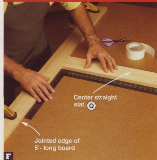
Apply double-faced tape to the back of a straight slat (Q). Center it on the jointed edge of a 5'-long board, align it with a framing square, and stick it to your workbench.
