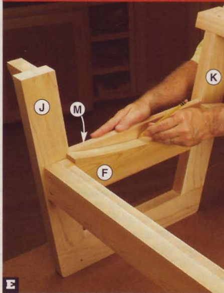
Position the seat support cover (M) between the front and rear legs (J, K) and tight against the seat support (F). Trace the profile of the seat support onto the seat support cover.
