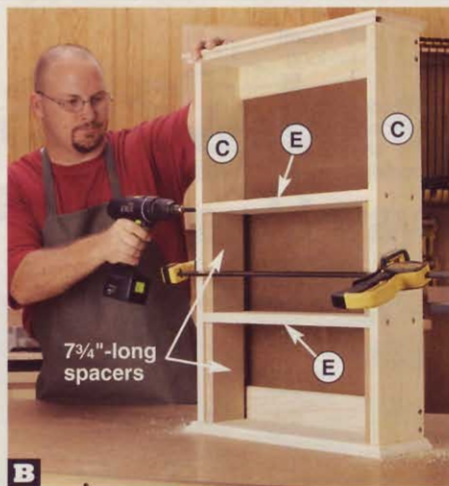
B Inserting 7\frac{3}{4} "-long scrap spacers, position the shelves (E) between the sides (C). Drill counterbored screw holes centered on the shelves' thickness, and drive the screws.
