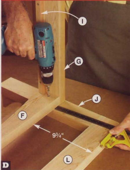
With the outer side of the side assembly facedown, position the seat frame 9\frac{3}{4} " from the bottom edge of the lower side rail (L). Drill screw holes, and drive the screws.
