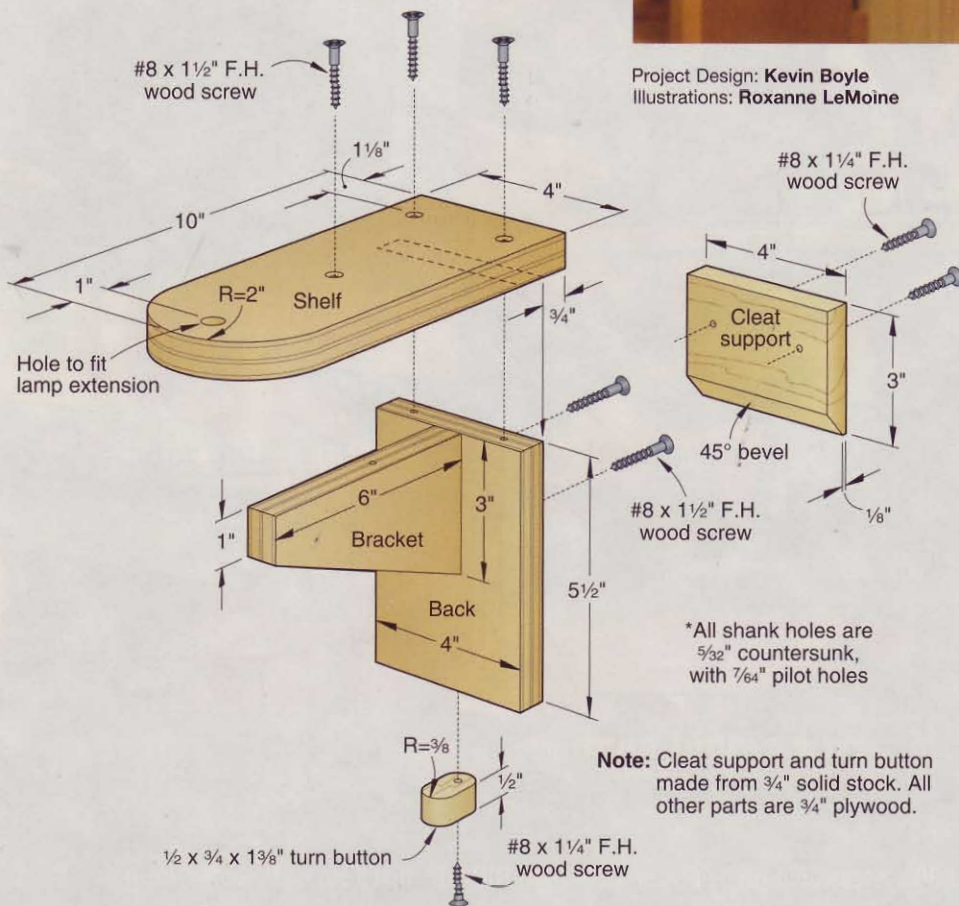
Rotate the turn button to secure the light support to the wall cleat.
