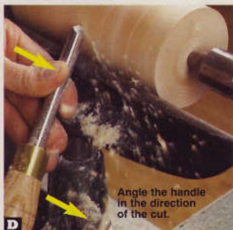
D Position the tool with one of its bevels riding flat on the workpiece, with the handle angled in the direction of the cut. Slightly rotate the tool, engaging the half of the cutting edge closest to its heel. Now advance the tool along the length of the workpiece.
