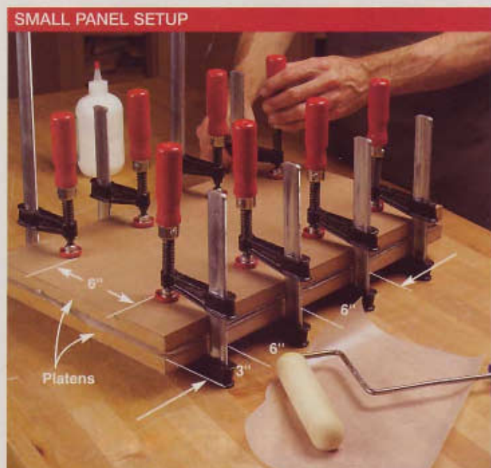
When veneering panels with only platens and clamps, position clamps 3" from each end and no more than 6" apart along the panel's length. Maintain 6" spacing between clamps on opposite sides of the panel.
