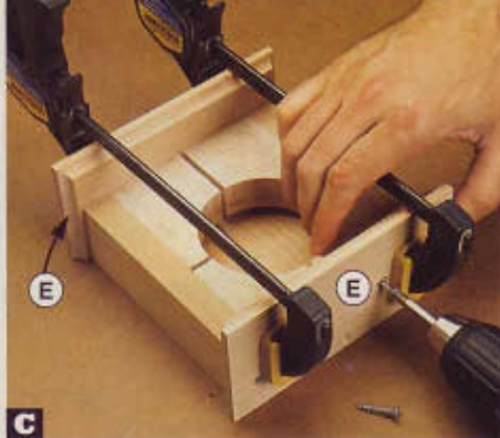
C Center the sub top and bottom (E) side-to-side on the clock case. Drill pilot holes, and drive the screws.
