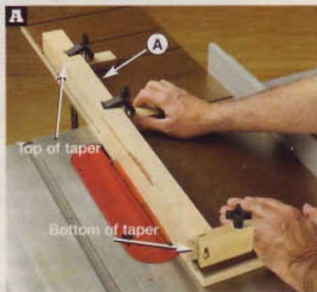
After marking the taper's upper end on the leg's side and its lower end on the leg's bottom, cut the tapers using a tapering jig.
