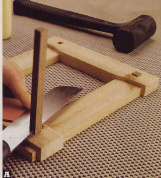
A With a 3/32" spacer placed under a flush-cutting saw, trim the corner-pin blank, leaving the pin proud of the rail's surface.
