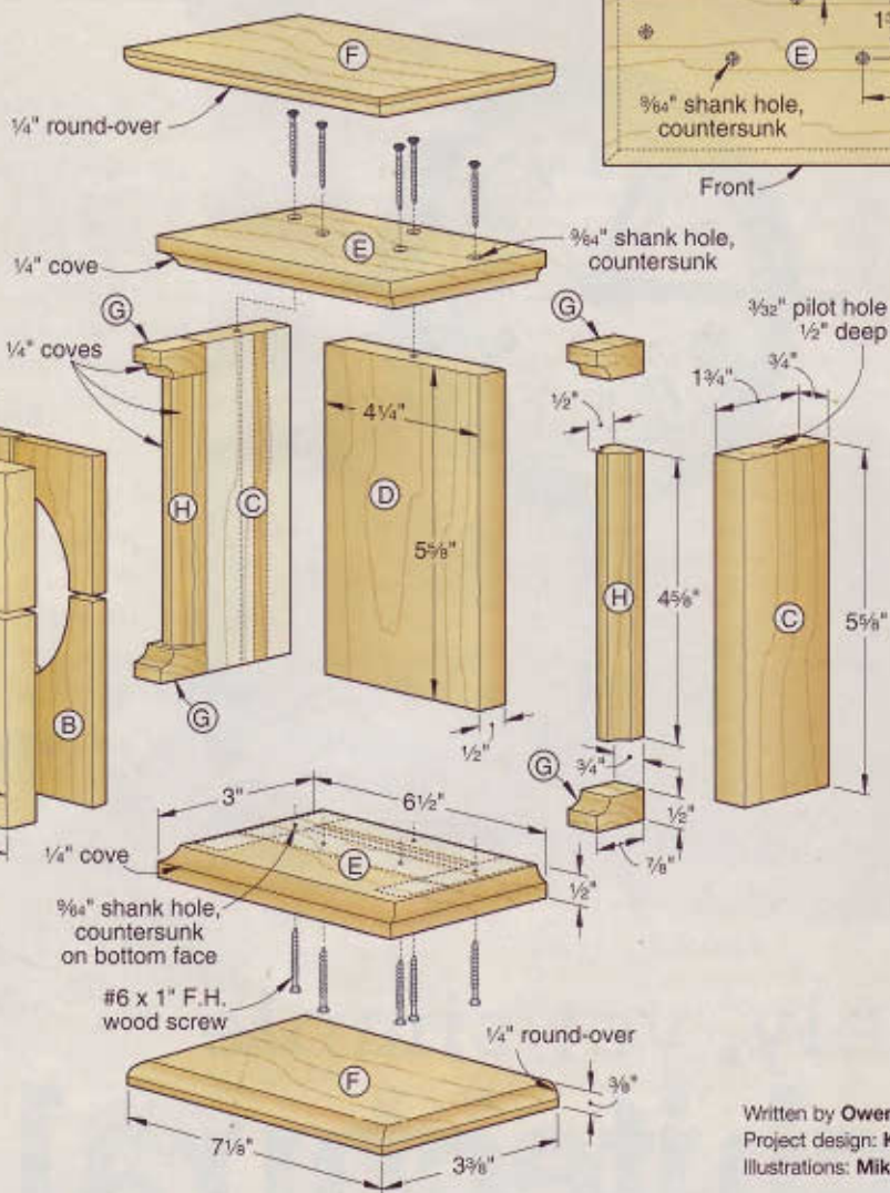
C Center the sub top and bottom (E) side-to-side on the clock case. Drill pilot holes, and drive the screws.
