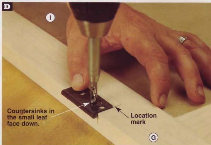
With its barrel tight against the door stile (G), align each hinge with its location mark. Using the holes in the hinge's small leaf as guides, drill screw pilot holes.
