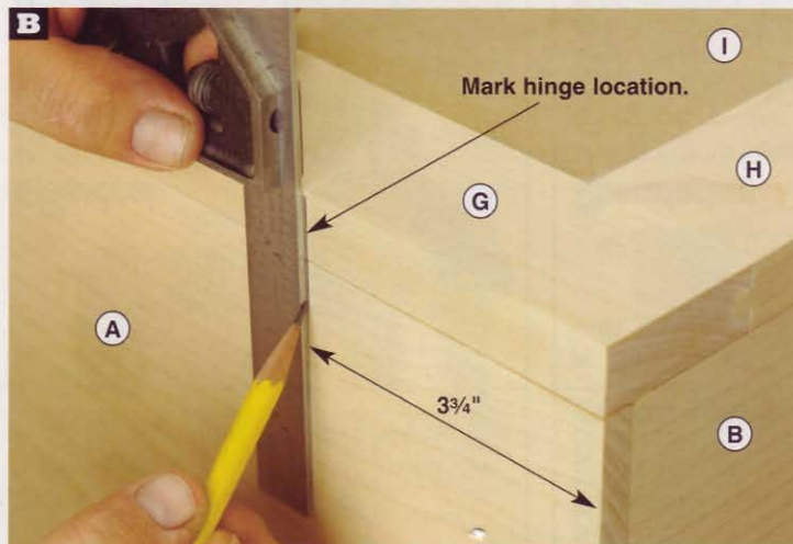
Position the door flush with the cabinet's top, bottom, and sides, and clamp it in place. Then mark the location of the top of the top hinge and the bottom of the bottom hinge.
