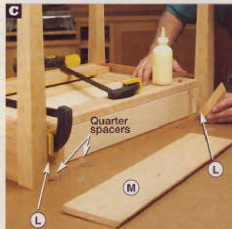
Using quarters to space the sleeper faces (L) \frac{1}{16} " from the workbench surface, glue, biscuit, and clamp them in place. A second pair of quarters awaits the drawer face (M).
