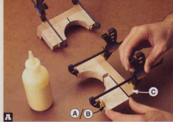
A Glue the mirror-image pair of face/backer pieces (A/B) to each side (C), aligning the pieces with the side's ends and front edge.
