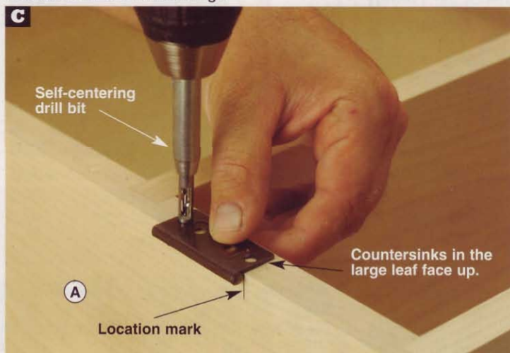
With its barrel tight against the side (A), align each hinge with its location mark. Using the holes in the hinge's large leaf as guides, drill screw pilot holes.
