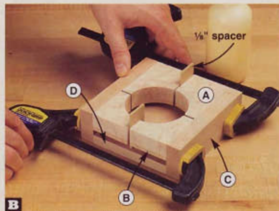
B Glue the side assemblies (A/B/C) to the back (D), inserting 1/8" spacers between the assemblies to keep them square.
