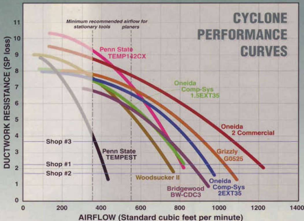
Tests were conducted using pilot tube and manometer at dust-collector inlet, and ductwork the same diameter as the inlet. Duct length was 10 times its diameter to stabilize airflow for accurate measurements. Filters were seasoned, emptied, and tapped clean before test to simulate workshop conditions.
