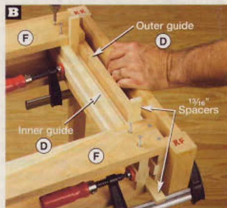
Insert \frac{13}{16} "-wide spacers between the outer and inner guides (D), and clamp the inner guide in place. Using the holes in the rails (F) as guides, drill pilot holes, and drive the screws.
