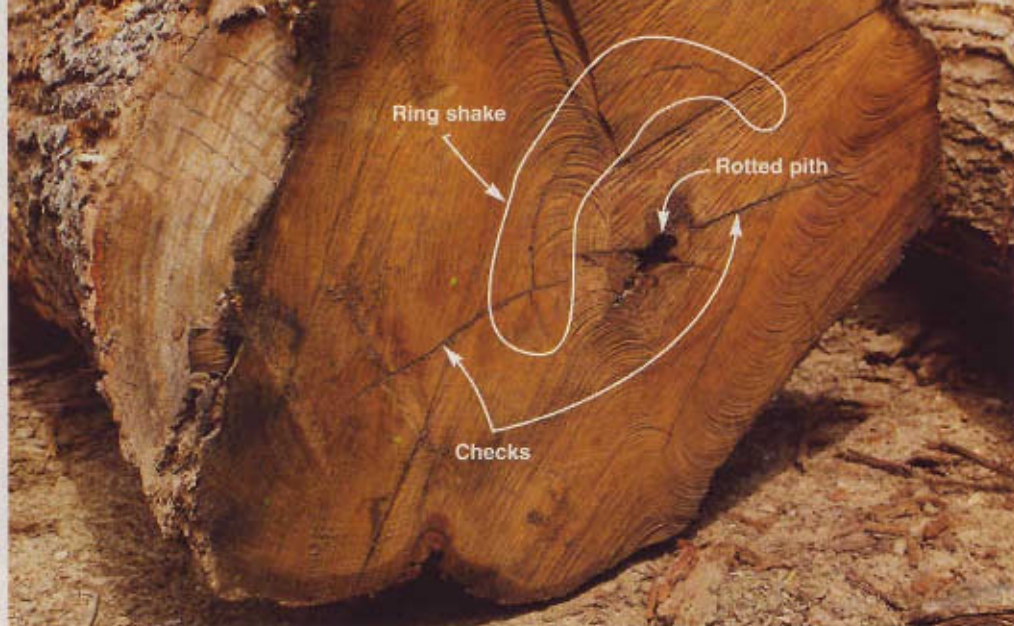
The butt of this log shows a few ills, but an experienced eye can tell the log remains suitable for milling. If these conditions progress, though, much of the wood will go to waste.
