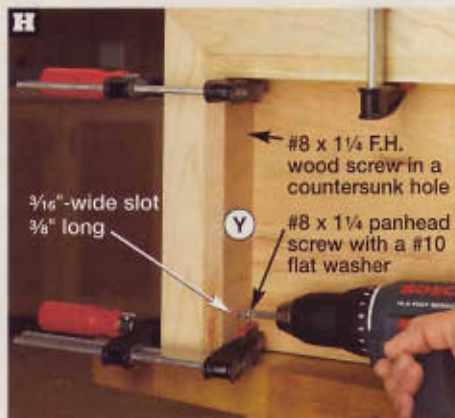
With the miter and front 2" of the side crown glued, clamp it in place. Drill pilot holes and drive a #8x1 1/4" flathead wood screw in the hole and a #8x1 1/4" panhead screw with a #10 flat washer in the slot.
