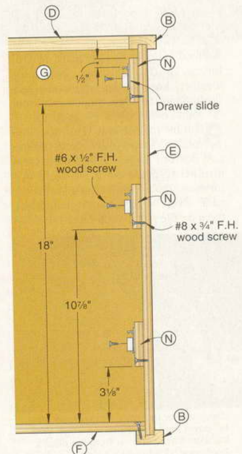
B With their ends against the cabinet's bottom, use a pair of 18"-long spacers to position the top cleats. Then glue and screw the cleats in place.
