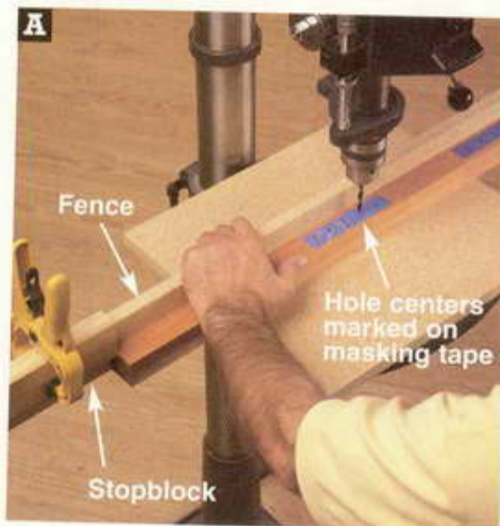
Mark the right-rear leg shelf-support hole centers on masking tape. Align each mark with the bit, and position a stopblock. Drill all four legs at each stopblock position.
