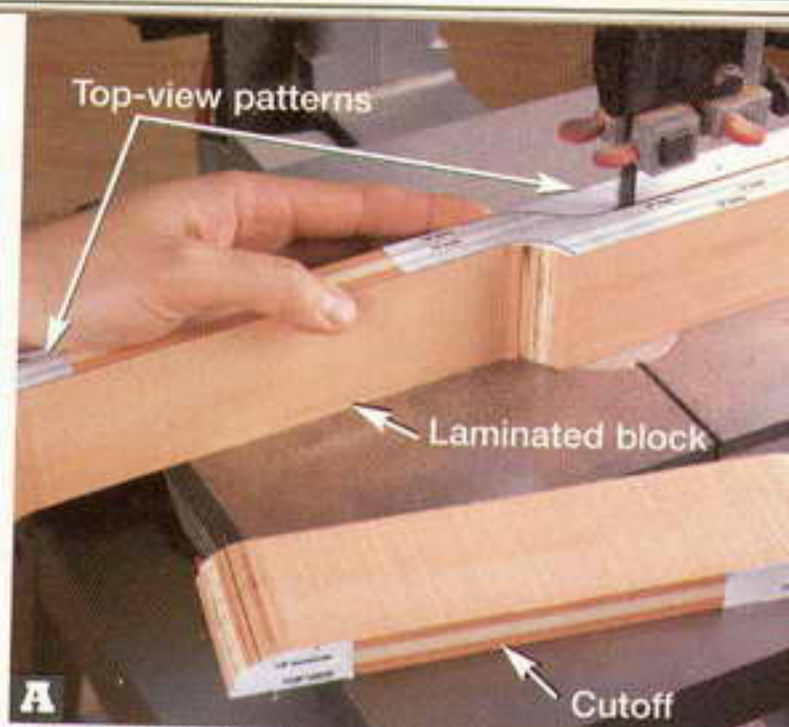
A Bandsaw the laminated block, staying just outside the top-view pattern lines. Save the cutoffs for reattachment to the block.
