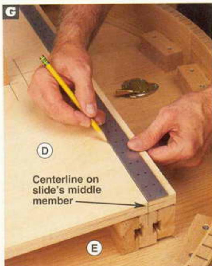
Mark the center of each slide's middle member on its ends. Draw lines across the platform, connecting the marks.
