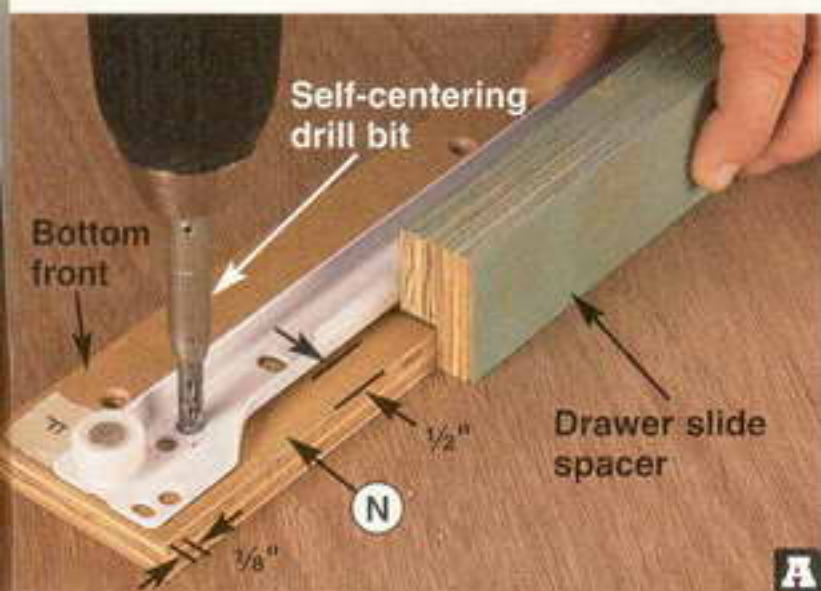
Use a spacer to position the drawer slide 1/2 inch down from the cleat's top edge. With the slide's front end 1/8 inch from the cleat's front edge, drill the pilot holes.
