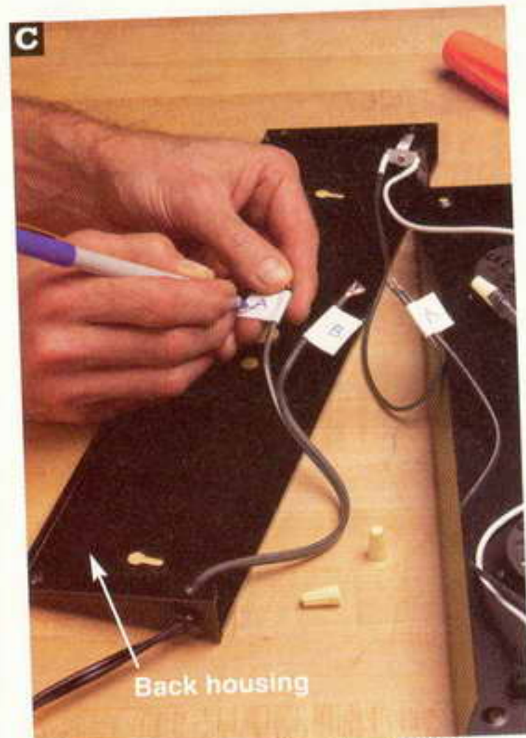
Disconnect the cord from the internal wiring by removing the wire nuts. Mark the wires for proper reassembly.
