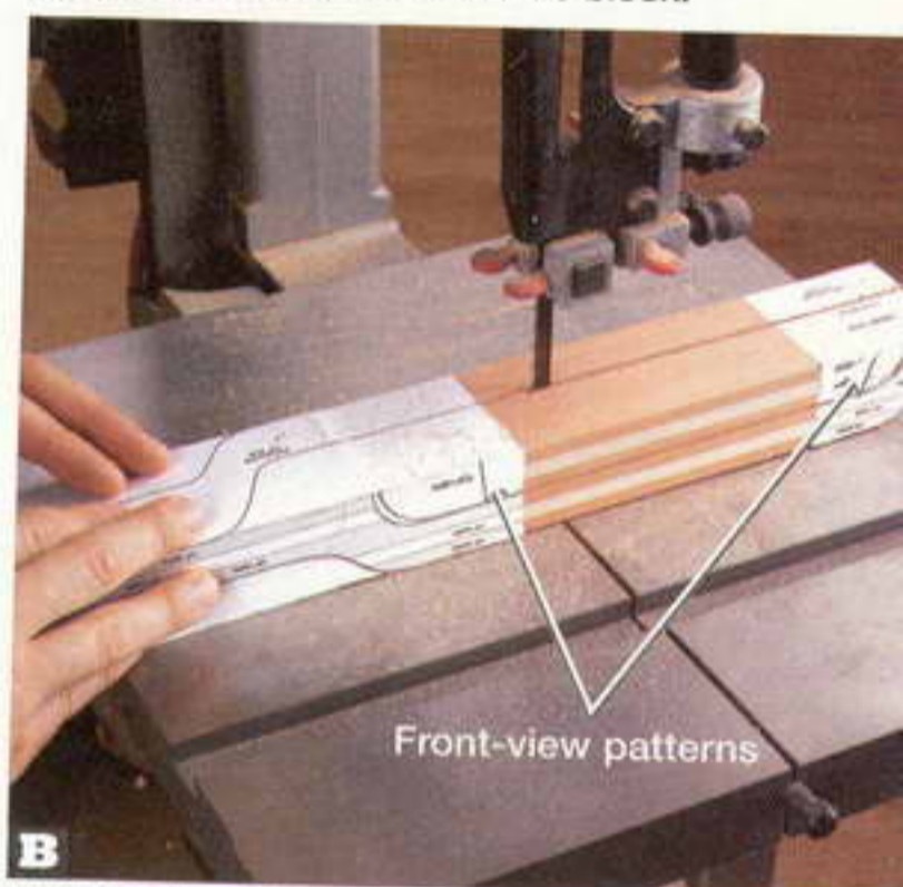
B With the front-view patterns adhered where shown, bandsaw just outside the pattern lines to complete the handle's shape.
