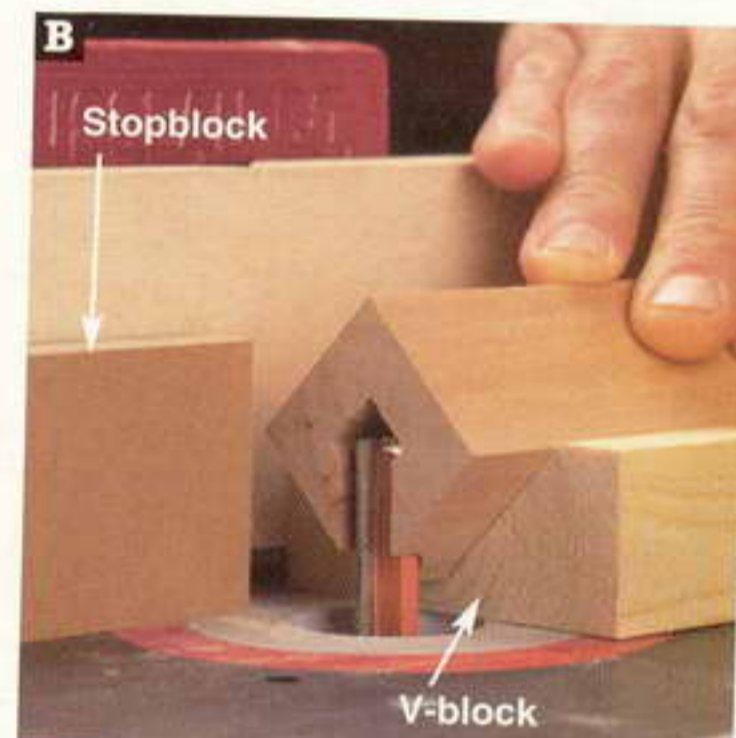
With the right rear leg cradled in a V-block, rout the top and bottom 1/2"-long notches in progressive 1/8" increments. Clamp a stopblock to the fence to control the depth.
