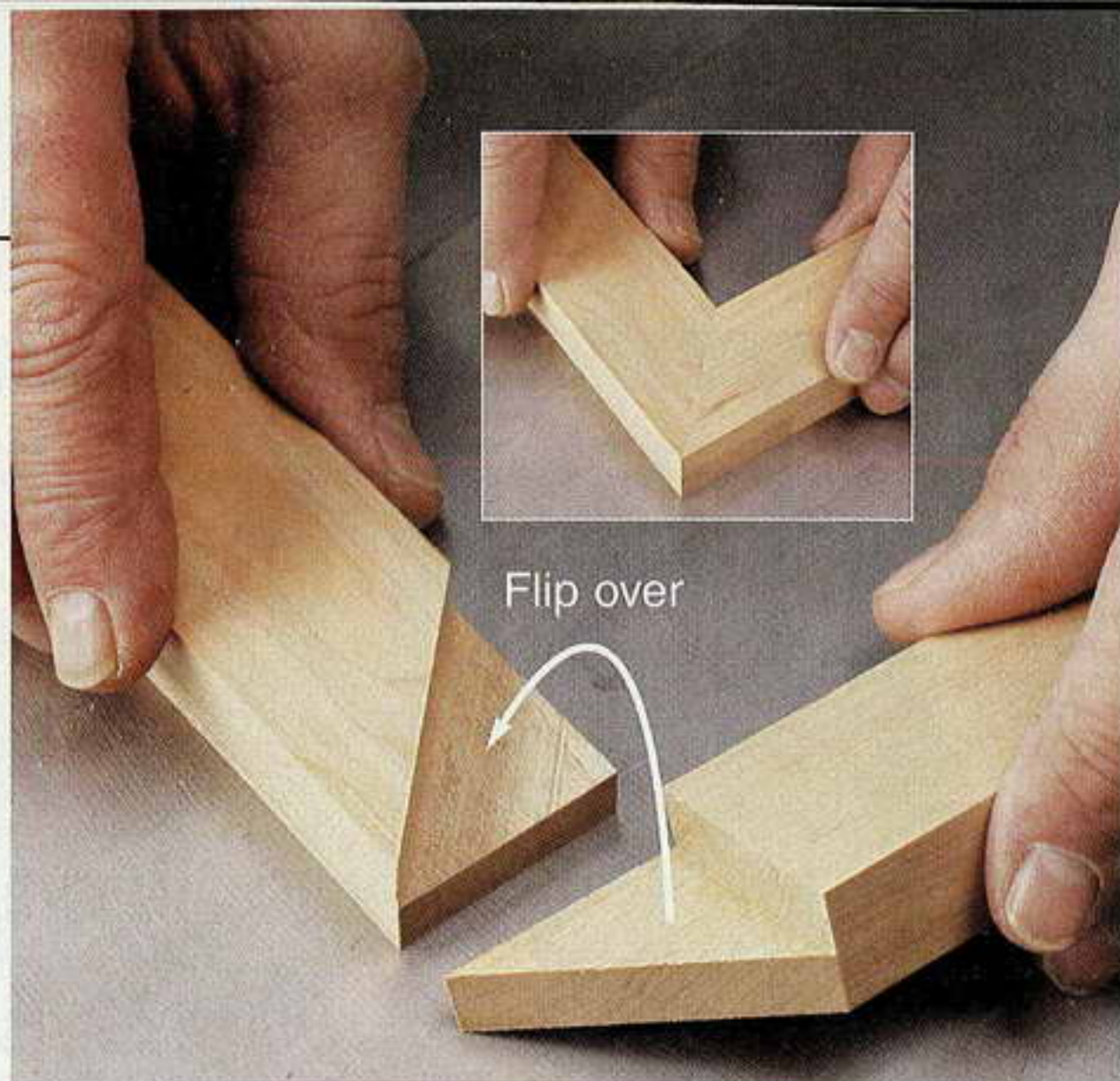
A mitered half-lap joint consists of two parts like the ones shown here. Just flip the piece at right, and the mating miters form the completed joint, inset. We placed the exposed end grain at the top and bottom of the frame.
