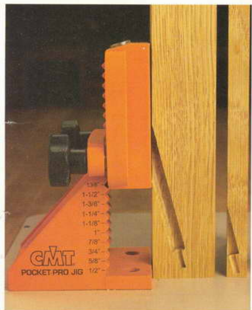
Whether you're making pocket holes in 1/2"-thick drawer sides (right), 1 5/8"-thick bed rails (left), or something in between, the Pocket Pro easily adjusts to any 1/8" increment within that range.
