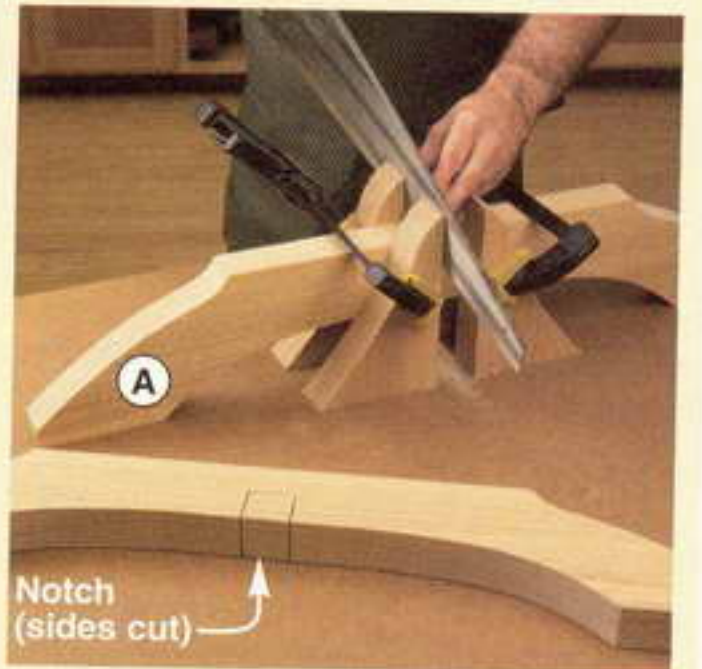
With the bottom cutoff removed, cut the sides of the notch, keeping the saw tight against the end cutoffs.
