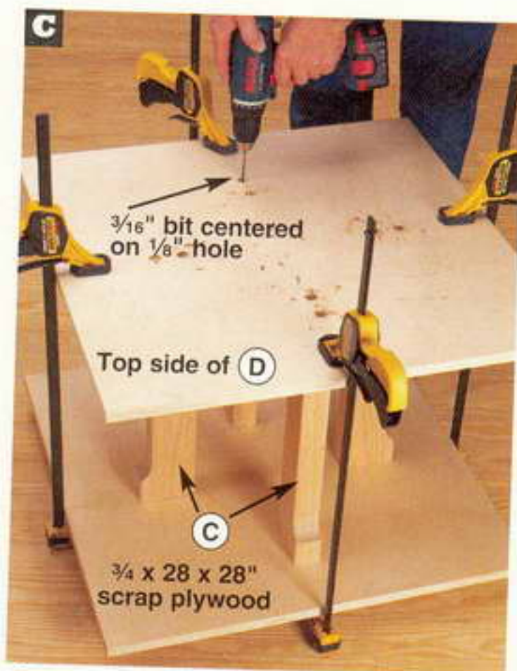
Centering a \frac{3}{16} " bit on the platform's \frac{1}{8} " holes, drill a pair of 1\frac{3}{4} "-deep pilot holes in each leg (C).
