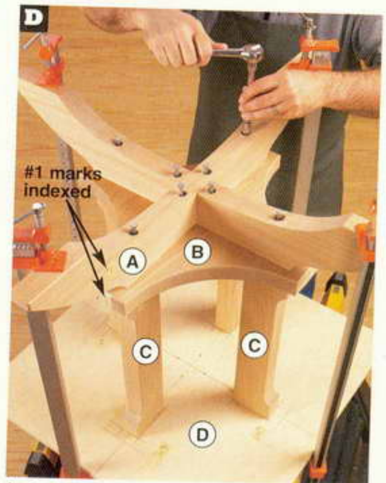
Index the feet (A) on the base (B), and align their mounting holes. Clamp the assembly, and drive the lag screws.
