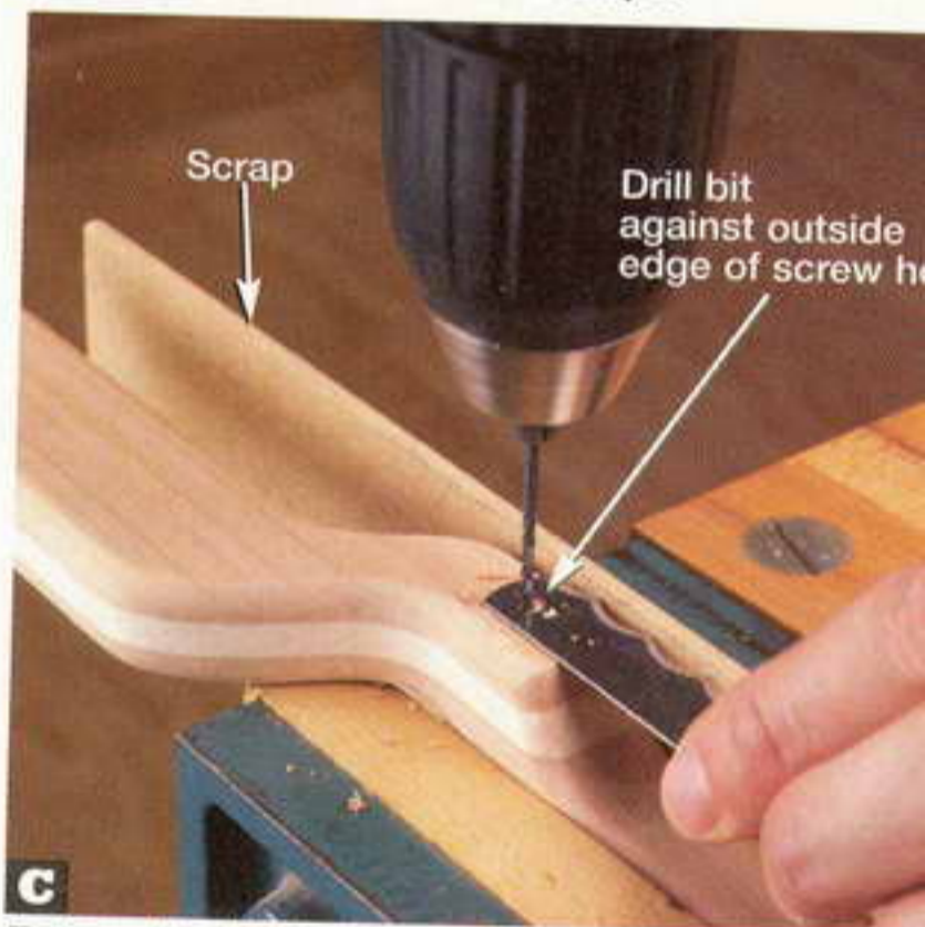
C To keep the blade tight between the screws, drill pilot holes against the outside edge of the blade's screw holes.
