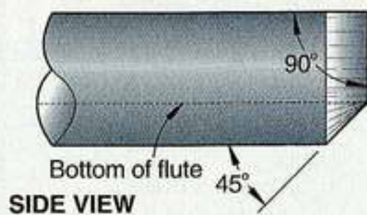
3 3/4" ROUGHING GOUGE
