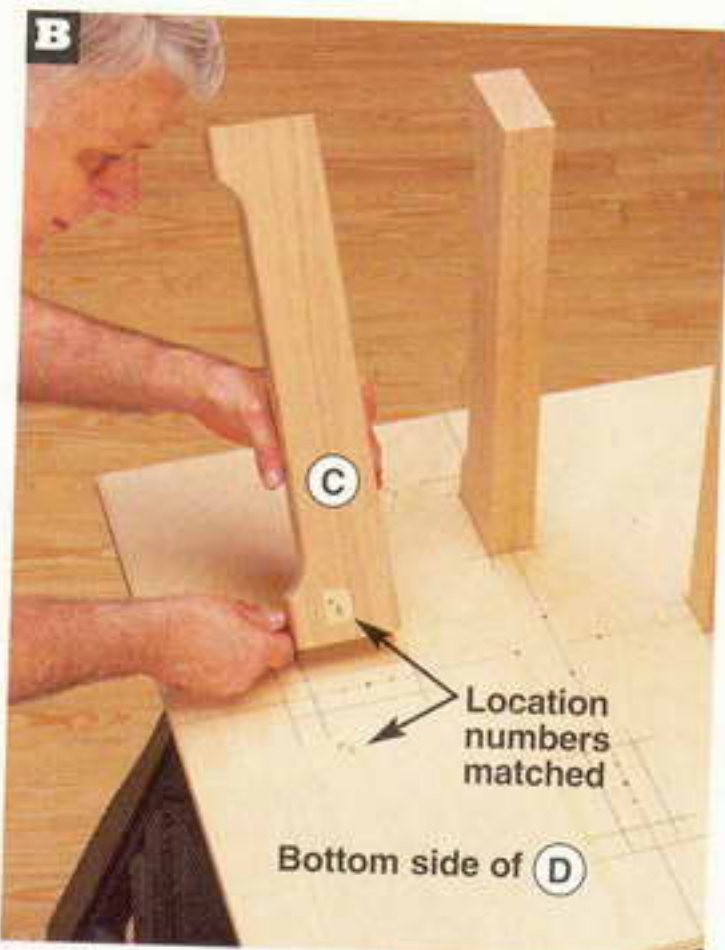
Match the legs (C) to the numbered locations on the slide platform (D). Align the legs with the layout lines.
