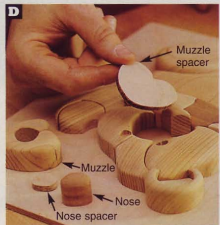
Install the muzzle spacer followed by the muzzle. Then insert the nose spacer and the nose into the muzzle opening.
