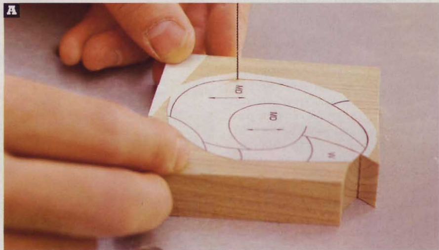
For tight-fitting parts, scrollsaw right down the middle of the intarsia pattern lines.
