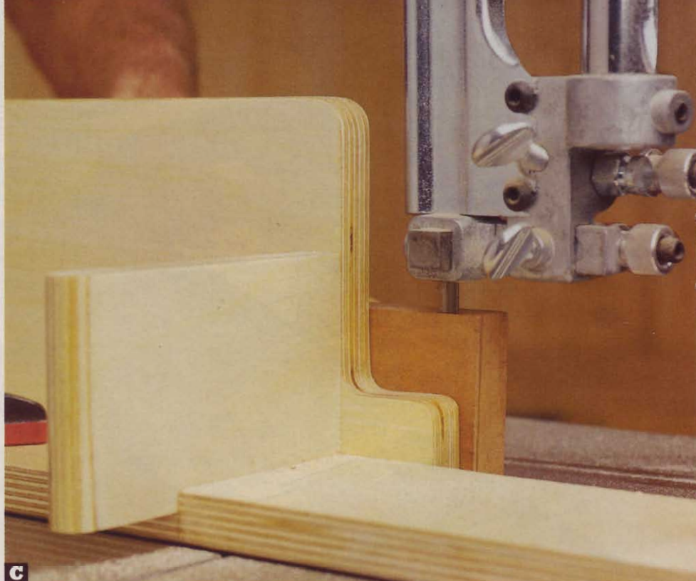
C The cut-out section of the resawing fence allows you to bring the upper blade guides down as low as possible. This step keeps the blade from twisting as you resaw.
