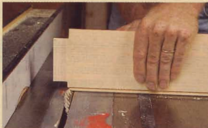
Step 3: Miter-cut just the bead on the tenoned rail, using the miter gauge.
