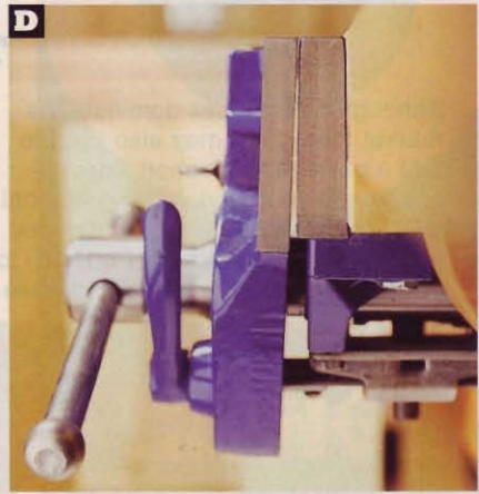
D Toed-in jaws, shown on the Record 52ED, meet at the top first, then become parallel as you tighten them. (Wooden jaw faces removed for clarity.)
