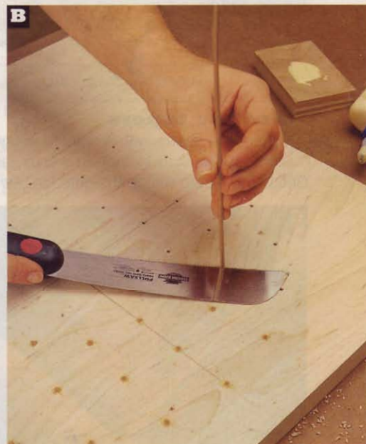
Dip the end of a 1/8" walnut dowel in glue, and then insert it in a hole. Trim the dowel flush. Repeat until all holes are filled.
