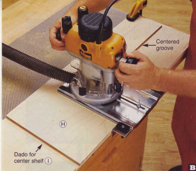
Adjust your router's edge guide to center the bit on the width of a side (H), and rout a groove from the bottom to the dado for the center shelf (I).
