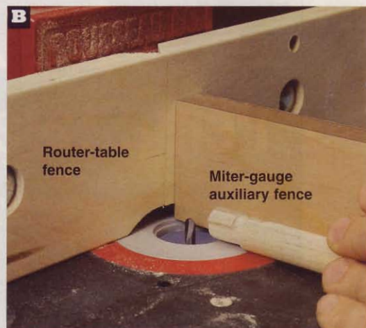
B Push the stock all the way to the fence, and rotate it once counterclockwise. Then nibble away the rest of the waste.
