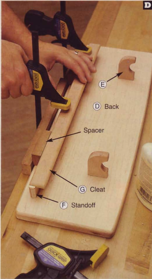
Using 3/4"-thick spacers to position the standoff/cleat assembly, glue and clamp it in place, centered on the back's length.
