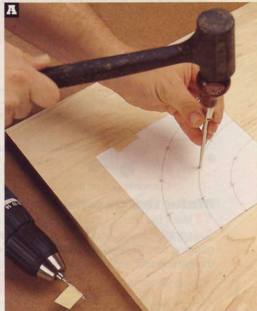
Align the pattern with the quadrant lines, and secure it with masking tape. Use an awl to mark the hole centers.
