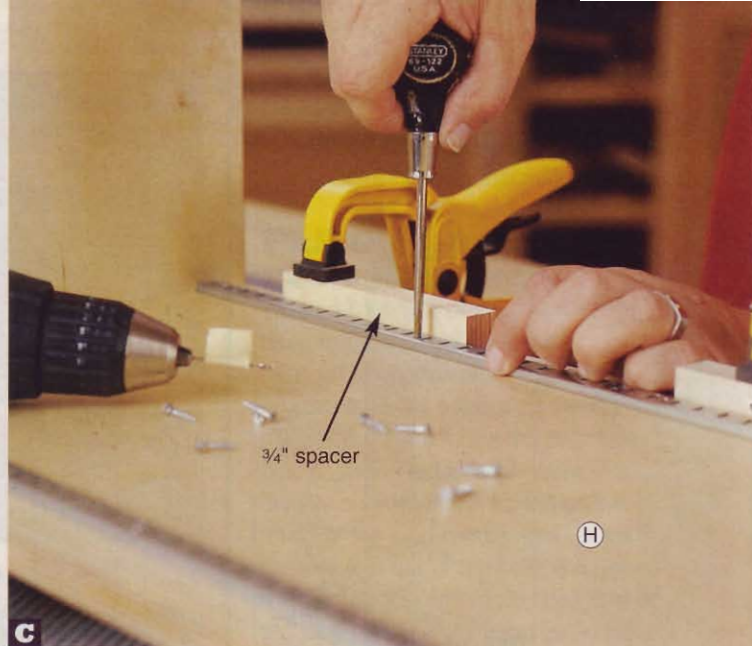
Clamp scrap 3/4" plywood spacers flush to the edges of each side (H). Position the shelf standard against the spacers, and mark the screw holes with an awl.
