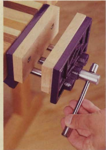
D Toed-in jaws, shown on the Record 52ED, meet at the top first, then become parallel as you tighten them. (Wooden jaw faces removed for clarity.)
