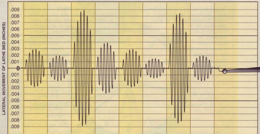
Tests conducted by turning the same bowl blank, mounted between centers, at a no-load spindle speed of approximately 1,400 rpm. A dial indicator, placed against the lathe bed and in line with the blank, measured vibration. All lathes were tested freestanding on a concrete floor.
