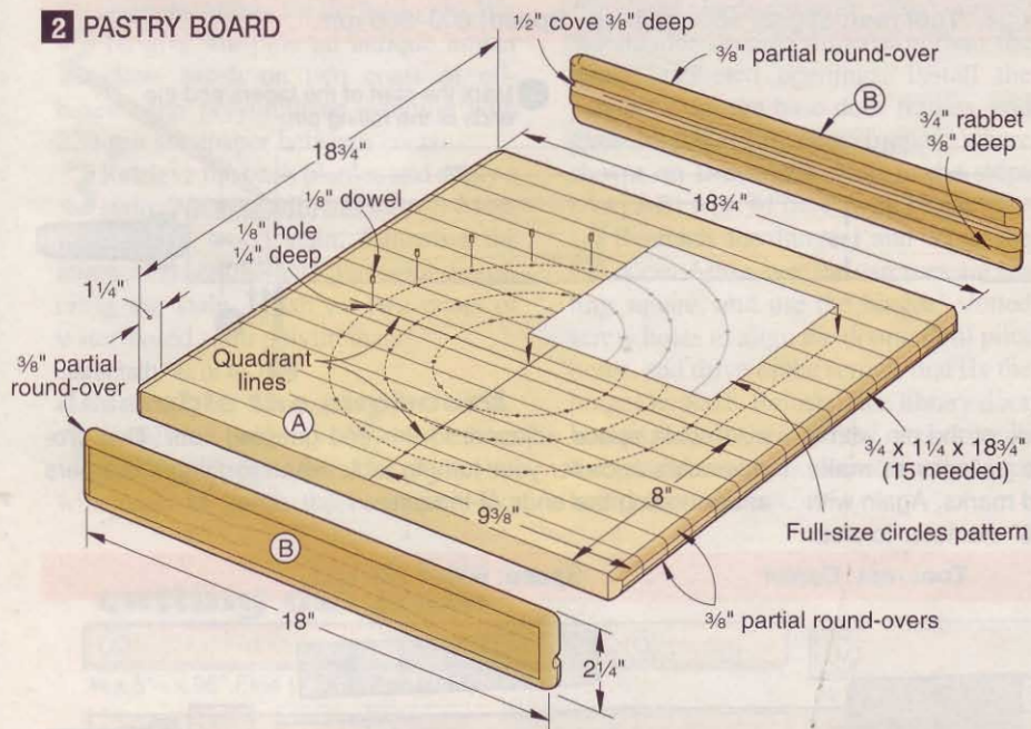
Align the pattern with the quadrant lines, and secure it with masking tape. Use an awl to mark the hole centers.
