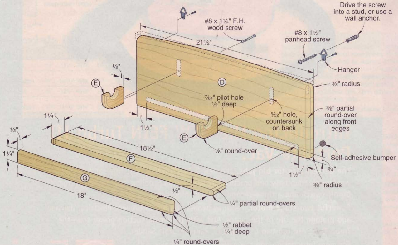
6 WALL RACK EXPLODED VIEW
