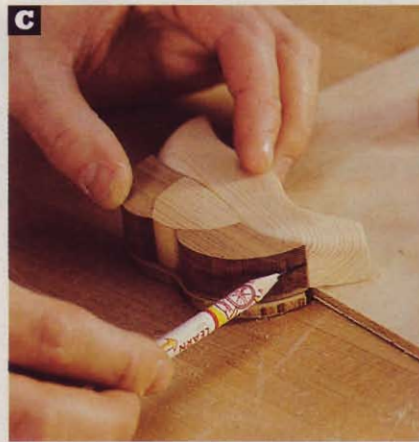
Check the transition between adjacent parts as you contour them. Re-mark and continue sanding as necessary.
