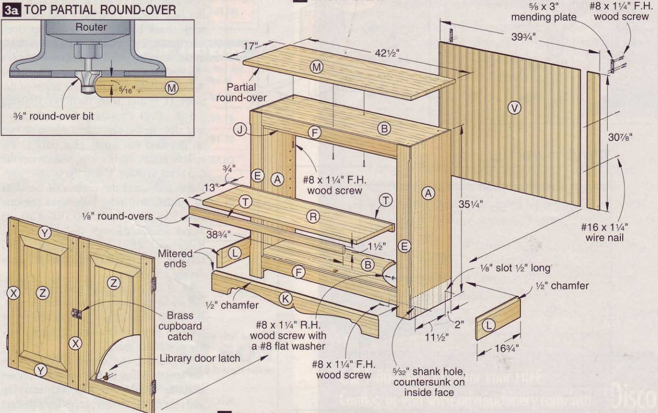
3 BASE CABINET EXPLODED VIEW
