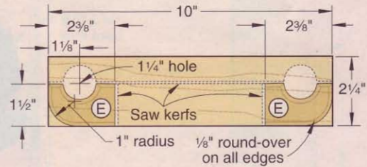
6a HANGER CLEAT
