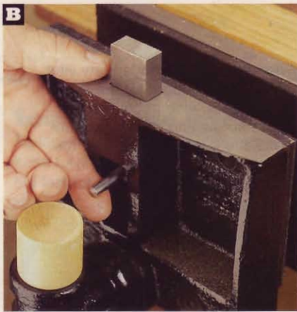
B Jorgensen's pop-up dog rises to the occasion with a simple lift lever. Spring steel in the jaw eliminates the need for a locking thumbscrew.
