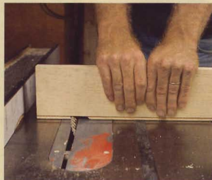
Step 4: With the stile against the fence, miter-cut the stile's bead, removing the remaining waste with repeated passes.
