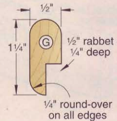
6a HANGER CLEAT
