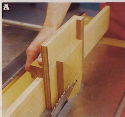
A A bevel jig that runs on an auxiliary fence makes beveling the cap tops safe and accurate.
