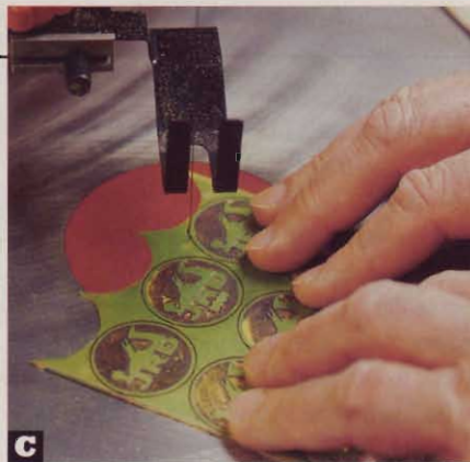
C With a very fine jeweler's blade in our scrollsaw, and good lighting, we were able to cut out our round nameplates smoothly and accurately.
