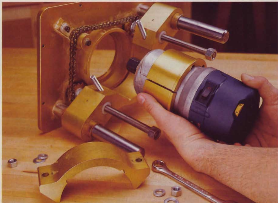
Adapter collars make midsize routers fit the ProLift Ni28, Mast-R-Lift, and Precision Router Lift (PRL), shown above . The ProLift AI13 fits these routers out of the box.
