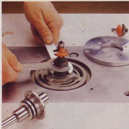
Cranking the BenchDog ProLift Ni28 to full height makes bit changing easy from above the table.
