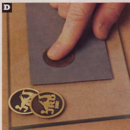
D Tape 600-grit wet/dry sandpaper onto the piece of glass used earlier. A rolled-up piece of tape on the back of the nameplate keeps your finger from slipping.
