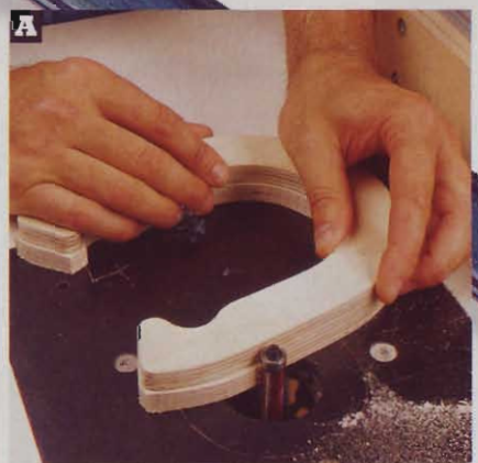
Rout the rough-cut horseshoes to shape using a flush-trim bit and template horseshoe. Take it slow, and keep a firm grip as you rout around the ends.
