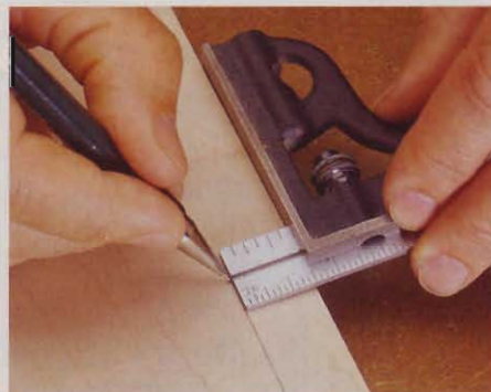
For a line parallel to an edge, place the pencil at the correct spot, then adjust your combination square to match. Put the grooved side up, so the pencil won't slip into the notch. Hold the pencil against the square as you slide it along the edge.
