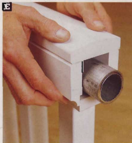
The hollow space formed by the railing cap and upper baluster stringer houses a length of 1\frac{1}{2} " galvanized steel pipe.
