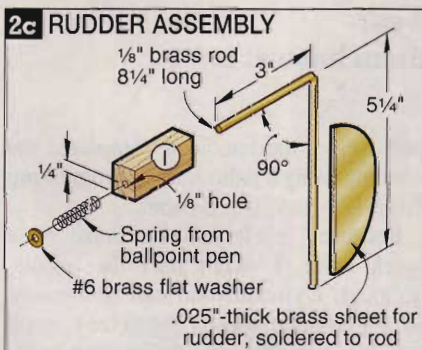
A pair of clothespins holds the rudder centered on the shaft while you solder it in place.
