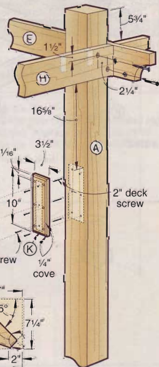
4 BRACKET MOUNTING
