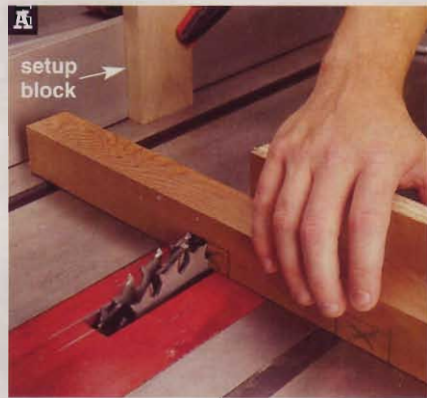
Butt the workpiece against the setup block, holding it securely against the miter gauge. Then make the first cut.
