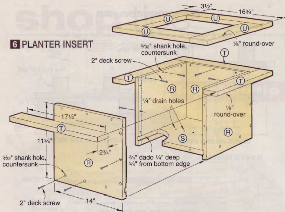
The planter inserts in the top of each column lift out for easy maintenance.
