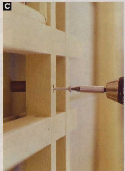
Attach all four mounting screws loosely at first, then snug them down to hold the trellis firmly to the wall.
