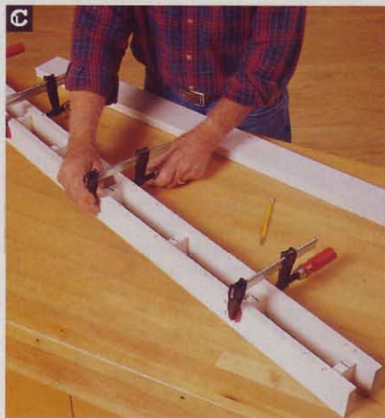
Clamp 2x2" scrap blocks between the upper rail sides (J) to keep them properly spaced and parallel.
