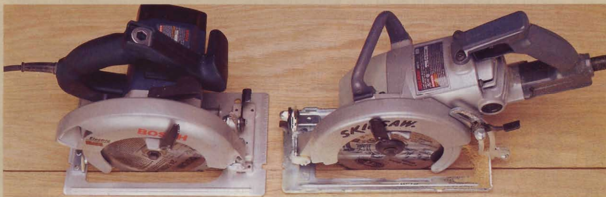
With its motor shaft perpendicular to the blade arbor, rather than parallel to it, a worm-drive saw ( right ) is longer and narrower than a helical-gear saw ( left ).
