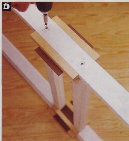
Use the spacing jigs to maintain 4" spaces between balusters and keep them centered on the stringers.
