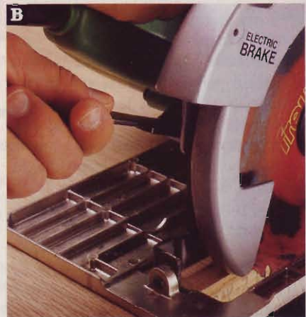
Depth-locking levers located between the handle and blade guard are awkward to operate with the left hand while holding the saw in your right.
