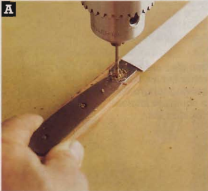
A Predrilled holes in the tang guide the drill bit to create holes for pins that, along with epoxy, attach the scales in place.
