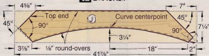
4a BRACKET
