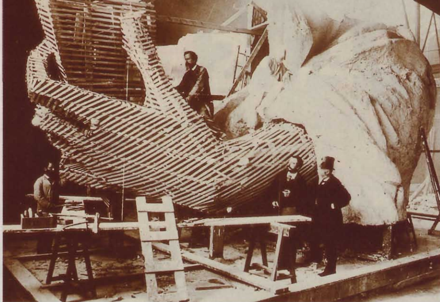
Before the final wooden molds could be constructed, it was necessary to make actual-size replicas of the statue's components out of wood lath and plaster.
