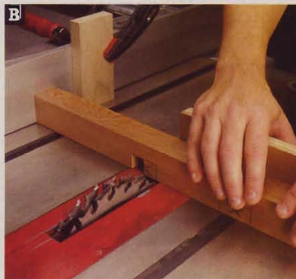
For the second pass, butt the workpiece against the fence. This doubles the dado width without a setup change.
