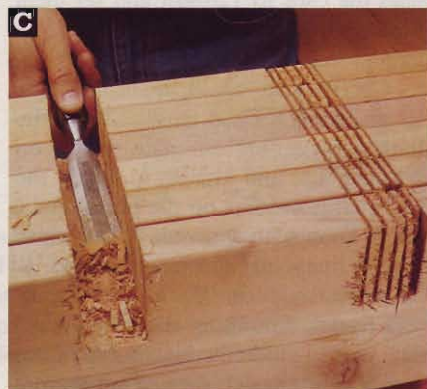
Use a chisel and hammer to clean out the notches, smoothing their bottoms to a uniform depth.
