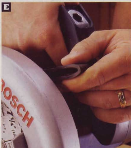
E This lever retracts the lower blade guard of the Bosch 1657 so you don't have to reach down around the blade when making pocket cuts.
