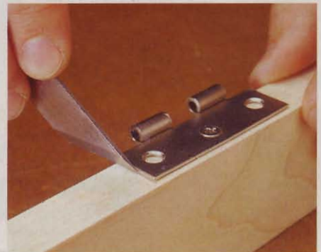
Use a knife that's flat on one side and beveled on the other to define a recessed area, such as a hinge mortise. The line will guide your chisel. This marking knife, item number 127680 in the Woodcraft catalog, costs $11.99. Call 800/225-1153.
