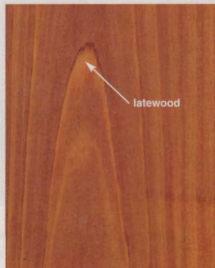
Stained with "Antique Cherry," this baldcypress board takes a lighter tone in the denser latewood. Use wood conditioner or gel stain to achieve consistent color.
