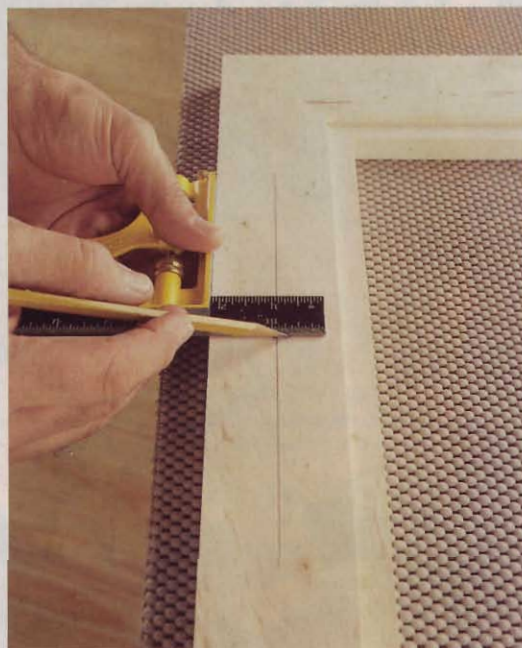
1 Mark the slot Locate the keyhole slot by drawing a long center-line on your workpiece. Measure and mark the bottom end of the keyhole slot, as shown, with a short perpendicular line.
