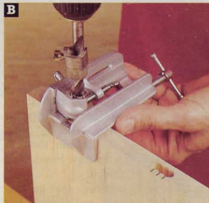
When drilling the mortises, use a doweling jig to keep your drill bit centered and vertical. The bit stop controls the depth as shown here with bottom shelf (G).
