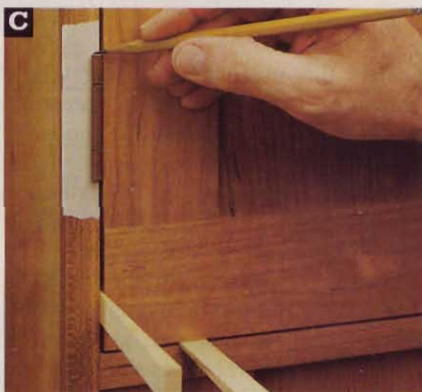
C Using wedges to hold the doors in place, mark the hinge locations on masking tape adhered to the carcass.
