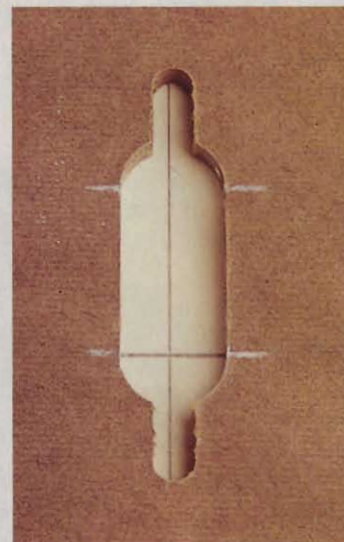
2 Index the template Align the short line with the slot-index marks on the template, and center the long line in the dust-relief slots. Clamp the template to the workpiece, and set your plunge router's depth stop so the bit will leave a 1/8-3/16"-thick shoulder above the keyhole slot.
