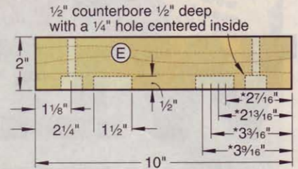
1f BOTTOM SIDE RAIL DETAIL
