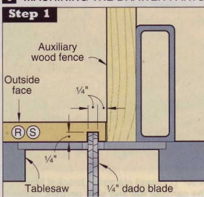
To make the drawer-side half of the lock-rabbit joint, cut dados across the drawer sides' ends.
