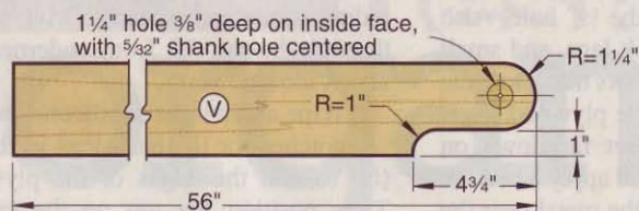
5a FRONT/BACK TRIM DETAIL
