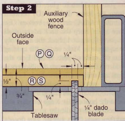
Without moving the blade or fence, cut the drawer-bottom grooves in the fronts and sides.
