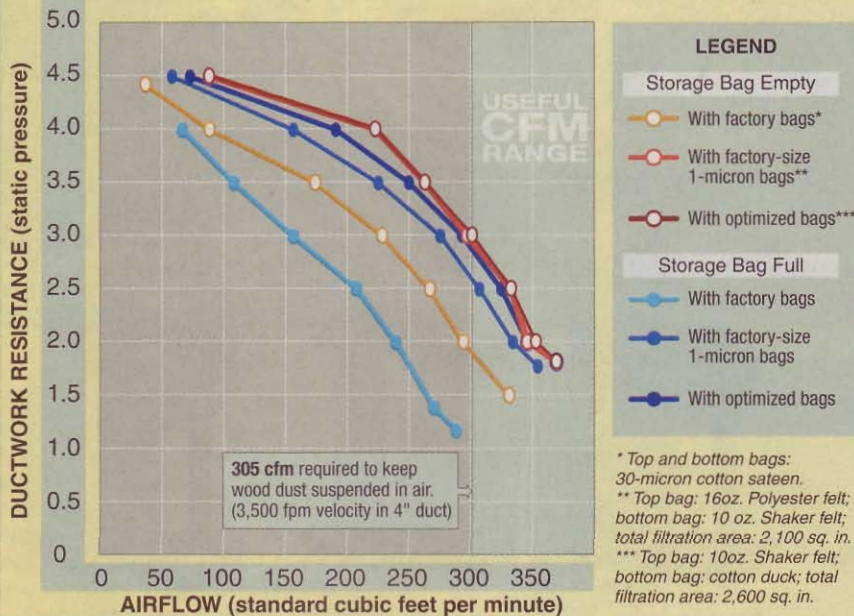
The optimized bag set for the Grizzly G8027 performed better—even with the storage bag full—than the factory bags did when empty.
