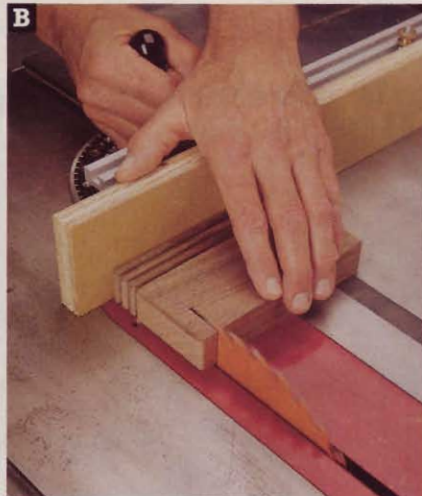
B An extension attached to your miter gauge eliminates chip-out when cutting the sides (B) from the glued-up blank.
