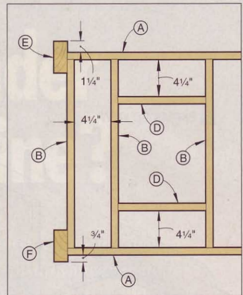
1a CARCASE DETAIL TOP VIEW
