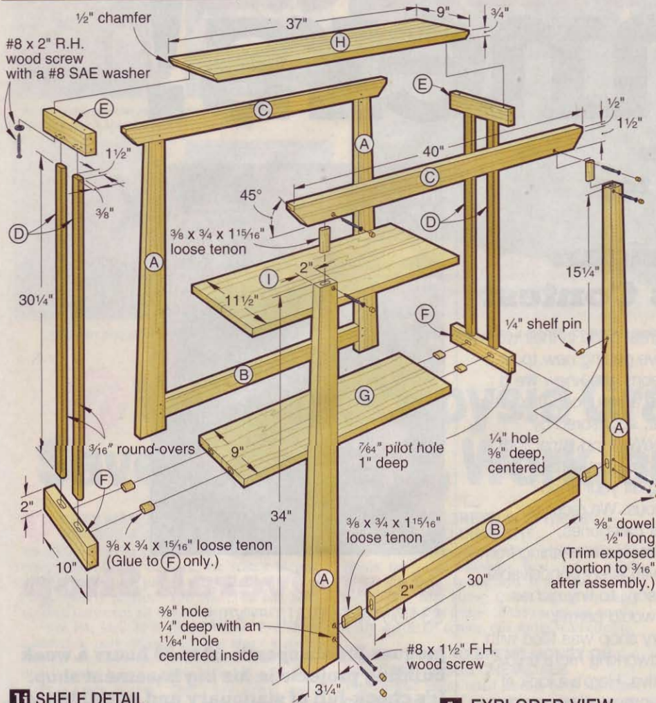
1 EXPLODED VIEW
