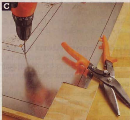
Support the metal top on a sheet of scrap plywood as you drill the holes at the corners of the rectangles.
