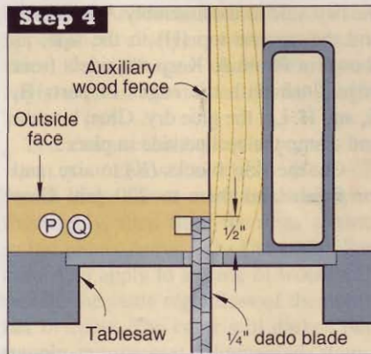
Reposition the fence, and finish the joint by cutting away part of the groove's inside lip.
