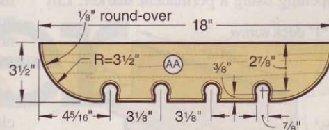
5b TOOL-RACK DETAIL
