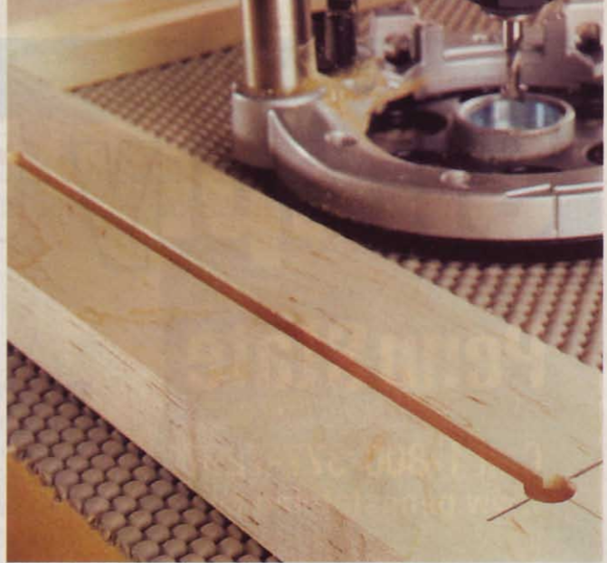
Our simple router template helps you make long keyhole slots, such as the slot shown above, or short slots, as shown below.
