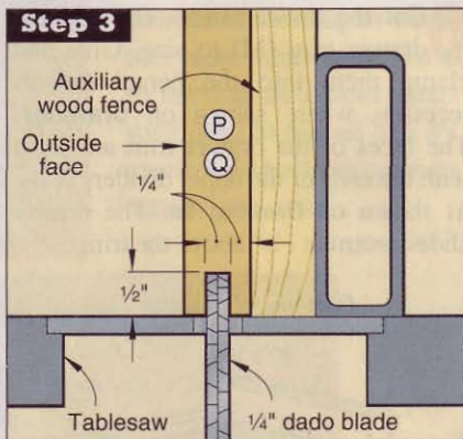
To make the drawer-front half of the joint, raise the dado blade and cut grooves in the fronts' ends.
