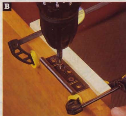
To help align them while drilling, push the no-mortise hinges, knuckle up, against a small scrap block.
