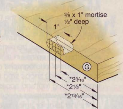
1h TOP DETAIL
