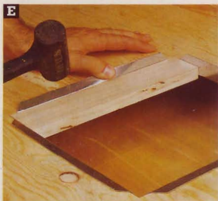
Wrap the metal around the perimeter, then form the cut-out opening. The hardwood scrap keeps the metal from rising.
