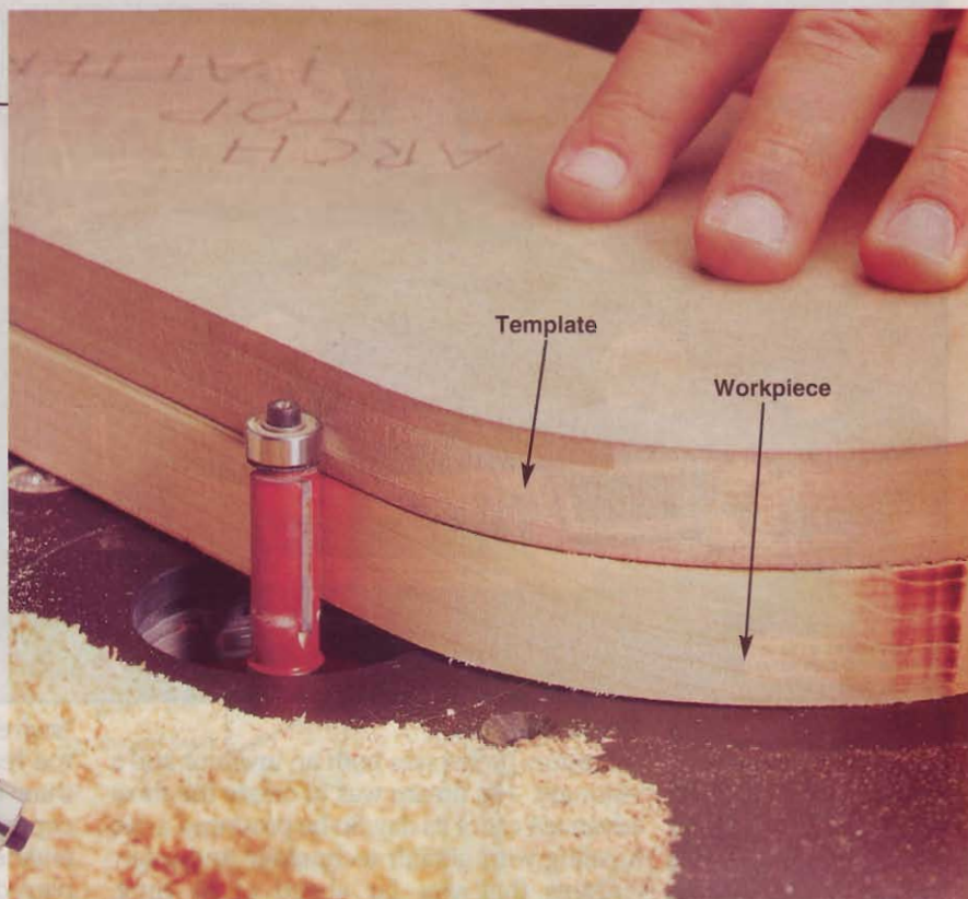
Cutting across the grain can cause the bit to become grabby and may result in burning. Bandsawing your rough workpiece close to the pattern line reduces the risk.
