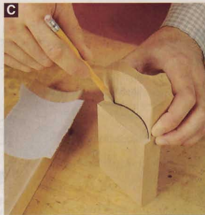
C Make a custom sanding block by tracing the cove molding's profile onto a piece of scrap and bandsawing it to shape.
