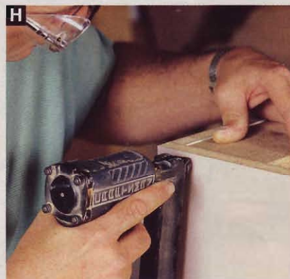
H Glue the backer boards in place, then add small fasteners to hold them while the glue dries. Use a pneumatic gun, or just tap in some brads with a hammer.
