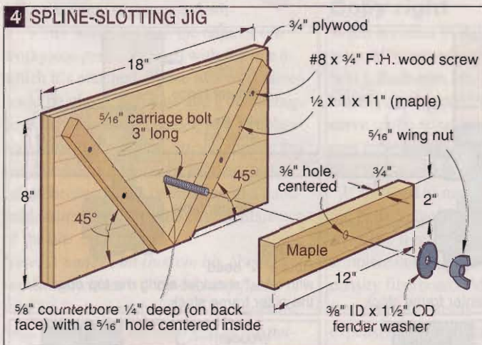
With the blade centered in the thickness of the frame, cut slots for the splines.
