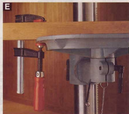
The wide rim around Delta's squarish table provides an excellent clamping surface for holding a workpiece or attaching a jig.
