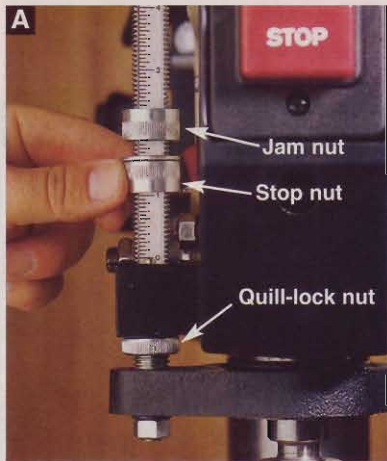
The stop nut of a three-nut system (Photo A) sets the drilling depth, the jam nut locks the stop nut in place, and the quill-lock nut fixes the quill's upward travel. Delta's stop system (Photo B) employs a quick-set stop nut and separate ratcheting-lever quill lock. In our tests, the models with dial stops on the quill-feed hub (Photo C) were easy to use but unreliable over the long haul.
