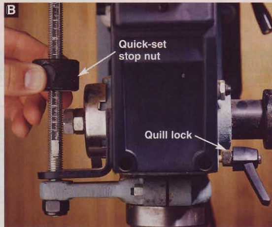
The stop nut of a three-nut system (Photo A) sets the drilling depth, the jam nut locks the stop nut in place, and the quill-lock nut fixes the quill's upward travel. Delta's stop system (Photo B) employs a quick-set stop nut and separate ratcheting-lever quill lock. In our tests, the models with dial stops on the quill-feed hub (Photo C) were easy to use but unreliable over the long haul.
