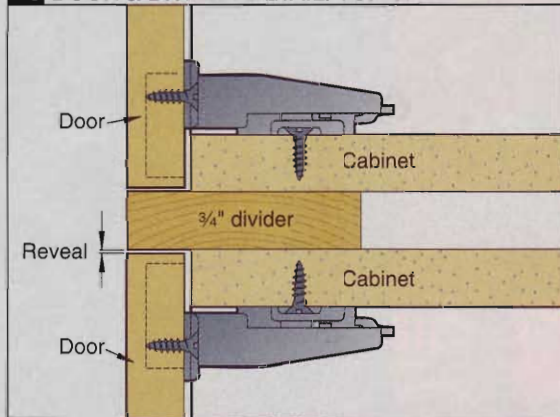
2b DOOR & DIVIDER DETAIL/TOP VIEW
