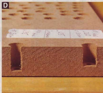
The 100th hole (left) we drilled with the Grizzly G7944 is \frac{1}{8} " deeper than the first (right). By the 25th hole, we could see the depth difference without measuring.
