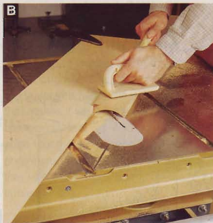
B Securely clamp an angled fence to your tablesaw to cut the cove in the molding blanks. Pushblocks are a must.
