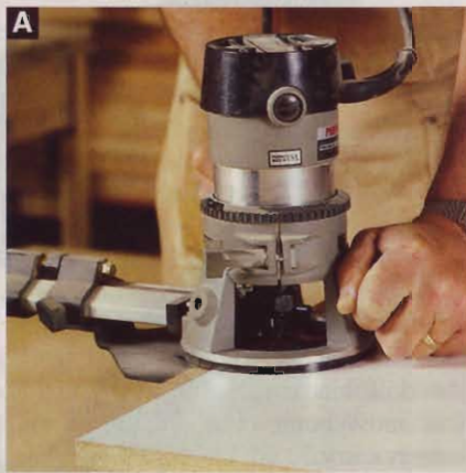
A Equip your router with a good edge guide before you start making grooves for cabinet backs. Set the guide, then do all the backs at once.
