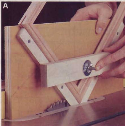
With the blade centered in the thickness of the frame, cut slots for the splines.
