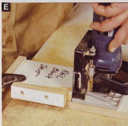
E Make a simple jig to guide your biscuit joiner for the drawer divider slots, then label it. Again, you eliminate the need for measurements.
