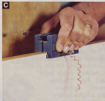
C A razor-sharp trimmer quickly cuts the lightweight veneer. This spring-loaded model handles both sides at once, and works on stock of various thicknesses.
