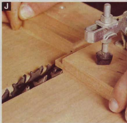
J This shopmade tenoning jig features a hold-down toggle clamp. Make your own carriage-style jig, or use a miter gauge.
