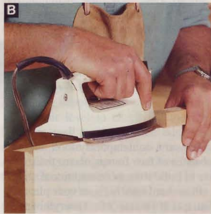
B All you need to apply veneer is an inexpensive household iron. If you plan to do a lot of cabinet work, you can buy veneer tape in 250' rolls.
