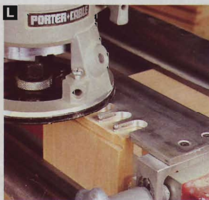
L Buy an affordable dovetail jig, practice with it, and you'll be able to make the drawer joints quickly.
