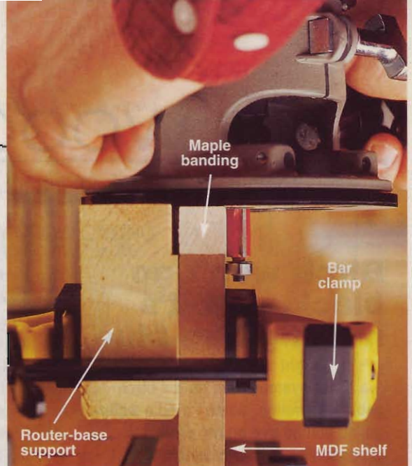
Cut a shallow rabbet in the 2x4 support piece to relieve the banding on the untrimmed side.
