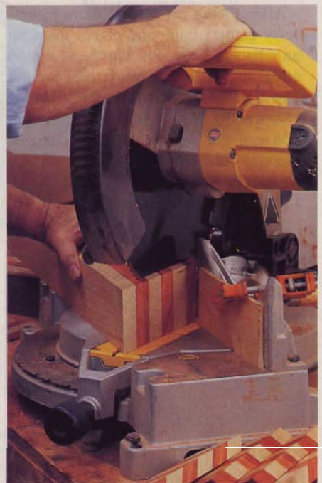
Jerry clamps a stop to his miter saw fence, then makes 45° cuts through the laminated block.
