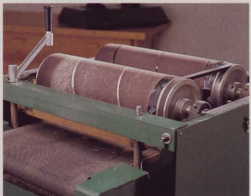
Grizzly's drum duet cuts your sanding time in half by allowing you to use different grits on each drum. Note that the height adjustment crank can be moved to another lug, such as the one in the foreground.
