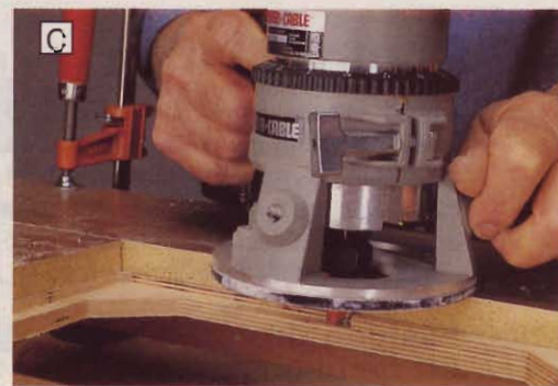
C With the bearing of the pattern bit riding on the routing guides, form the insert recess.
