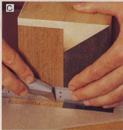
Place your metal ruler on edge against the box, and cut away the extra veneer.
