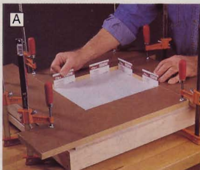
A Use business or playing cards as spacers to provide working clearance for the insert.
