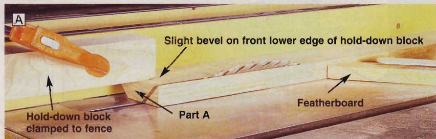
To rip the second beveled edge on the leg outer wraps (A), clamp a hold-down block in back of the blade and a featherboard in front of the blade.
