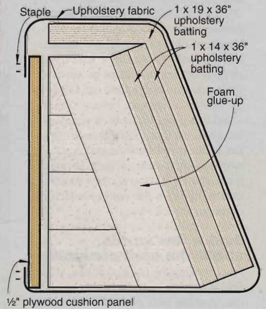
BACK-CUSHION ASSEMBLY
