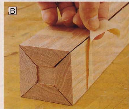
Wrap masking tape around the leg assemblies (parts A, B) to check the fit of the miters. This core is too big.
