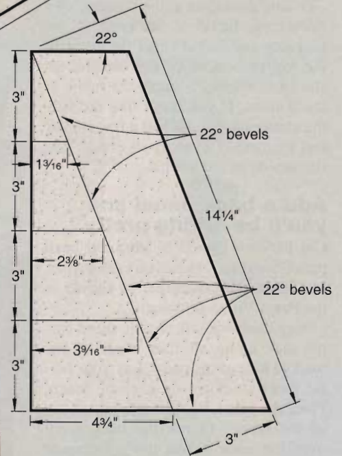
BACK-CUSHION ASSEMBLY
