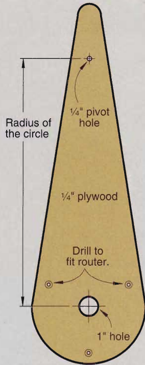
ROUTER TRAMMEL
