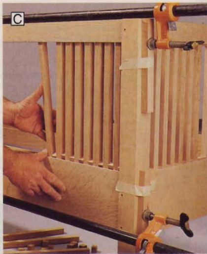
Dry-fit the back spindles and spacers, then cut the spacers at both ends to the same length.
