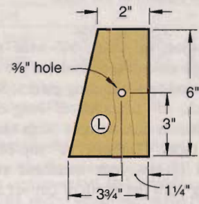
ARM BLOCK
