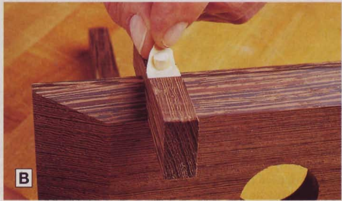
B When you remove the tape, the glue that squeezed out when you inserted the dowels comes off with it.
