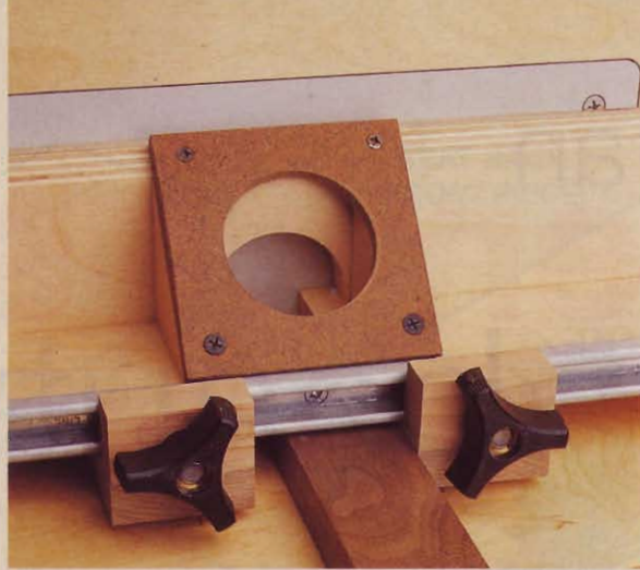
For mortising, set both stop blocks whenever possible. Guide the stock with your miter gauge.
