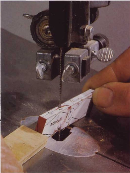
For safety's sake, use a scrap of wood to help guide the propeller cuts.
