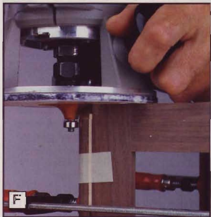
When routing the top of the upper case, \frac{1}{8} \times \frac{1}{8} " strips of wood taped into the rabbets keep the pilot bearing from dropping into them.
