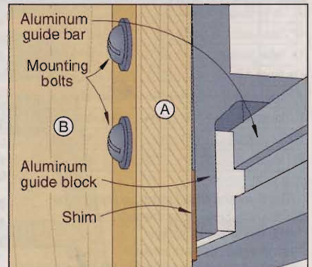
SHIMMING THE TABLE UPRIGHT
