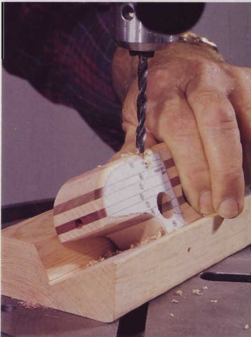
Use the drilling jig to bore the angled pontoon-strut holes (shown here) and wing-strut holes.
