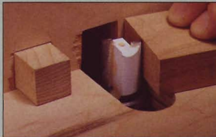
Match the height of the router bit to the thickness of a scrap piece from your panel stock, then raise the bit \frac{1}{32} ".
