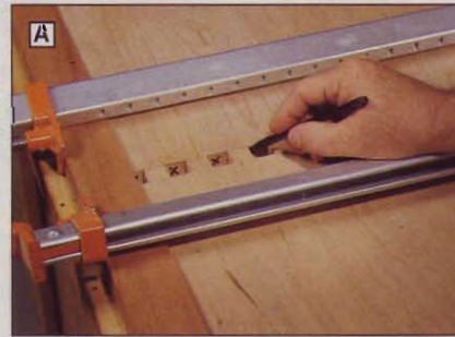
With the bottom edges aligned, mark the notch locations on the back panel.
