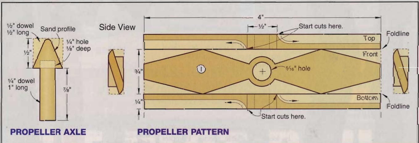
For safety's sake, use a scrap of wood to help guide the propeller cuts.
