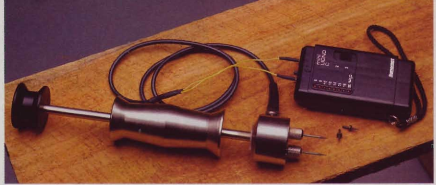
If you need to measure deep into a workpiece, consider a meter that will accept a hammer electrode for deep readings, such as the Lignomat shown.
