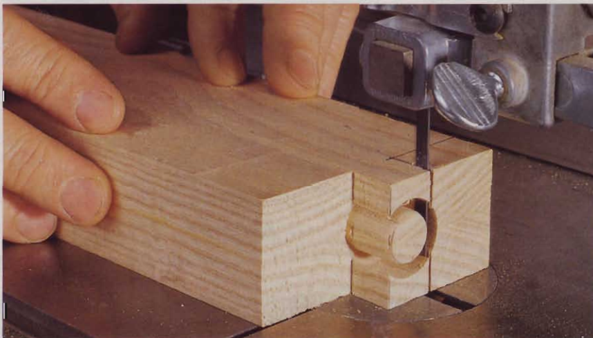
Once you've pinpointed the right location for a tenon, the drilling work goes quickly.
