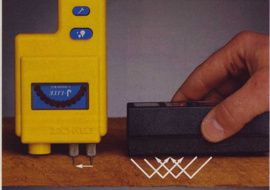
Meters with pins, such as the Delmhorst J-Lite at left, are sometimes called "resistance" meters, although they measure the wood's conductivity. Pinless meters, such as the Wagner L606 at right, are also known as electromagnetic meters because they use radio waves to measure wood moisture.
