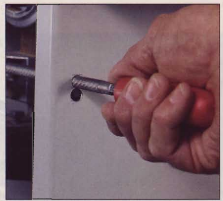
Use a rat-tail file to turn the 3/8" holes into a slot for the upper rail.
