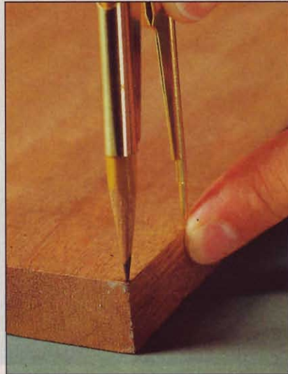
STEP 1 Hold the compass point at the edge of the stock with the pencil point at the corner. Swing an arc.
