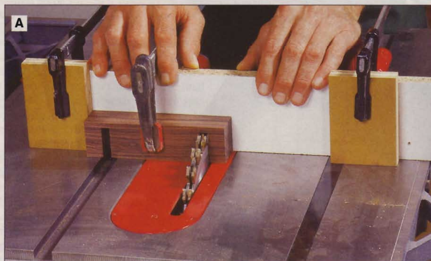
A Install an extended miter-gauge fence to saw the deep dados in the body.
