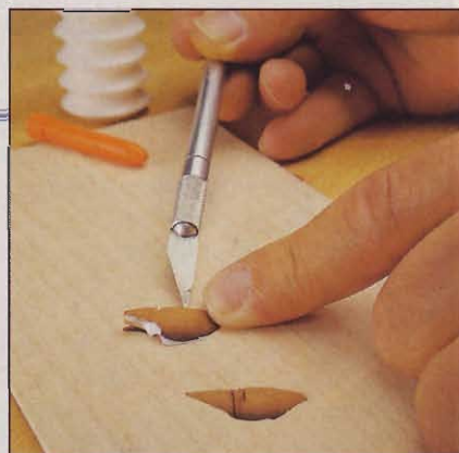
Apply glue to the edges of the inlay pieces and press them firmly into the background panel.
