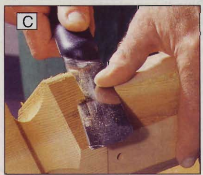
C Cut the square base of the ready-made finial to match the octagonal post. The top of the finial remains square.
