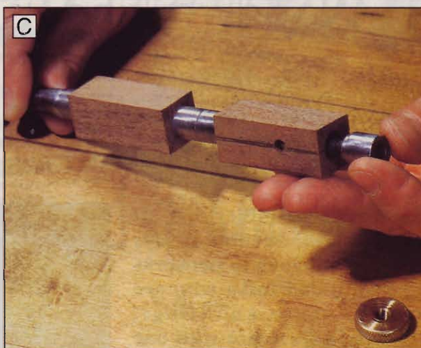
C Slide the blanks and sizing bushings onto a standard pen-turning mandrel.
