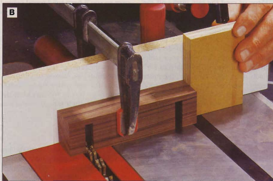
B The body dados help when setting stopblocks for sawing hinge dados in the lid.
