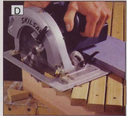
Install the base slats, then trim them to length with a portable circular saw.
