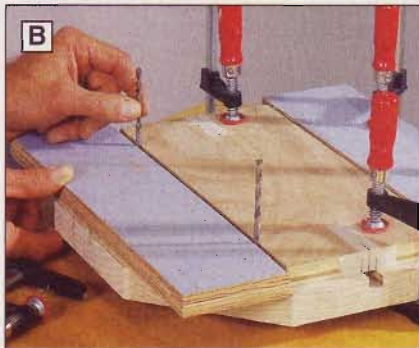
After routing the rough grooves, reinstall the setup block and the guides, now spaced \frac{3}{16} " apart. Then remove the setup block and rout the dovetail slot.
