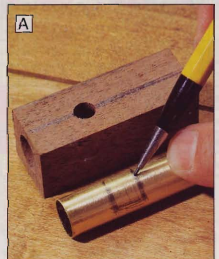
Mark the area on the brass tube that will be exposed by the hole in the top blank. Allowing a little extra is a good idea.
