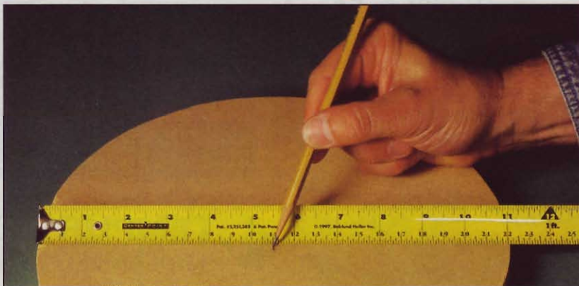
The longest measurement across a circle is the diameter. Mark the midpoint of two diameters 90° apart to locate the center.
