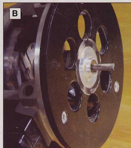
Shorten the nose of the router guide bushing to work with a thin template.
