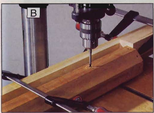
B Set a stopblock to drill holes at the same height in five faces of the post. Drill them straight with a drill press.
