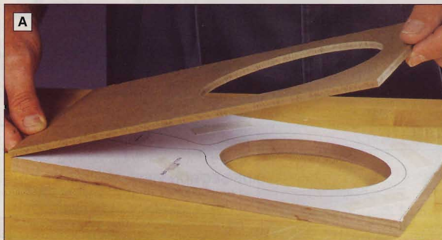
The hardboard template guides the router when forming the rabbet for the beveled mirror glass.
