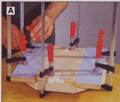
A Mark centerlines on each end of your setup block, align with the first diagonal, and clamp routing guides in place.
