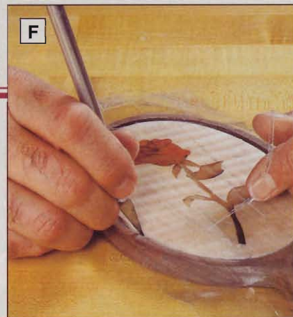
F Mask the back insert and the mirror frame with packaging tape. Apply a wide strip along the joint. Then, cut away the tape over the gap between the back insert and the frame.
