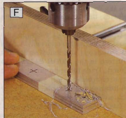
F Bundle the aluminum bars and drill the holes with a drill press for accuracy and to speed up the job.
