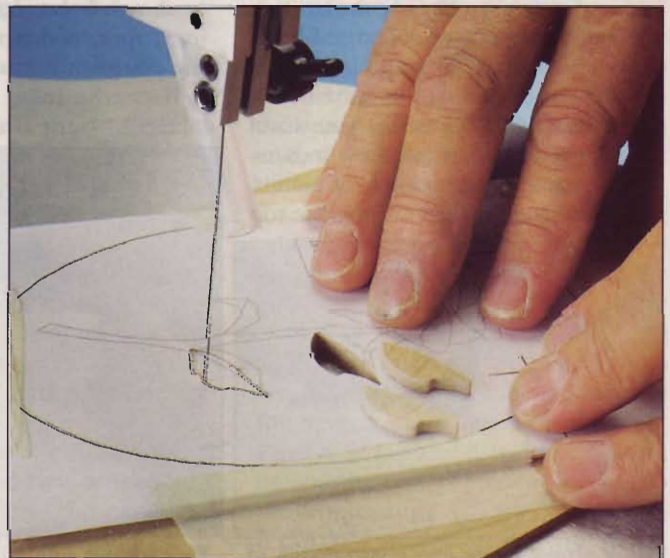
As you saw, save the inlay pieces and discard the waste pieces cut from the background panel.
