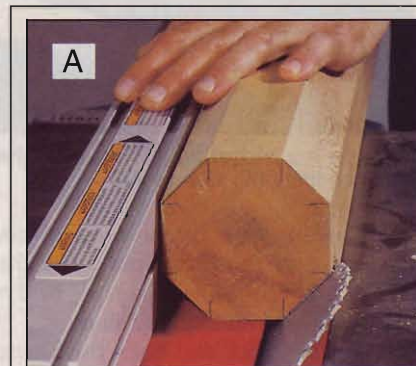
Saw the corners off a standard 4×4 cedar post to make the octagonal post (A) for the stand.
