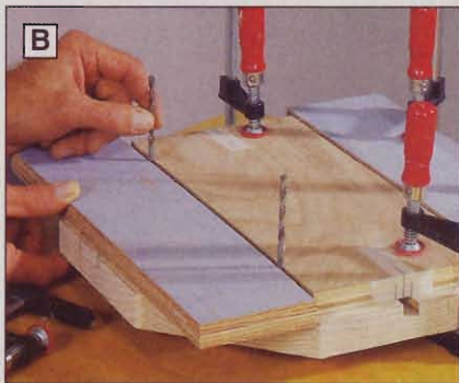
B After routing the rough grooves, reinstall the setup block and the guides, now spaced \frac{3}{16} " apart. Then remove the setup block and rout the dovetail slot.
