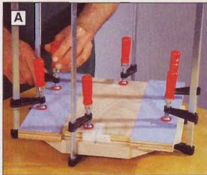
Mark centerlines on each end of your setup block, align with the first diagonal, and clamp routing guides in place.
