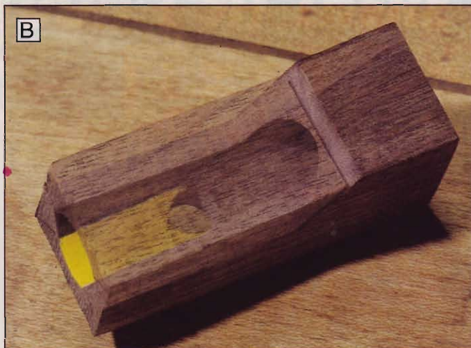
B When gluing the tube into the top blank, swab epoxy on the hole wall, except for the yellow-marked area.
