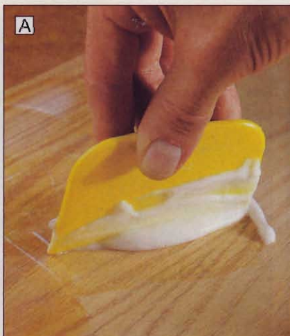
Paste wood filler, top center, makes a smooth foundation for the finish. Wet-sand with a simple solution of liquid detergent and water, left, using a rubber sanding block, bottom center. Polish with an automotive wax, bottom right.
