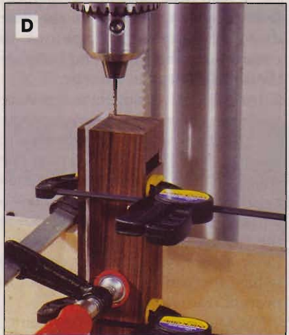
D Insert a cardboard spacer between the body and lid when drilling hinge holes.
