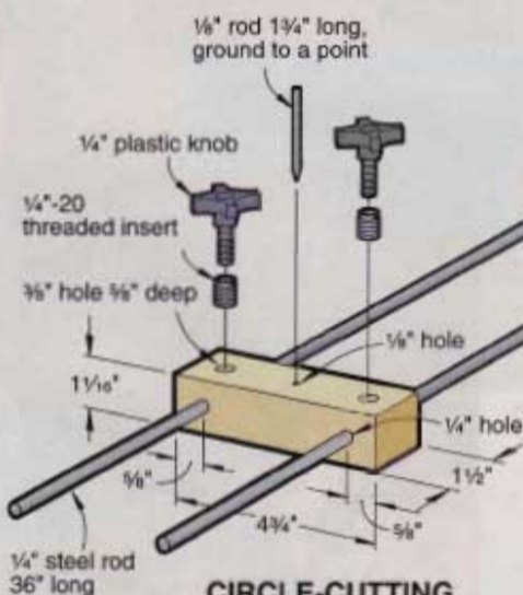
CIRCLE-CUTTING TRAMMEL
