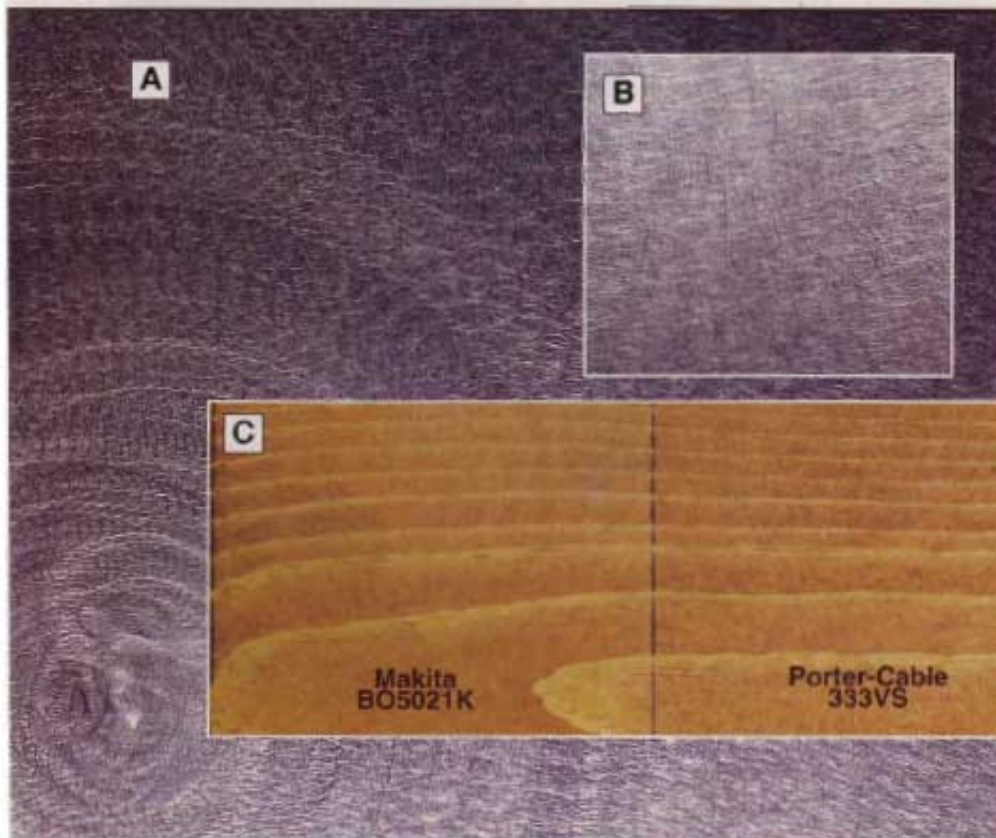
A. Less-expensive sanders leave more-detectable scratches like these left by the Black & Decker RO100 in acrylic.
