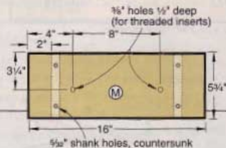
BENCH-MOUNT PARTS VIEW
