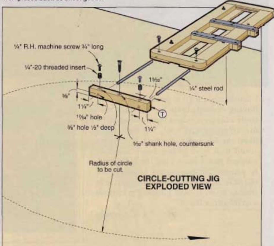
With this special circle-jig attachment, you can rout arcs and circles in large workpieces such as sheet goods.
