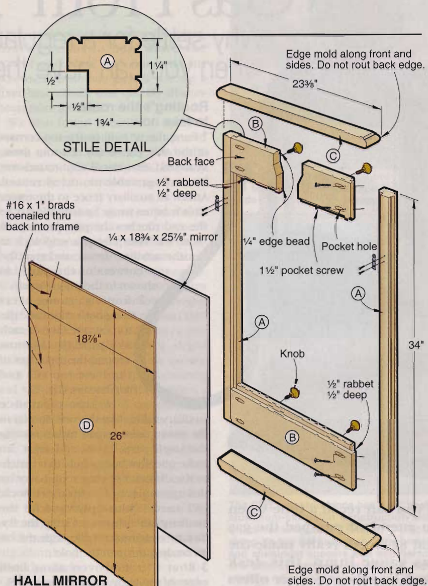
HALL MIRROR EXPLODED VIEW (shown from back)
