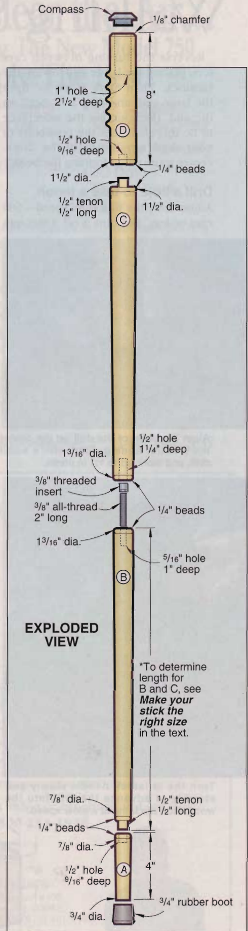
The shaft sections may prove too long to drill on some lathes. Set up the lathe to check before starting.
