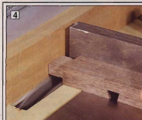
4 Fit an auxiliary fence to your tablesaw and use a \frac{3}{4} " dado blade to cut the tenons on the base rails.
