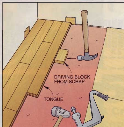
FIGURE 2 To keep the courses parallel, tap boards together before nailing.
