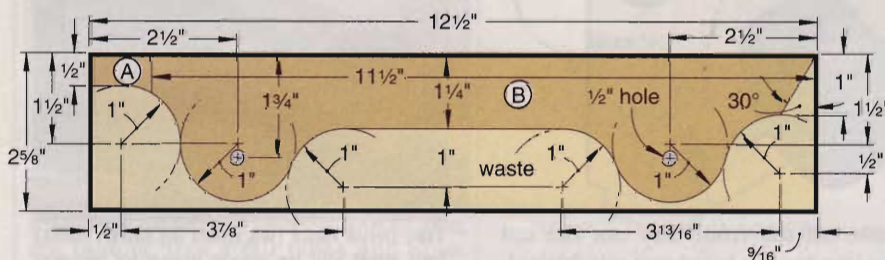
PARTS VIEW
