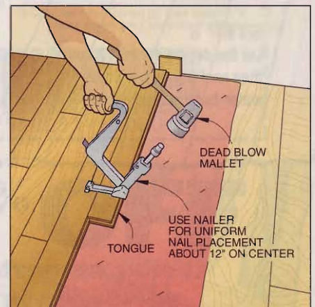
FIGURE 3 A power nailer drives and sets each nail with two blows from a heavy mallet.
