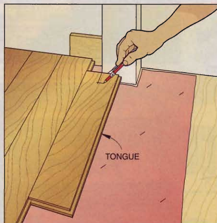
FIGURE 5 Use a compass to scribe cutouts for casings and other irregularities.
