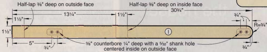
STAND UPRIGHT
