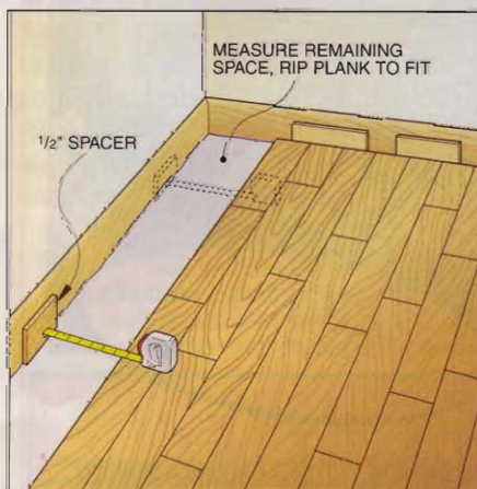
FIGURE 4 Measure for the first and last planks at several points, and rip them to fit.
