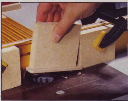
Attach a scrapwood handle to the side panel with double-faced tape when routing the slot.
