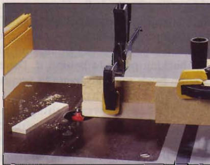
An auxiliary fence on the miter gauge supports the side panels to prevent tear-out when routing radii on the corners.
