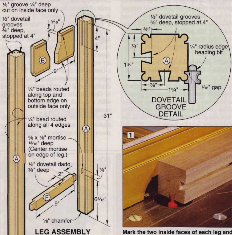
1 Mark the two inside faces of each leg and rout 4"-long dovetail slots at the top. A stopblock limits the workpiece travel.
