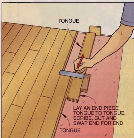
FIGURE 4 You'll need to cut the last board in each course. Here's an easy way to measure.
