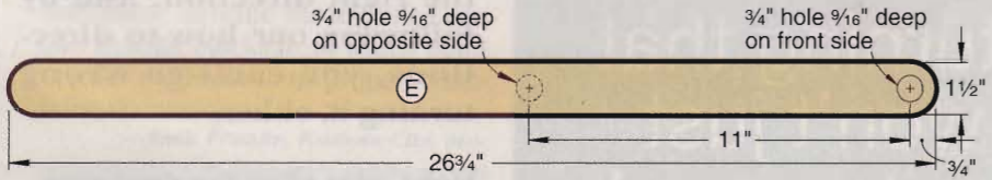
FRONT LEG
