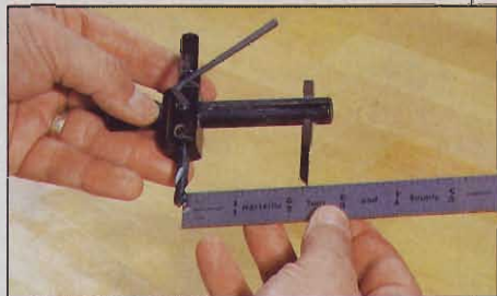
You can set the circle cutter to make any size hole. Measure the radius of the hole (half the diameter) from the center of the pilot bit to the outside of the blade.
