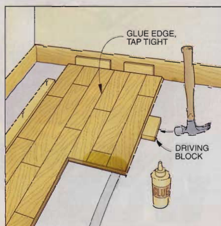
FIGURE 3 Apply a thin bead of glue along the groove in the second plank, and tap it in place.
