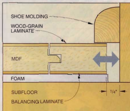
FIGURE 1 Laminate, which is more stable than wood, requires 1/4-inch spacing around the edges.
