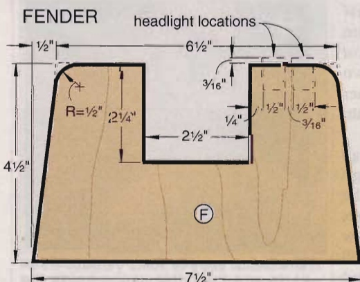
PARTS VIEW
