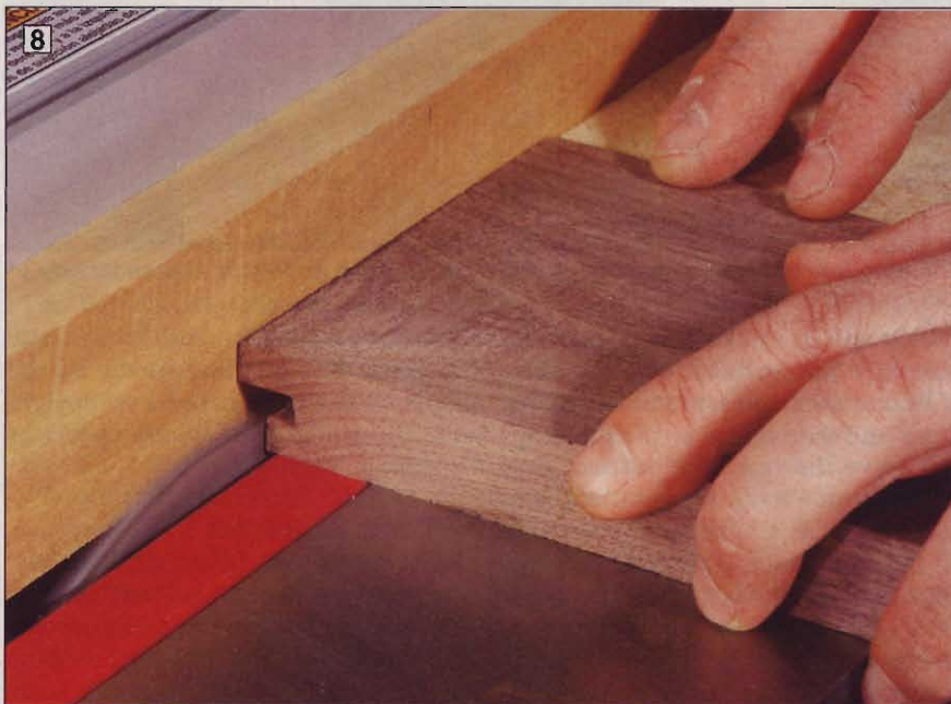
After cutting a centered groove in the end of the drawer front, trim half of the rear tongue to make a locking joint.
