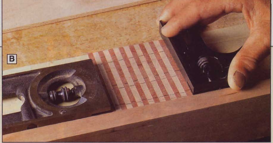
B Use a square (left) to be certain that your first segment goes onto the masking tape straight, then dry-fit the segments together. Recheck with a try-square periodically.
