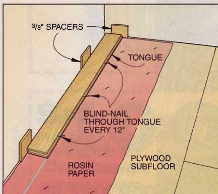
FIGURE 1 Leave a 3/8-inch gap between the flooring and walls. Molding will cover the gap.
