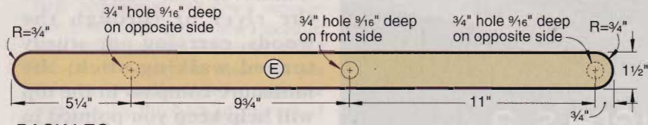
BACK LEG
