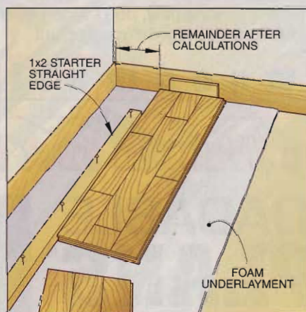
FIGURE 2 After you've figured out a starting line, nail a straightedge to secure the first plank.
