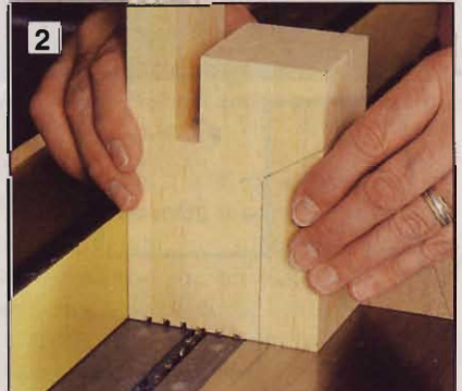
The fence gauges the position of the kerfs and the miter gauge holds the blank square when cutting the grille.
