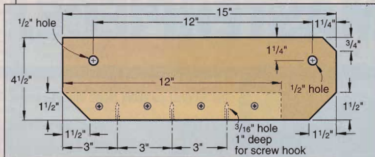
LUMBER / CLAMP RACK
