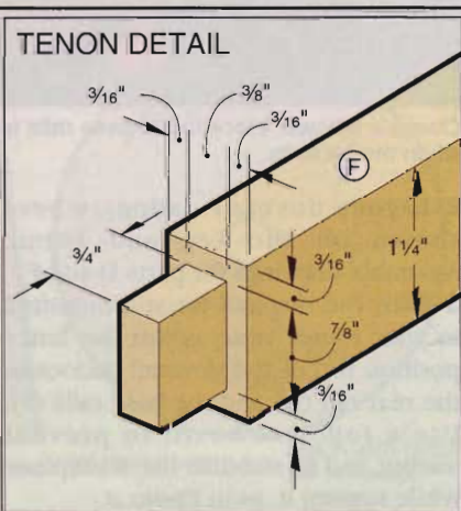
4 Fit an auxiliary fence to your tablesaw and use a \frac{3}{4} " dado blade to cut the tenons on the base rails.
