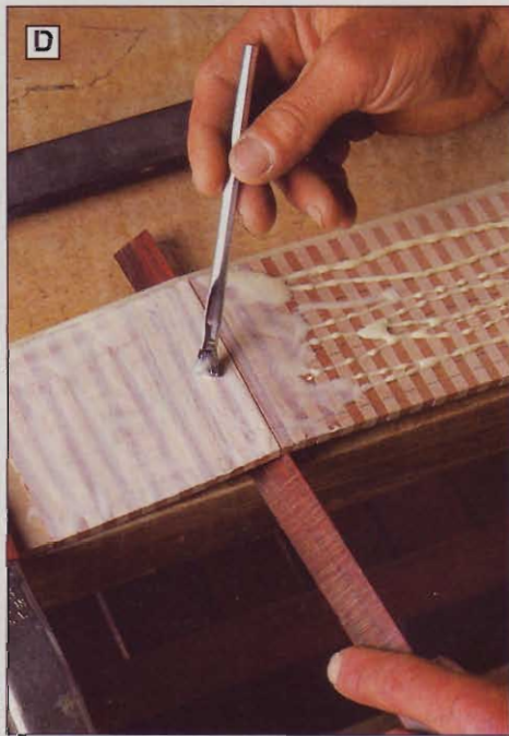
D Lifting the dry-fit segments slightly with a thin stick opens the gap between them, making it easy to brush glue into the joints.
