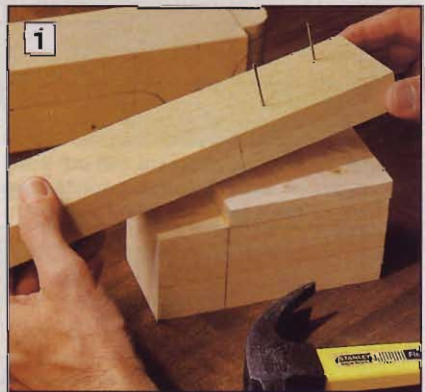
TIP: Drive nails (we used 4d finish nails) into what will be waste areas to prevent laminations from creeping when you clamp them.
