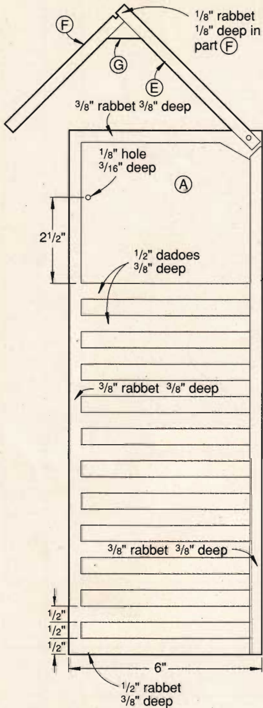
SIDE SECTION VIEW COMPUTER MEDIA BOX See page 68
