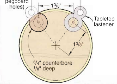
2" (distance between pegboard holes) END VIEW DETAIL
