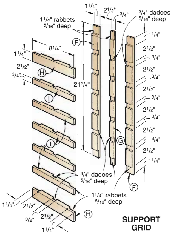
To ensure flat grids, we glued the pieces together, clamped them to flat stock, and left them there until the glue dried.
