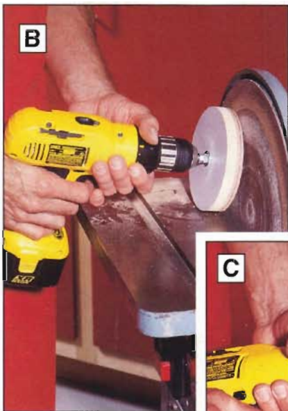
Form the beveled surface on the cap (E) by spinning the piece against a disc sander ( above ). The reference circle and edge line show the limits of the bevel ( right ).
