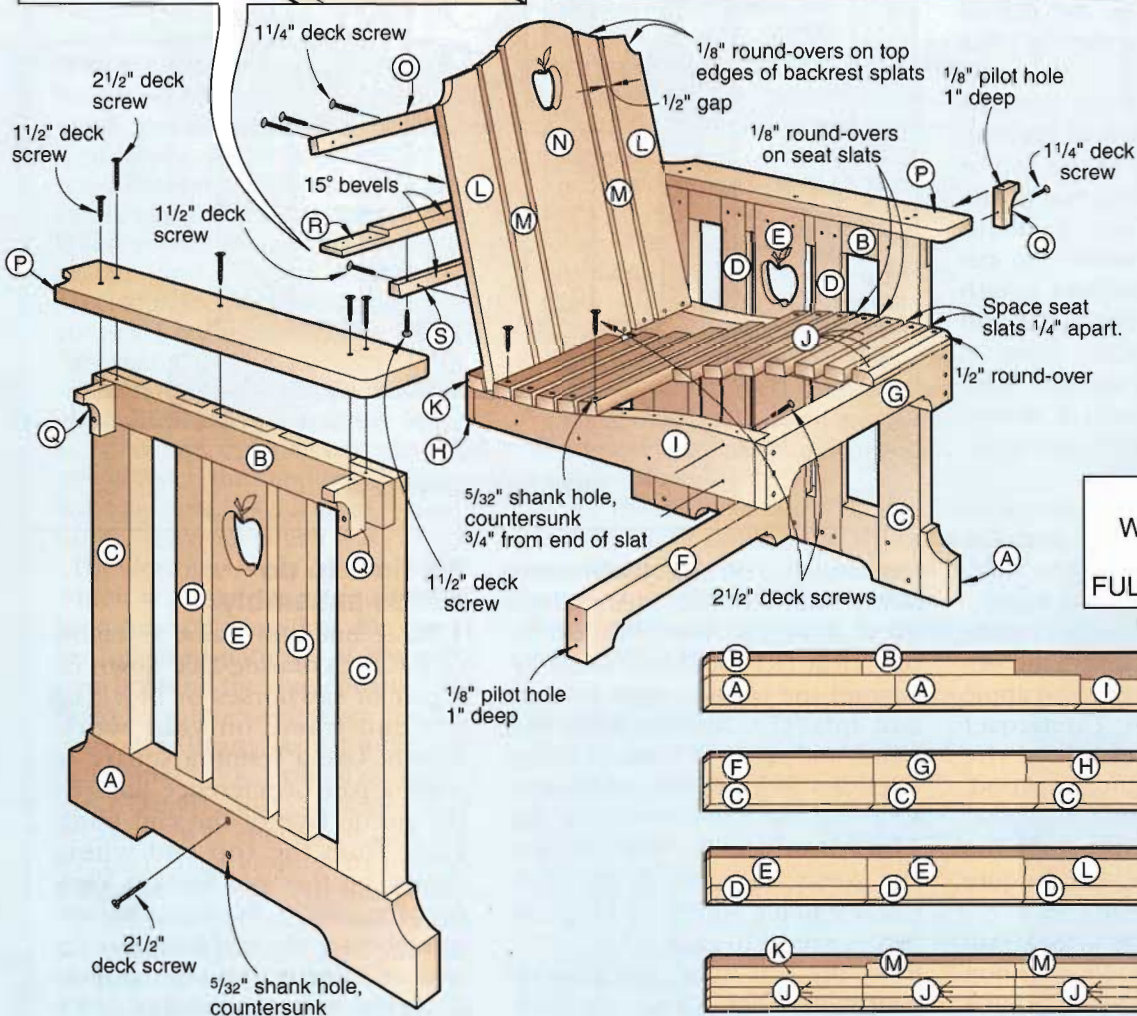
EXPLODED VIEW
