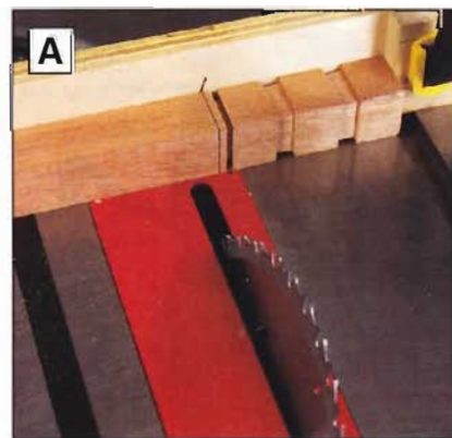
Align the saw kerf through the auxiliary miter-gauge fence with the mark on the body to saw the body bottom bevels.
