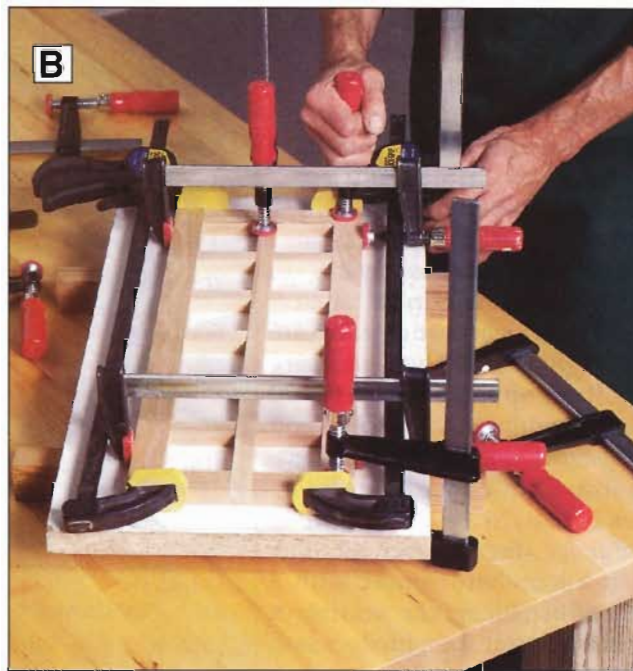
To ensure flat grids, we glued the pieces together, clamped them to flat stock, and left them there until the glue dried.
