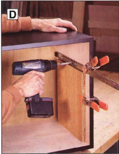
D We used a plywood spacer clamped to the inside of the drawer cabinet to level and position the drawer slides.
