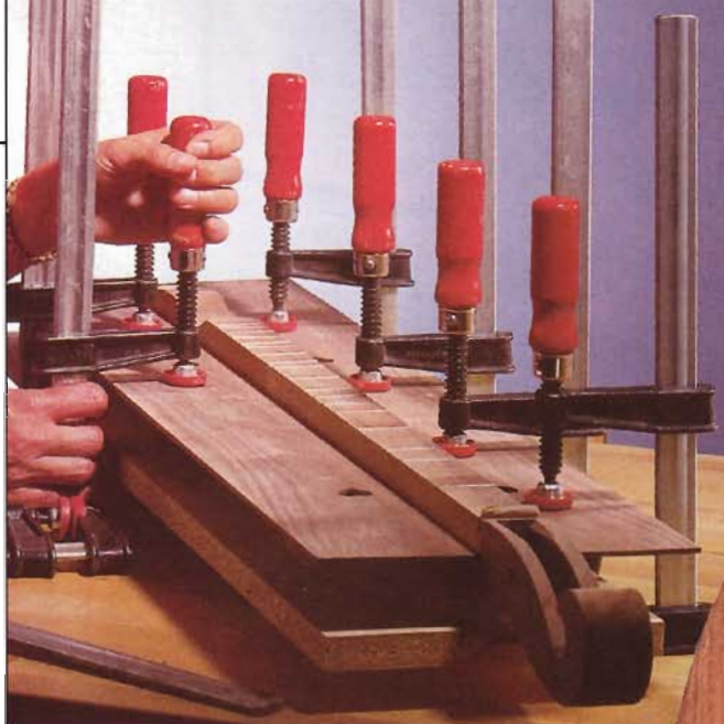
After gluing and clamping the walnut soundboard, Cheryl had to trim it to match the sides of her dulcimer.
