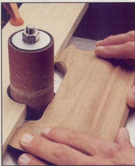
When forming the legs, use a fence with a drum or spindle sander to sand a straight edge and smooth radius.
