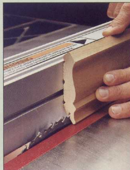
Hold the back side of the molding against your tablesaw's fence to cut the kerf that holds the panel in the center of the lid.
