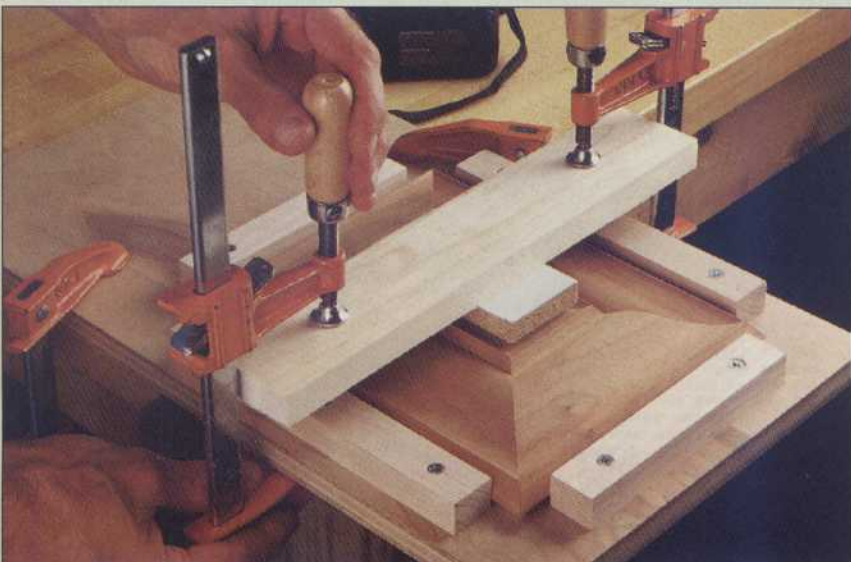
Apply glue to the mitered edges and squeeze them together with the help of some scrap stock and clamps.
