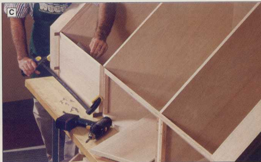
With the cabinet on its back, use spacers to create equal gaps between the molding and banded side panels.
