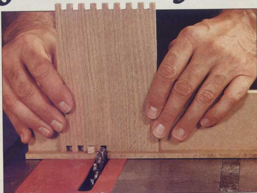
The key to this super-simple box-joint jig is setting it up precisely so the "fingers" of your box joints line up regardless if the workpiece is 3" or 13" wide.
