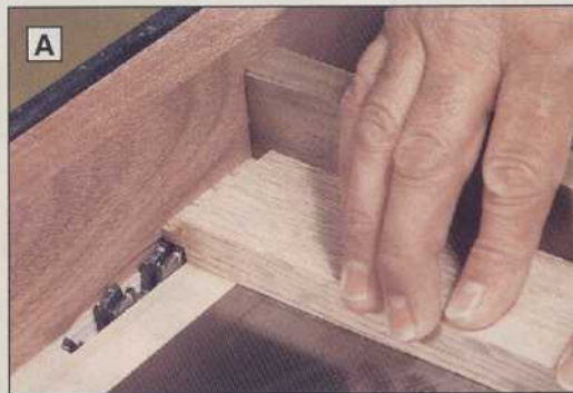
A A wood extension secured to our miter gauge minimizes chipout when cutting the rabbets to form the tenons on the ends of the rails.
