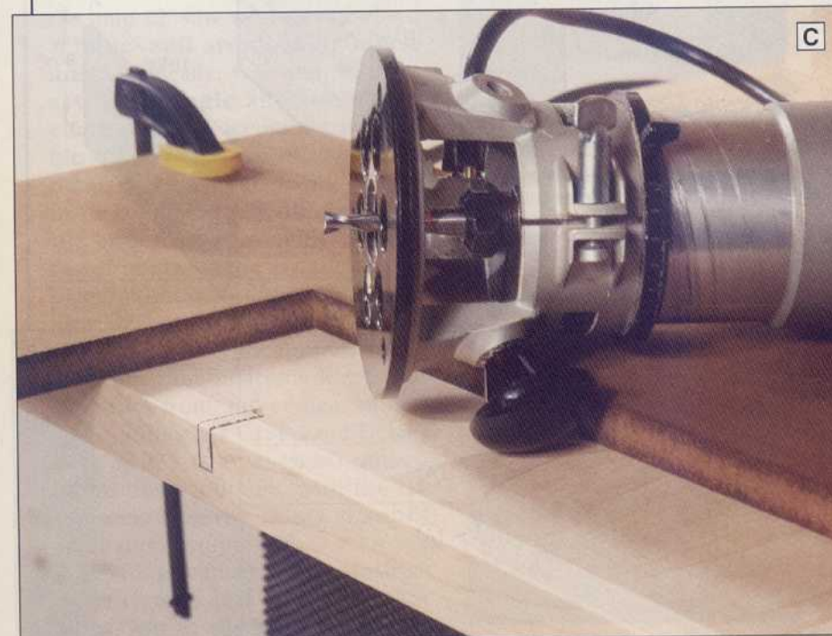
Using a \frac{3}{8} " straight bit and an L-shaped template, rout a \frac{3}{8} "-wide slot on the inside face of each side panel.
