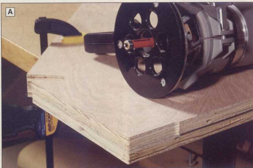
Using your first shelf as a template, rout the final shelves to finished shape with a router fitted with a piloted straight bit.
