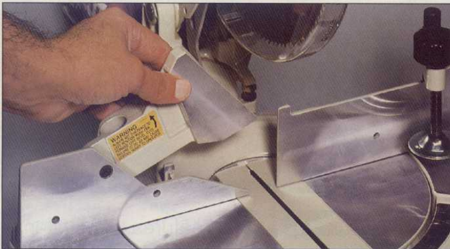
Makita's saw comes with a two-piece flip-up left fence, making it ideally suited for miter and bevel cuts. At 4 1/2", the LS1040's fence ranks as the highest in the 10" class.
