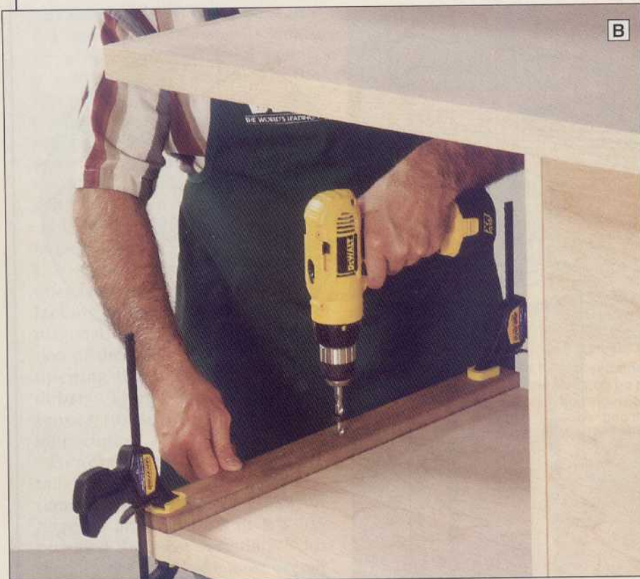
For accurately placed holes in the swivel top and inside surface of the side panels, use a hole guide to locate the holes.
