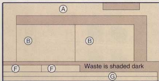
3/4 x 49 x 97" Medium density fiberboard (MDF)
