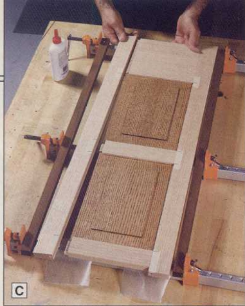
C Pencil lines on masking tape allows you to align the pieces when gluing and clamping each frame-and-panel assembly together.
