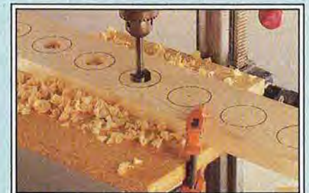
Mark the wheel centerpoints and radii, and use a 1" Forstner bit to drill holes \frac{1}{2} " deep for each wheel.
