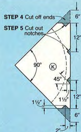
PLYWOOD SECTION (Top view)
