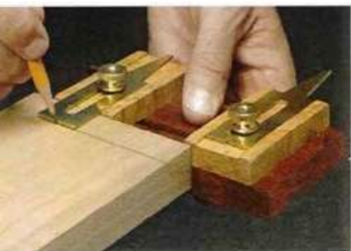
▲ Scribing Lines. A small notch in the end of each key holds your pencil tip for marking lines parallel to the edge of a workpiece.
