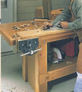
Heavy-Duty Workbench
