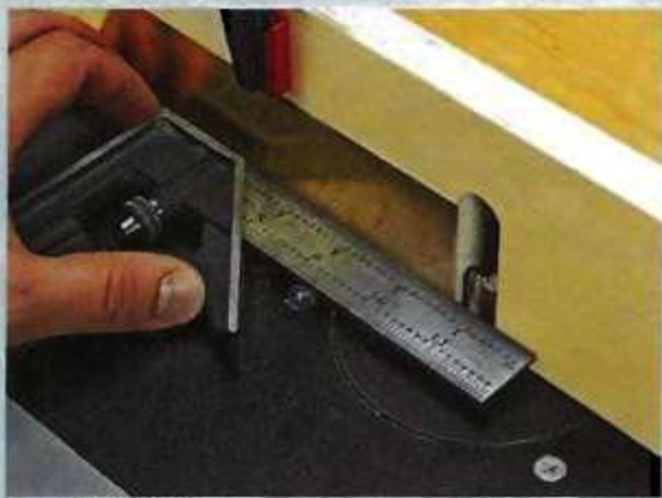
▲ Set Up the Fence. Clamp the auxiliary fence to the router table fence. Then place a combination square against the "outfeed" side. Adjust the fence until it's flush with the outside cutting edge of the bit.
