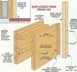
Tenon Saddle Jig. This simple jig makes cutting bridge joints or traditional tenons a breeze. The rip fence sets the jig's position to the blade.
