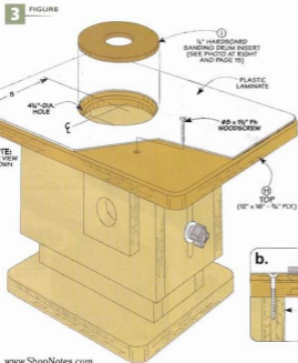
▲ Custom-Fit Inserts. To provide solid support for the workpiece and ensure good dust collection, you'll need to custom fit each insert to the table and sanding drum. To learn more about how to do this, turn to page 15.
