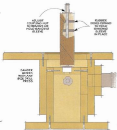
SIDE VIEW CROSS SECTION
