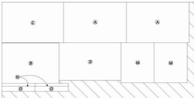
48" x 86" - \frac{3}{4} " PLYWOOD
