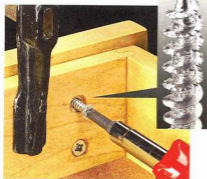
▲ Spax Screw. The unidrive head allows the screw to be driven with Phillips, Pozidrive or Robertson (square-drive) drivers. Serrated threads at the tip of the screw make them self-tapping and easy to drive.
