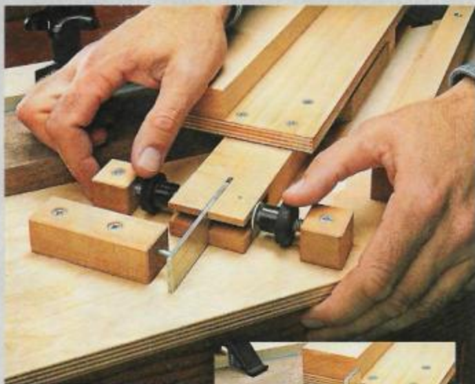
▲ Fine Tuning for a Perfect 45° Cut. With the guide assembly at 45°, set the screw until it touches the aluminum stop (see insert). Then it's easy to return to this position by just flipping the stop down and adjusting the knobs.
