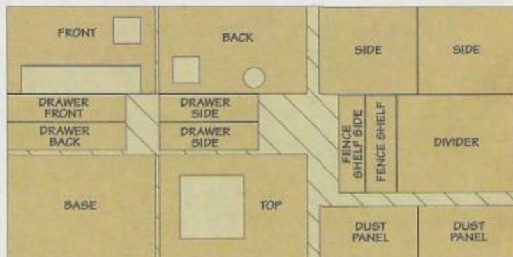
CUTTING DIAGRAM (48" x 96" - 3/4" PLYWOOD)
