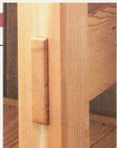
▲ Through Tenons. A few cuts on the table saw are all it takes to make perfectly sized mortises for the through tenons of the bench.
