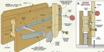
FENCE DETAIL
