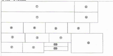
48" x 96" - 3/4" PLYWOOD
