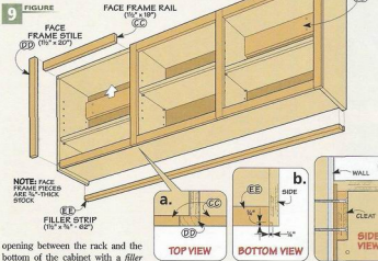
NOTE: FACE FRAME PIECES ARE \frac{1}{2} "-THICK STOCK a. TOP VIEW b. BOTTOM VIEW c. SIDE VIEW
