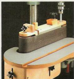
Drill Press Belt Sander page 6
