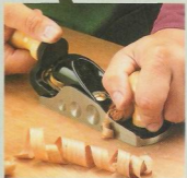
▲ Soothing Plane Kit. To turn the block plane into a versatile, low-angle smoothing plane, you can add a pair of knobs that provide a solid grip for bearing down on the workpiece.
