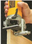
▲ Edge Guide. Most trim routers come with an edge guide accessory that makes it easy to trim edge flush without using a flush trim bit.
