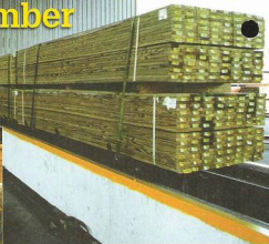
▲ Feeling the Pressure. A stack of freshly-treated lumber is rolled out from a large pressure chamber. Inside the chamber, vacuum pressure is used to impregnate the wood with a liquid chemical preservative.
