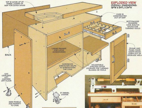
▲ Bed Extension. The lathe stand is extra-long in case you decide to expand your turning capacity by adding a bed extension to your mini-lathe.
