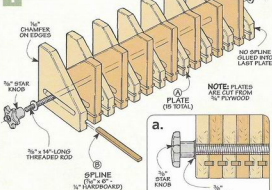
▲ V-Block. The V-block makes it easy to drill a hole in a dowel or round stock. The individual plates of the V-block can be adjusted for different diameters.
