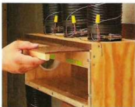
B. Dust Control Box. To direct dust and chips from the tool you're using to the dust collector, simply slide open the blast gate for that tool.
