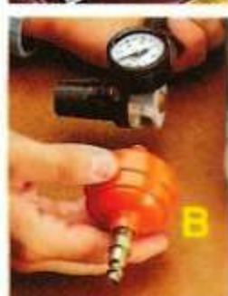
▲ Conversion Gun. With a conversion gun, air is supplied by a compressor. To avoid contaminating the finish, it's important to remove moisture from the air by installing a permanent trap (A) or disposable filter (B).
