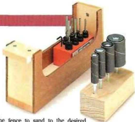
▲ One of the simplest ways to organize drill bits and accessories is to store them in wood blocks that fit inside the bins.
