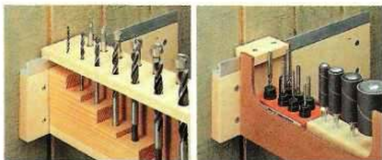
▲ Cleat. A two-part cleat that's made up of a hardwood mounting plate and a metal rail lets you hang each of the racks (left) and bins (right) on the wall. Just be sure to anchor the cleat securely to the wall.
