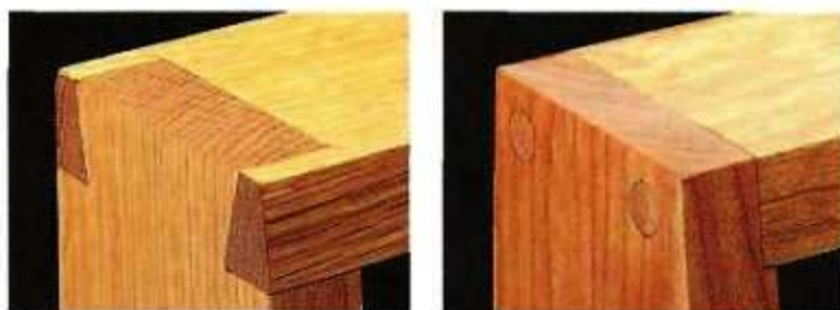
▲ Two Versions. You can use hand-cut dovetail joints (see photo at left) or rabbets, woodscrews, and plugs (right) to hold the rack together. Either way, it creates a strong, mechanical joint.
