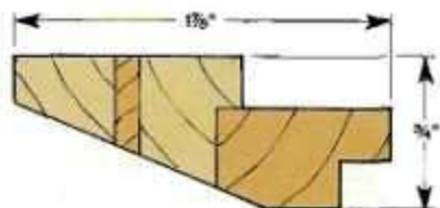
CROSS SECTION
