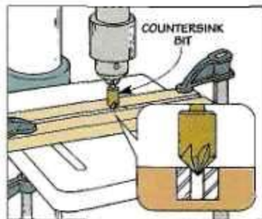
Step 3. To help center the tap, use a countersink bit to cut a slight chamfer around the rim of the hole.
