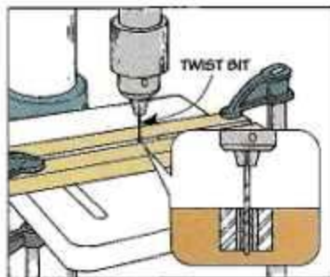
Step 2. Start by drilling a small ( \frac{3}{16} " ) hole. Then drill a series of larger holes up to \frac{1}{8} ".
