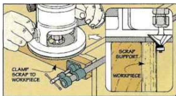
B. Scrap Support. To add extra support that keeps the router from tipping on a narrow edge, clamp a scrap board to the side of the case.
