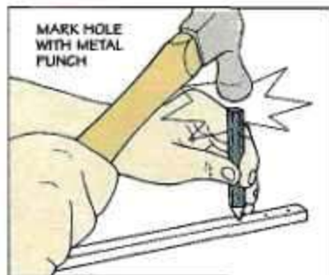
Step 1. To prevent the bit from wandering, use a metal punch to create a dimple in the bar.
