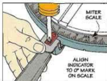
B. Align Indicator. Once you get a perfectly square test cut (see margin), align the indicator with the 0° mark on the miter scale.
