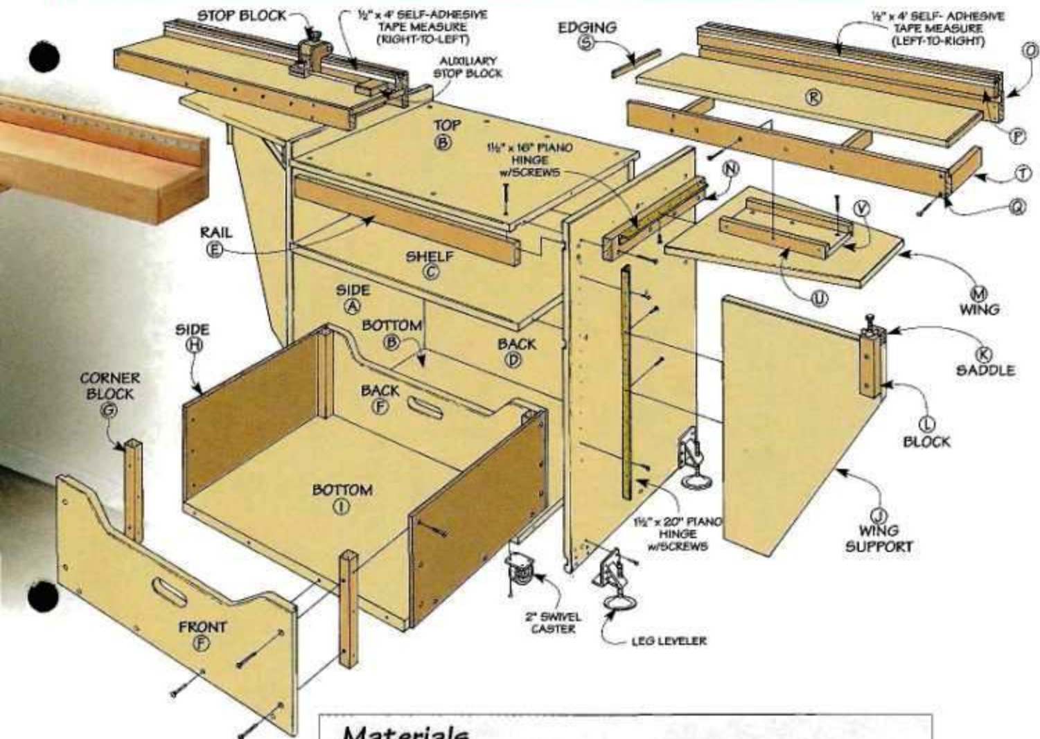
EXPLODED VIEW OVERALL DIMENSIONS: 43½" H x 96¼" W x 21" D
