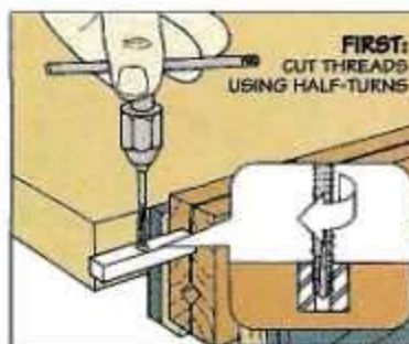
Step 5. With the tap straight up and down, begin cutting the threads (left). After each half-turn, back off the tap to clear the waste (right). Then repeat the process until the threads are cut all the way down.
