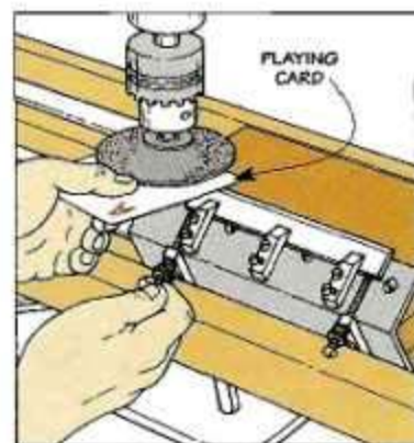
Step 4. A playing card works like a feeler gauge as you adjust the stops to position the knife.
