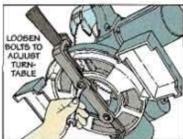
A. Adjust Turntable. After loosening two bolts on the bottom of the saw, adjust the turntable so the blade is square to the fence.
