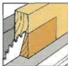
To cut the wedge, start by ripping the blank at an angle.
