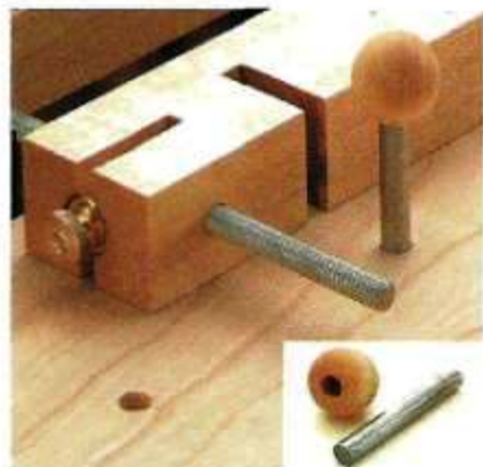
B. Index Pin. An index pin made from a cutoff bolt and a wood ball positions the drilling guide automatically.
