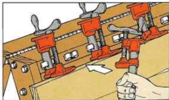
Step 4. After the last workpiece is positioned, tighten the back clamps. Then add another row of clamps across the top of the panel.
