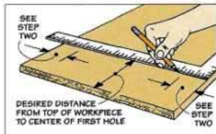
Step 1. Once you decide how far from the top (or bottom) to start the holes, square a line across the workpiece.
