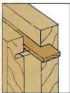
A waxed, wood "key" helps keep the T-slot aligned during glue-up.
