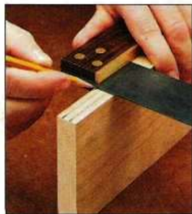
Length. Use a try square to lay out the shoulders and determine the length of the tenon.
