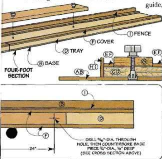
Router. With the cutting guide clamped across a wide panel, it can also be used to turn your hand-held router into a precision tool when routing dados (or grooves).
