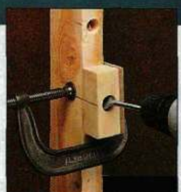
▲ When drilling an angled hole, this simple guide makes it easy to start the bit at the correct angle. Just clamp the guide in place so the angled back edge is against the stud. This raises the hole in the guide at a slight angle which helps position the drill bit.
