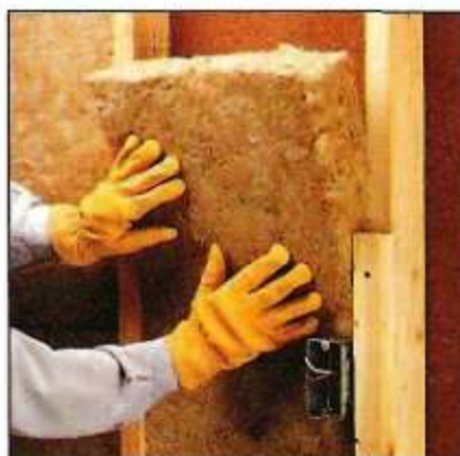
Step 2. A quick and inexpensive way to increase the STC of a wall is to tuck a sound blanket between the studs.
