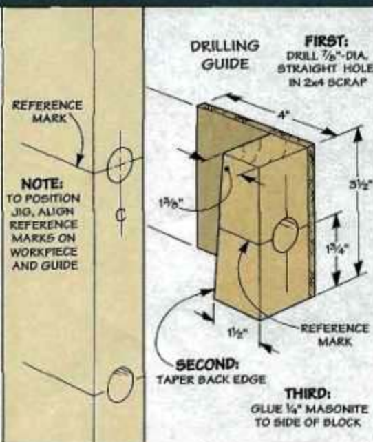
▲ When drilling an angled hole, this simple guide makes it easy to start the bit at the correct angle. Just clamp the guide in place so the angled back edge is against the stud. This raises the hole in the guide at a slight angle which helps position the drill bit.
