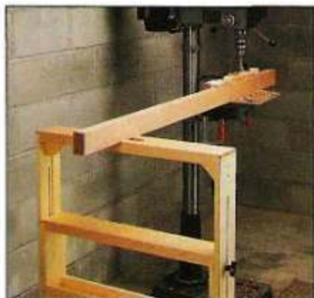
A. Work Support. This sawhorse can support a long workpiece when working at the drill press or band saw.
