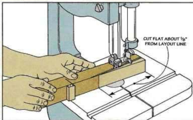
Step 4: Using a band saw (or hand saw) rough cut a flat on the leg that's about \frac{1}{8} " from the layout line. This flat creates a support that spans the throat opening of the jointer table.
