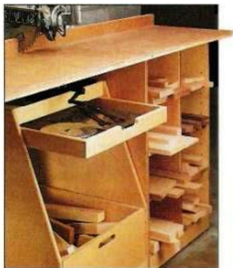
Radial Arm Saw Stand
