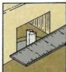
A straightedge makes it easy to set your router bit flush with the fence.
