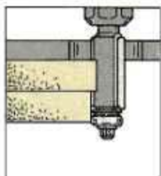
To trim the edges flush, I used a flush trim bit in a hand-held router.
