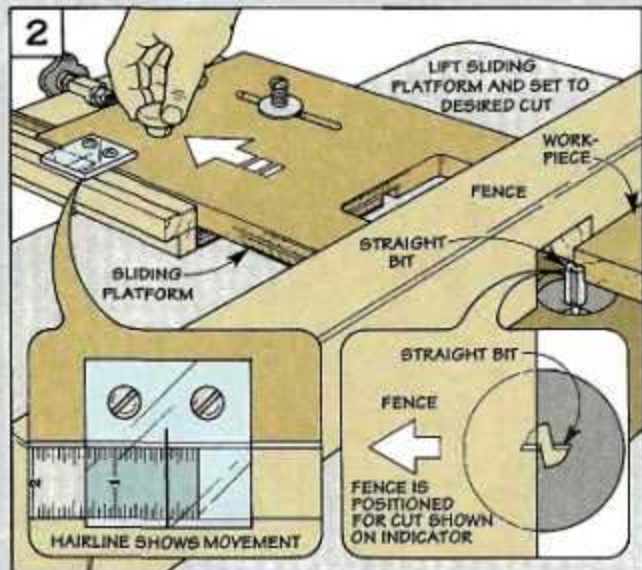
Set the Fence: After setting the ruler to "zero," lift the platform and slide the fence into position. The indicator shows exactly how much you've moved the fence.
