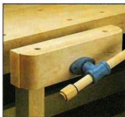
C. Optional Vise: A sturdy vise combines with a simple round dog system to make clamping a workpiece easy.
