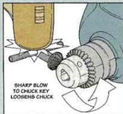
▲ The next step is to insert the chuck key. Rap it sharply with a hammer to loosen chuck. Then remove by hand.
